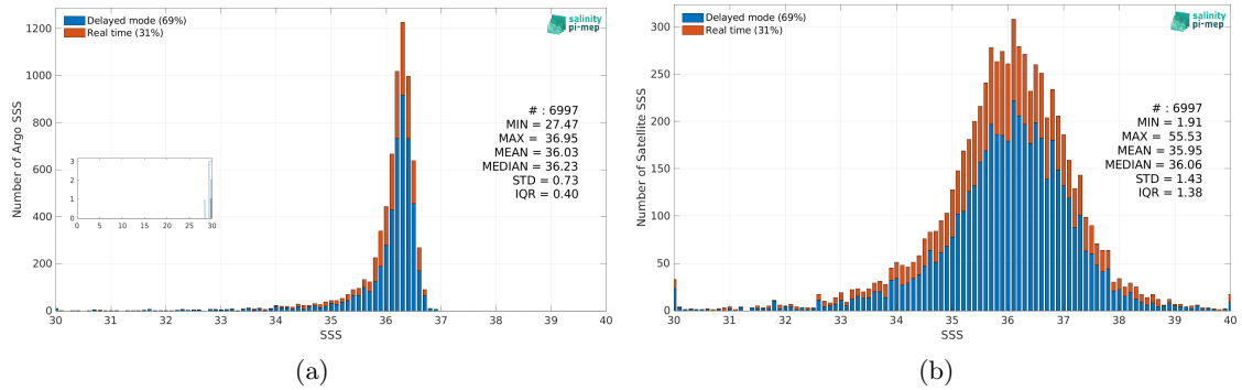
Figure 2: Histograms of SSS from Argo (a) and SMOS SSS L2Q v331 - No FLAG (CMEMS-CATDS-CPDC) (b) considering all match-up pairs per bins of 0.1 over the Gulf of Mexico Pi-MEP region and for the full satellite product period.
