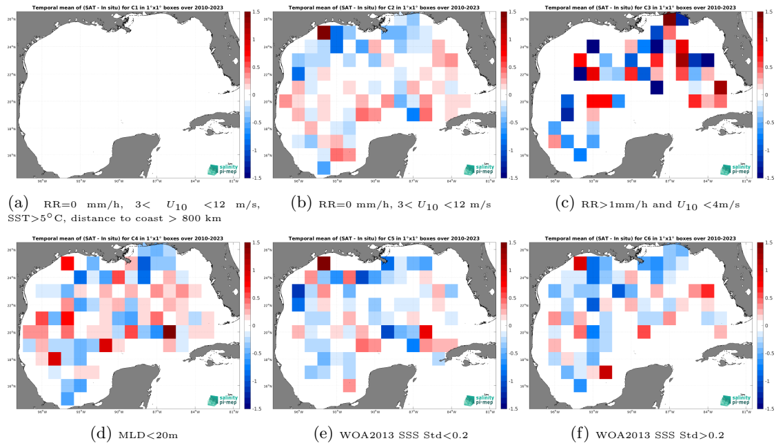
Figure 12: Temporal mean gridded over spatial boxes of size 1^\circ \times 1^\circ of \Delta SSS (SMOS SSS L2Q v331 - No FLAG (CMEMS-CATDS-CPDC) - Argo) for 6 different subdatasets corresponding to:RR=0 mm/h, 3 < U_{10} < 12 m/s, SST > 5^\circ\text{C} , distance to coast > 800 km (a), RR=0 mm/h, 3 < U_{10} < 12 m/s (b), RR > 1 mm/h and U_{10} < 4 m/s (c),MLD < 20 m (d),WOA2013 SSS Std < 0.2 (e),WOA2013 SSS Std > 0.2 (f).
