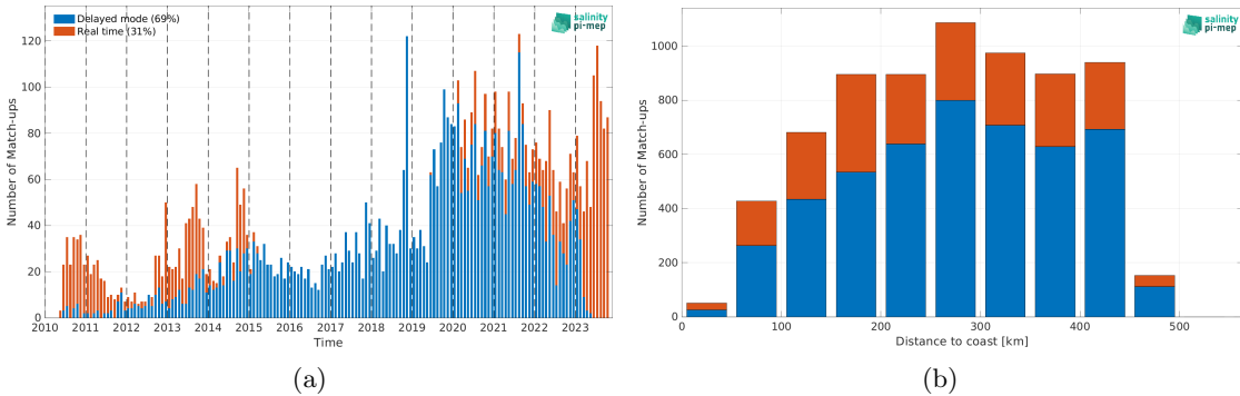
Figure 1: Number of match-ups between Argo and SMOS SSS L2Q v331 - No FLAG (CMEMS-CATDS-CPDC) SSS as a function of time (a) and as function of the distance to coast (b) over the Gulf of Mexico Pi-MEP region and for the full satellite product period.
