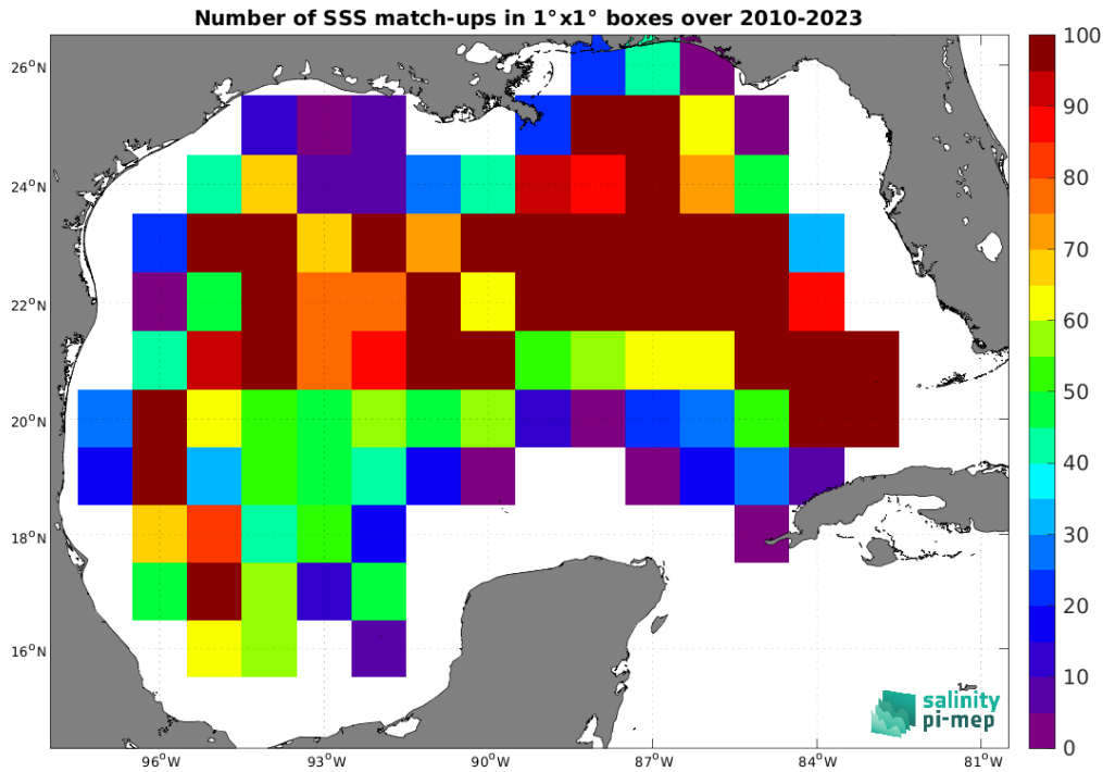
Figure 4: Number of SSS match-ups between Argo SSS and the SMOS SSS L2Q v331 - No FLAG (CMEMS-CATDS-CPDC) SSS product for the Gulf of Mexico Pi-MEP region over 1^\circ \times 1^\circ boxes and for the full satellite product period.
