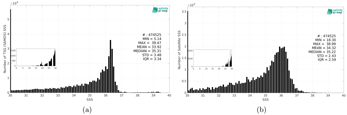
Figure 3: Histograms of SSS from TSG (SAMOS) (a) and SMOS SSS L3 v9 - 9 Days (CATDS-CEC-LOCEAN) (b) considering all match-up pairs per bins of 0.1 over the Gulf of Mexico Pi-MEP region and for the full satellite product period.
