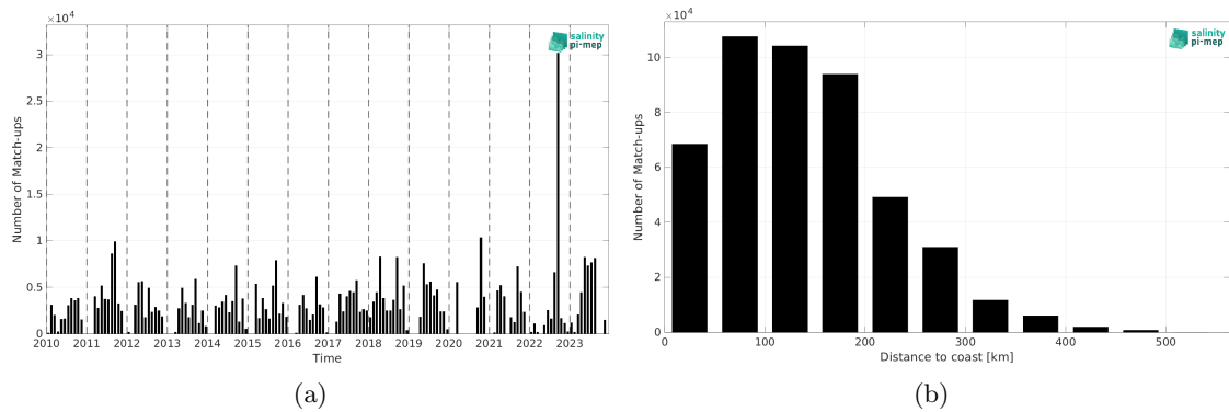
Figure 2: Number of match-ups between TSG (SAMOS) and SMOS SSS L3 v9 - 9 Days (CATDS-CEC-LOCEAN) SSS as a function of time (a) and as function of the distance to coast (b) over the Gulf of Mexico Pi-MEP region and for the full satellite product period.
