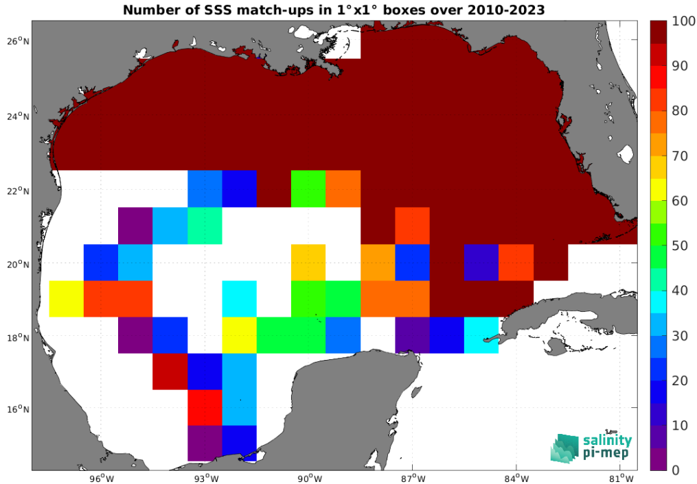
Figure 5: Number of SSS match-ups between TSG (SAMOS) SSS and the SMOS SSS L3 v9 - 9 Days (CATDS-CEC-LOCEAN) SSS product for the Gulf of Mexico Pi-MEP region over 1^\circ \times 1^\circ boxes and for the full satellite product period.
