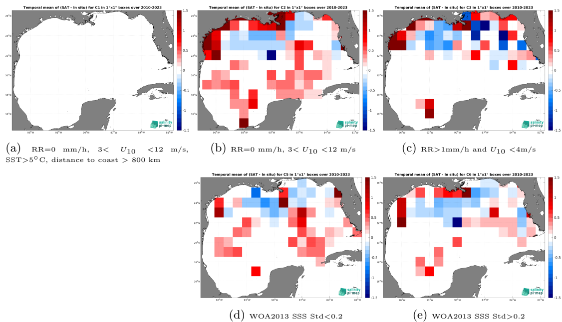
Figure 14: Temporal mean gridded over spatial boxes of size 1^\circ \times 1^\circ of \Delta SSS (SMOS SSS L3 v9 - 9 Days (CATDS-CEC-LOCEAN) - TSG (SAMOS)) for 5 different subdatasets corresponding to:RR=0 mm/h, 3 < U_{10} < 12 m/s, SST >5^\circ C, distance to coast > 800 km (a), RR=0 mm/h, 3 < U_{10} < 12 m/s (b), RR >1 mm/h and U_{10} < 4 m/s (c), WOA2013 SSS Std <0.2 (d), WOA2013 SSS Std >0.2 (e).
