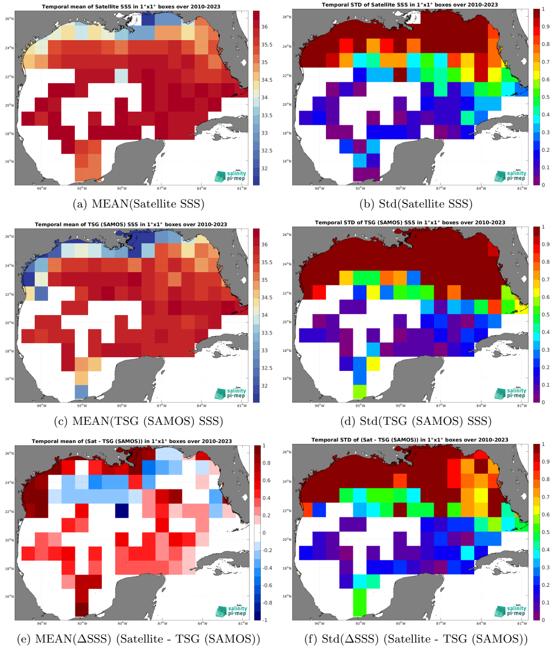
Figure 7: Temporal mean (left) and Std (right) of SSS from SMOS SSS L3 v9 - 9 Days (CATDS-CEC-LOCEAN) (top), TSG (SAMOS) (middle), and of \Delta SSS (Satellite - TSG (SAMOS)). Only match-up pairs are used to generate these maps.
