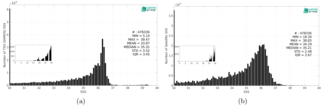
Figure 2: Histograms of SSS from TSG (SAMOS) (a) and SMOS SSS L3 v9 - 9 Days (CATDS-CEC-LOCEAN) (b) considering all match-up pairs per bins of 0.1 over the Gulf of Mexico Pi-MEP region and for the full satellite product period.
