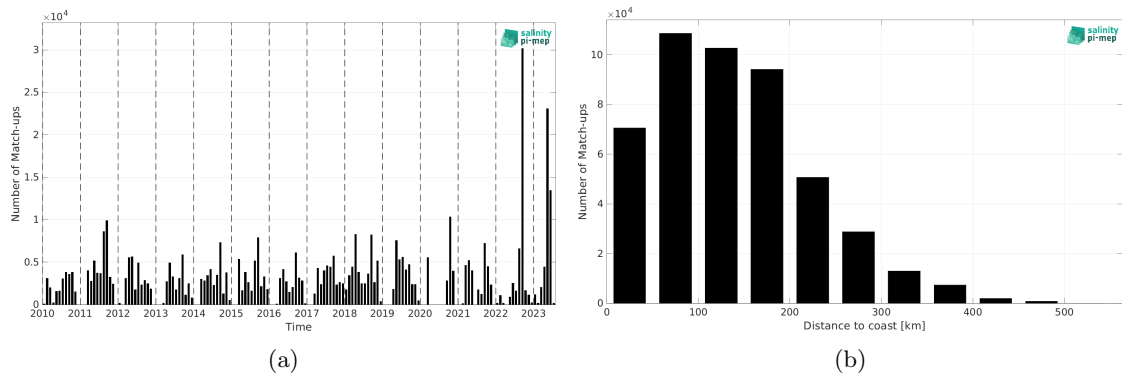
Figure 1: Number of match-ups between TSG (SAMOS) and SMOS SSS L3 v9 - 9 Days (CATDS-CEC-LOCEAN) SSS as a function of time (a) and as function of the distance to coast (b) over the Gulf of Mexico Pi-MEP region and for the full satellite product period.
