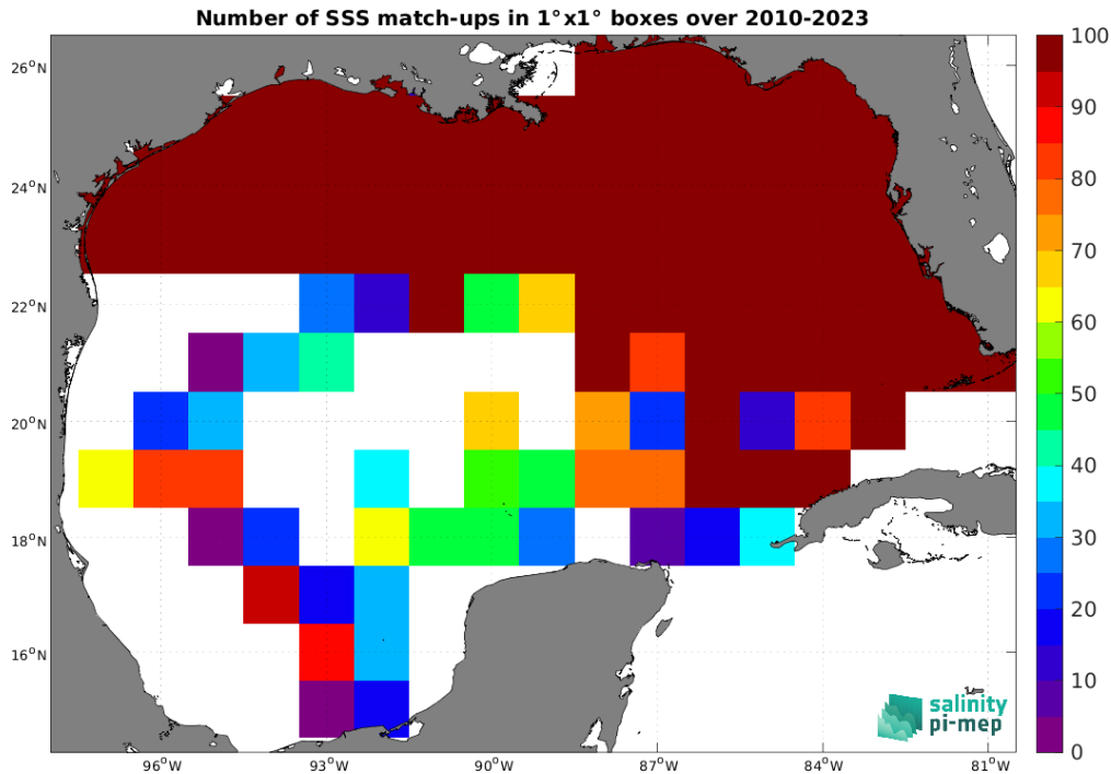
Figure 4: Number of SSS match-ups between TSG (SAMOS) SSS and the SMOS SSS L3 v9 - 9 Days (CATDS-CEC-LOCEAN) SSS product for the Gulf of Mexico Pi-MEP region over 1^\circ \times 1^\circ boxes and for the full satellite product period.
