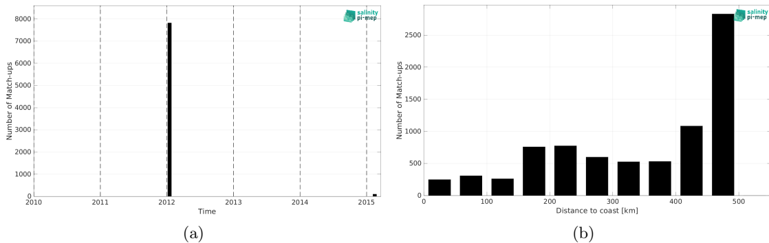
Figure 2: Number of match-ups between TSG (GOSUD-Sailing-ship) and SMOS SSS L3 v9 - 9 Days (CATDS-CEC-LOCEAN) SSS as a function of time (a) and as function of the distance to coast (b) over the Gulf of Mexico Pi-MEP region and for the full satellite product period.
