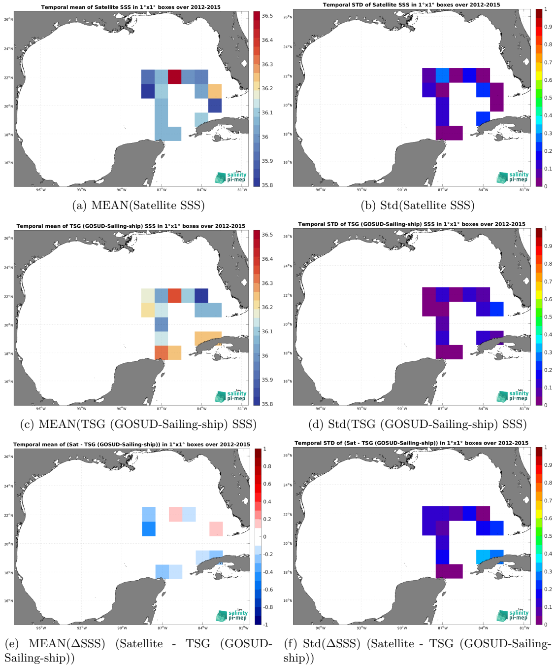
Figure 7: Temporal mean (left) and Std (right) of SSS from SMOS SSS L3 v9 - 9 Days (CATDS-CEC-LOCEAN) (top), TSG (GOSUD-Sailing-ship) (middle), and of \Delta SSS (Satellite - TSG (GOSUD-Sailing-ship)). Only match-up pairs are used to generate these maps.
