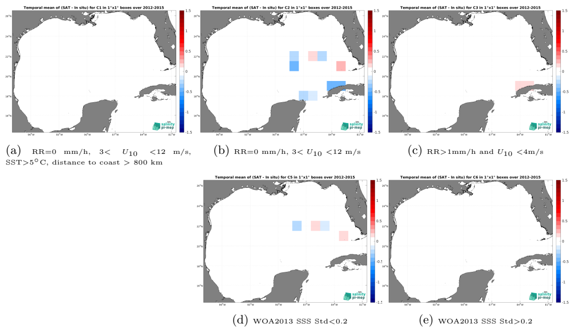
Figure 14: Temporal mean gridded over spatial boxes of size 1^\circ \times 1^\circ of \Delta SSS (SMOS SSS L3 v9 - 9 Days (CATDS-CEC-LOCEAN) - TSG (GOSUD-Sailing-ship)) for 5 different subdatasets corresponding to:RR=0 mm/h, 3 < U_{10} < 12 m/s, SST >5^\circ\text{C} , distance to coast > 800 km (a), RR=0 mm/h, 3 < U_{10} < 12 m/s (b), RR >1 mm/h and U_{10} < 4 m/s (c), WOA2013 SSS Std <0.2 (d), WOA2013 SSS Std >0.2 (e).
