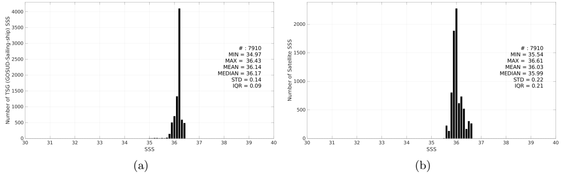
Figure 2: Histograms of SSS from TSG (GOSUD-Sailing-ship) (a) and SMOS SSS L3 v9 - 9 Days (CATDS-CEC-LOCEAN) (b) considering all match-up pairs per bins of 0.1 over the Gulf of Mexico Pi-MEP region and for the full satellite product period.
