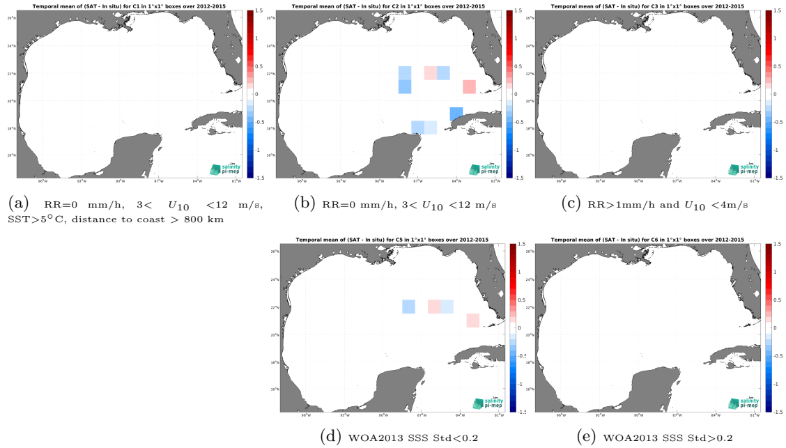
Figure 12: Temporal mean gridded over spatial boxes of size 1^\circ \times 1^\circ of \Delta SSS (SMOS SSS L3 v9 - 9 Days (CATDS-CEC-LOCEAN) - TSG (GOSUD-Sailing-ship)) for 5 different subdatasets corresponding to:RR=0 mm/h, 3 < U_{10} < 12 m/s, SST >5^\circ\text{C} , distance to coast > 800 km (a), RR=0 mm/h, 3 < U_{10} < 12 m/s (b), RR >1 mm/h and U_{10} < 4 m/s (c), WOA2013 SSS Std <0.2 (d), WOA2013 SSS Std >0.2 (e).
