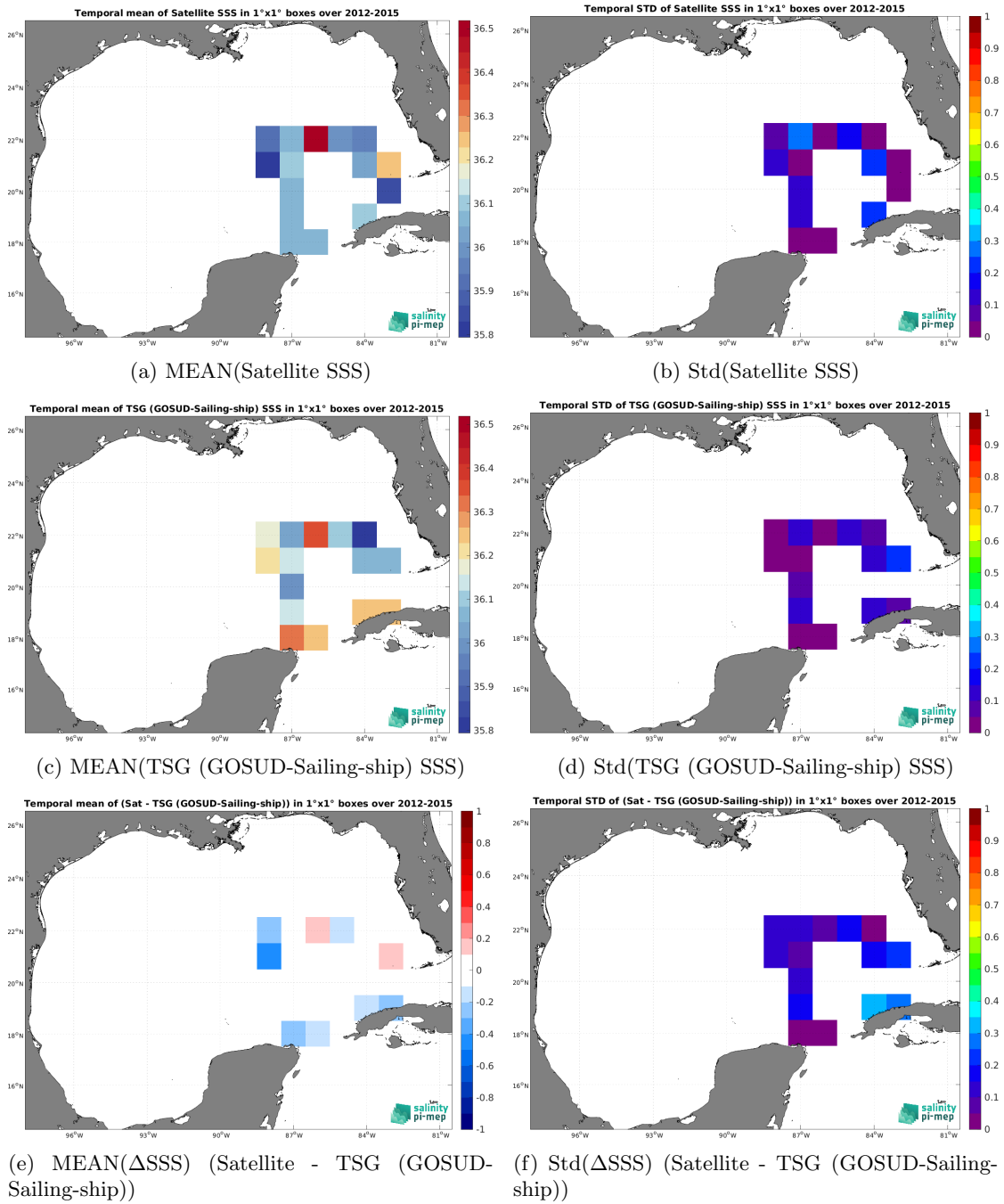
Figure 6: Temporal mean (left) and Std (right) of SSS from SMOS SSS L3 v9 - 9 Days (CATDS-CEC-LOCEAN) (top), TSG (GOSUD-Sailing-ship) (middle), and of \Delta SSS (Satellite - TSG (GOSUD-Sailing-ship)). Only match-up pairs are used to generate these maps.
