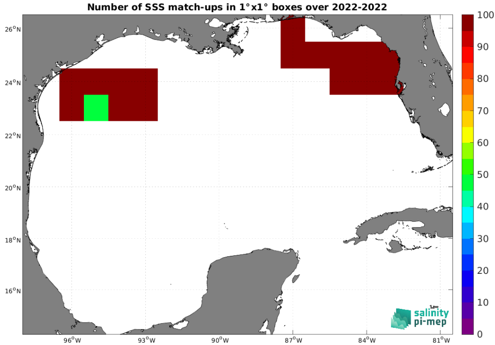
Figure 5: Number of SSS match-ups between Saildrone SSS and the SMOS SSS L3 v9 - 9 Days (CATDS-CEC-LOCEAN) SSS product for the Gulf of Mexico Pi-MEP region over 1^\circ \times 1^\circ boxes and for the full satellite product period.
