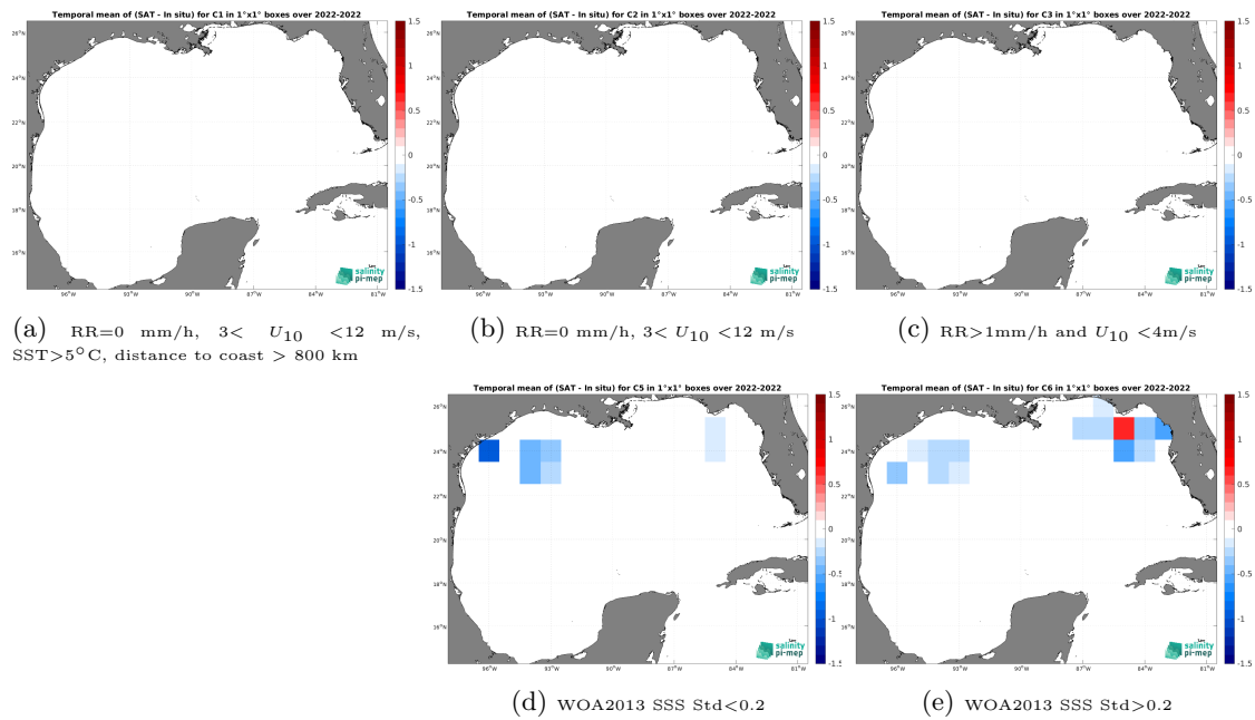
Figure 14: Temporal mean gridded over spatial boxes of size 1^\circ \times 1^\circ of \Delta SSS (SMOS SSS L3 v9 - 9 Days (CATDS-CEC-LOCEAN) - Saildrone) for 5 different subdatasets corresponding to:RR=0 mm/h, 3 < U_{10} < 12 m/s, SST > 5^\circ\text{C} , distance to coast > 800 km (a), RR=0 mm/h, 3 < U_{10} < 12 m/s (b), RR > 1 mm/h and U_{10} < 4 m/s (c), WOA2013 SSS Std < 0.2 (d), WOA2013 SSS Std > 0.2 (e).
