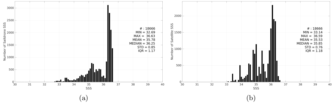
Figure 3: Histograms of SSS from Sairdrone (a) and SMOS SSS L3 v9 - 9 Days (CATDS-CEC-LOCEAN) (b) considering all match-up pairs per bins of 0.1 over the Gulf of Mexico Pi-MEP region and for the full satellite product period.
