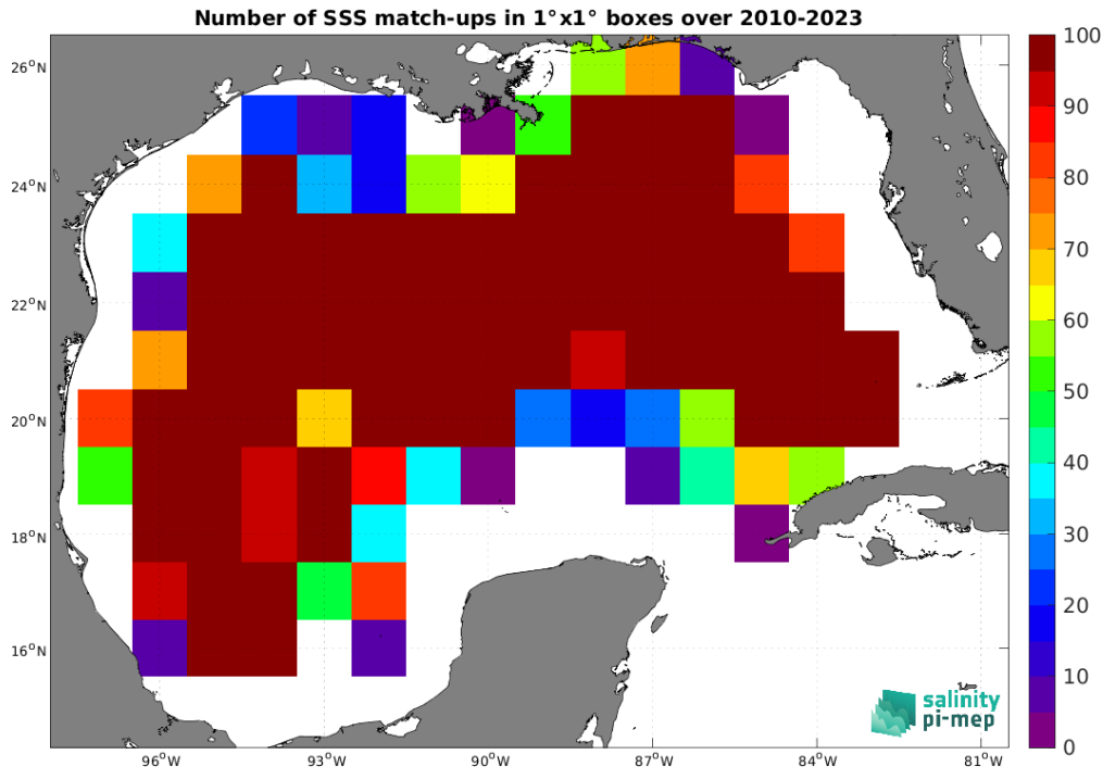
Figure 4: Number of SSS match-ups between Argo SSS and the SMOS SSS L3 v9 - 9 Days (CATDS-CEC-LOCEAN) SSS product for the Gulf of Mexico Pi-MEP region over 1^\circ \times 1^\circ boxes and for the full satellite product period.
