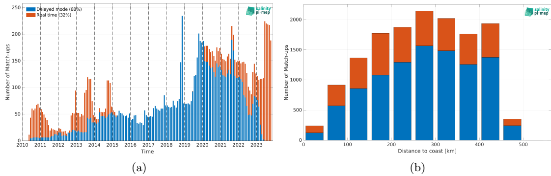
Figure 1: Number of match-ups between Argo and SMOS SSS L3 v9 - 9 Days (CATDS-CEC-LOCEAN) SSS as a function of time (a) and as function of the distance to coast (b) over the Gulf of Mexico Pi-MEP region and for the full satellite product period.
