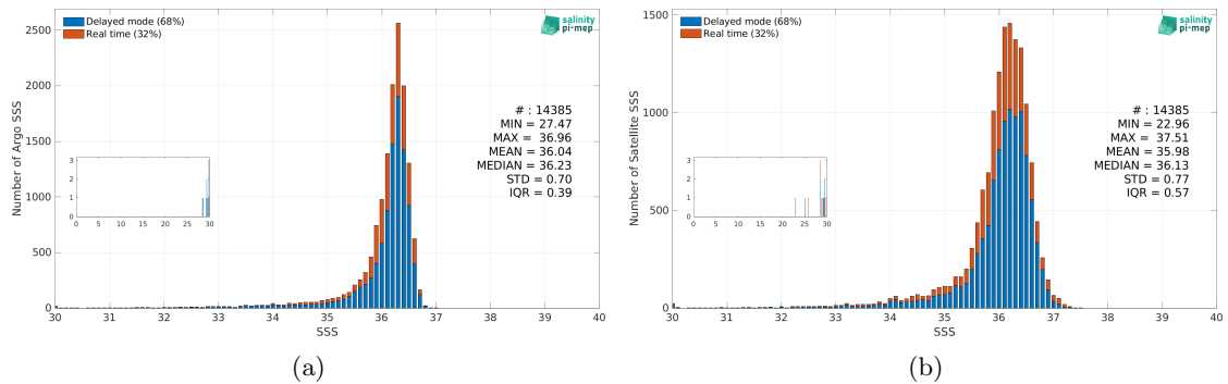
Figure 2: Histograms of SSS from Argo (a) and SMOS SSS L3 v9 - 9 Days (CATDS-CEC-LOCEAN) (b) considering all match-up pairs per bins of 0.1 over the Gulf of Mexico Pi-MEP region and for the full satellite product period.
