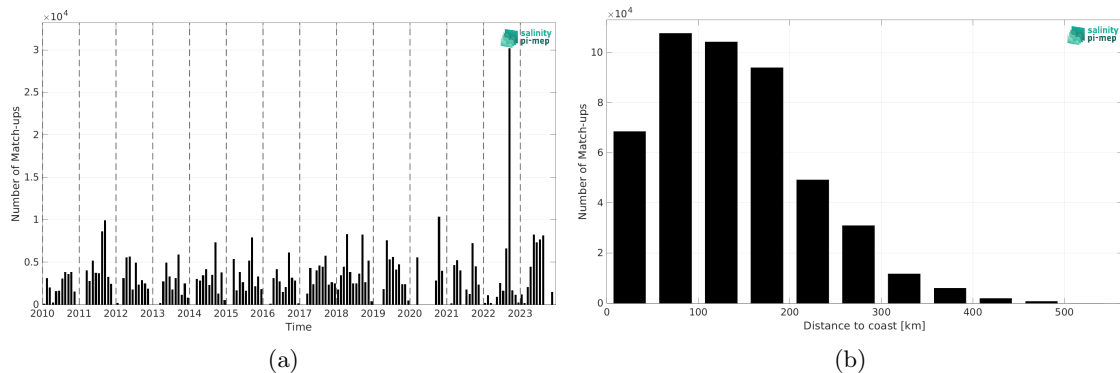
Figure 2: Number of match-ups between TSG (SAMOS) and SMOS SSS L3 v9 - 18 Days (CATDS-CEC-LOCEAN) SSS as a function of time (a) and as function of the distance to coast (b) over the Gulf of Mexico Pi-MEP region and for the full satellite product period.
