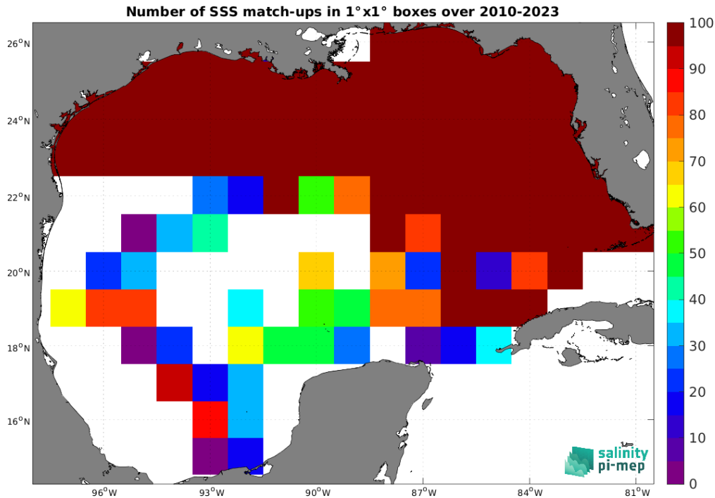
Figure 5: Number of SSS match-ups between TSG (SAMOS) SSS and the SMOS SSS L3 v9 - 18 Days (CATDS-CEC-LOCEAN) SSS product for the Gulf of Mexico Pi-MEP region over 1^\circ \times 1^\circ boxes and for the full satellite product period.
