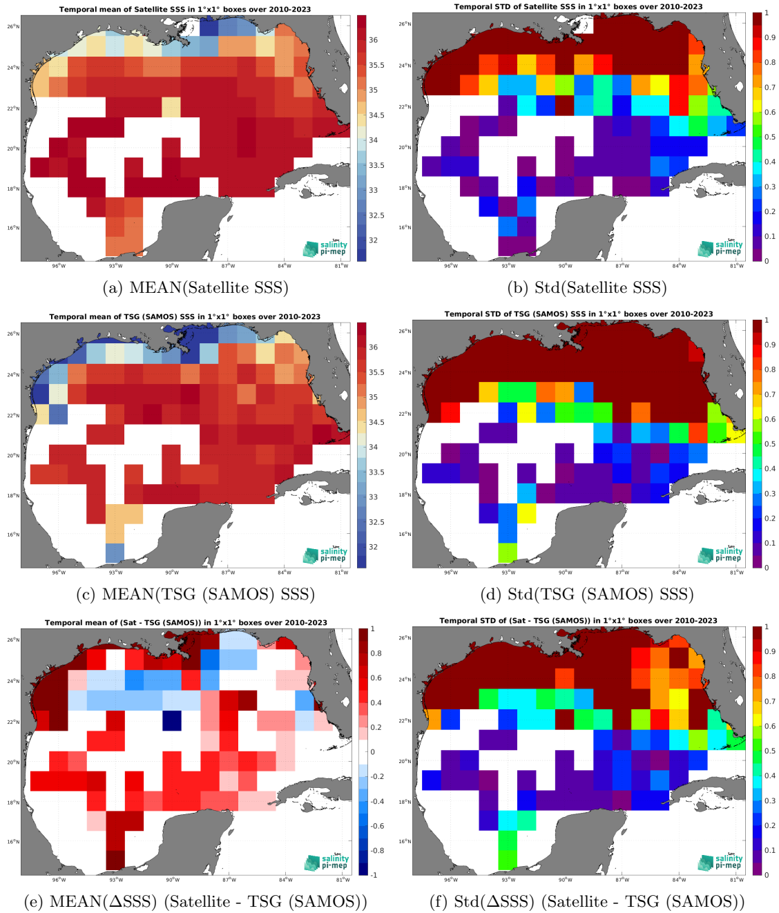
Figure 7: Temporal mean (left) and Std (right) of SSS from SMOS SSS L3 v9 - 18 Days (CATDS-CEC-LOCEAN) (top), TSG (SAMOS) (middle), and of \Delta SSS (Satellite - TSG (SAMOS)). Only match-up pairs are used to generate these maps.
