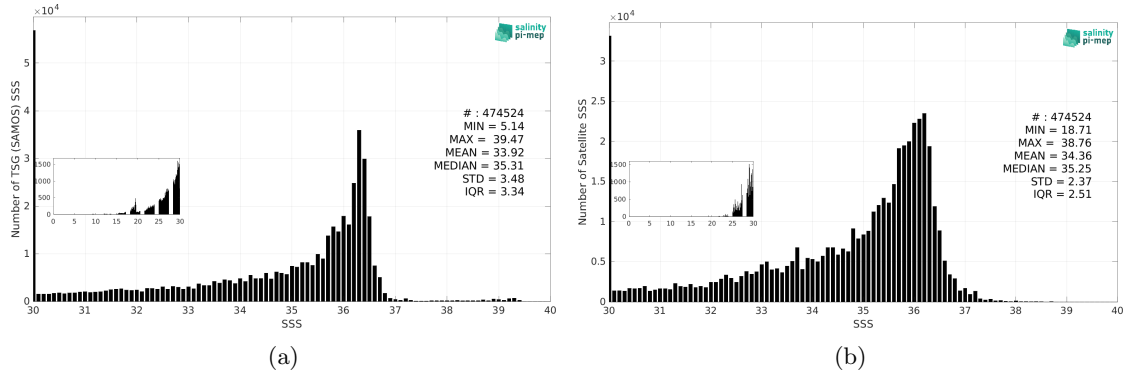
Figure 3: Histograms of SSS from TSG (SAMOS) (a) and SMOS SSS L3 v9 - 18 Days (CATDS-CEC-LOCEAN) (b) considering all match-up pairs per bins of 0.1 over the Gulf of Mexico Pi-MEP region and for the full satellite product period.
