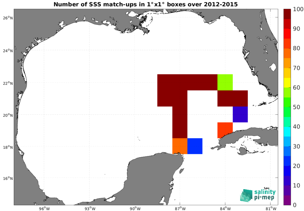
Figure 5: Number of SSS match-ups between TSG (GOSUD-Sailing-ship) SSS and the SMOS SSS L3 v9 - 18 Days (CATDS-CEC-LOCEAN) SSS product for the Gulf of Mexico Pi-MEP region over 1^\circ \times 1^\circ boxes and for the full satellite product period.
