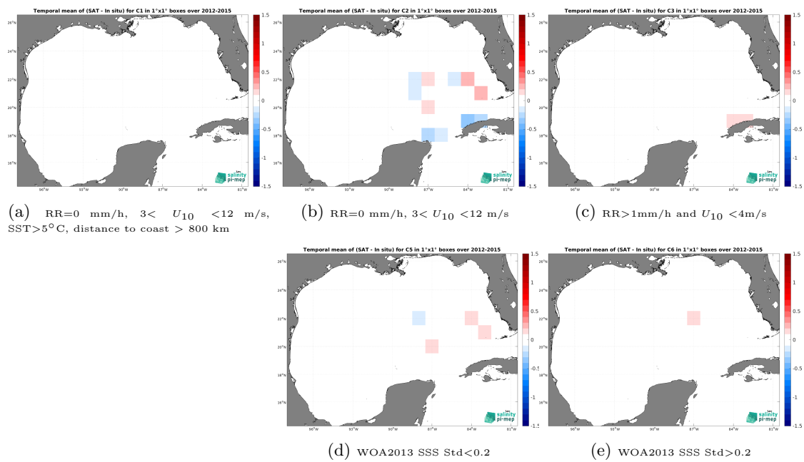
Figure 14: Temporal mean gridded over spatial boxes of size 1^\circ \times 1^\circ of \Delta SSS (SMOS SSS L3 v9 - 18 Days (CATDS-CEC-LOCEAN) - TSG (GOSUD-Sailing-ship)) for 5 different subdatasets corresponding to:RR=0 mm/h, 3 < U_{10} < 12 m/s, SST >5^\circ\text{C} , distance to coast > 800 km (a), RR=0 mm/h, 3 < U_{10} < 12 m/s (b), RR >1 mm/h and U_{10} < 4 m/s (c), WOA2013 SSS Std <0.2 (d), WOA2013 SSS Std >0.2 (e).
