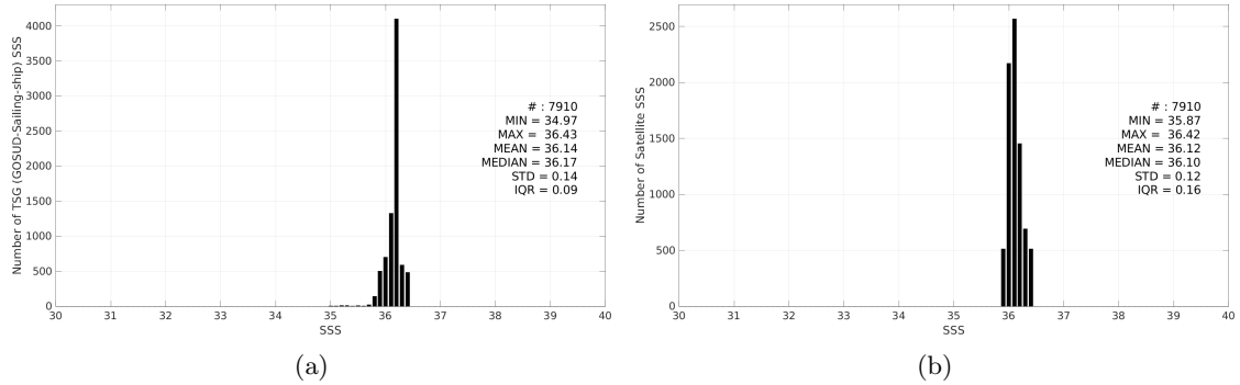
Figure 3: Histograms of SSS from TSG (GOSUD-Sailing-ship) (a) and SMOS SSS L3 v9 - 18 Days (CATDS-CEC-LOCEAN) (b) considering all match-up pairs per bins of 0.1 over the Gulf of Mexico Pi-MEP region and for the full satellite product period.
