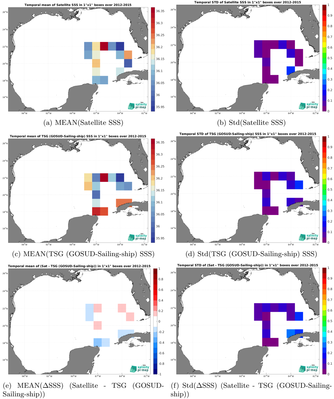
Figure 7: Temporal mean (left) and Std (right) of SSS from SMOS SSS L3 v9 - 18 Days (CATDS-CEC-LOCEAN) (top), TSG (GOSUD-Sailing-ship) (middle), and of \Delta SSS (Satellite - TSG (GOSUD-Sailing-ship)). Only match-up pairs are used to generate these maps.
