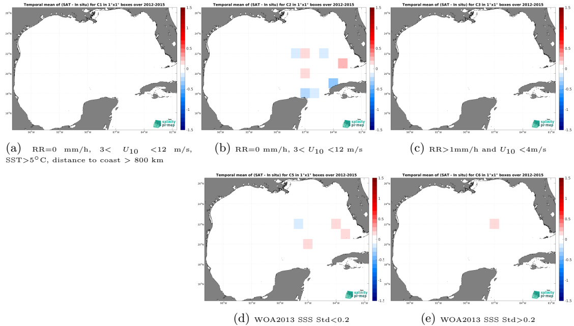
Figure 12: Temporal mean gridded over spatial boxes of size 1^\circ \times 1^\circ of \Delta SSS (SMOS SSS L3 v9 - 18 Days (CATDS-CEC-LOCEAN) - TSG (GOSUD-Sailing-ship)) for 5 different subdatasets corresponding to:RR=0 mm/h, 3 < U_{10} < 12 m/s, SST >5^\circ\text{C} , distance to coast > 800 km (a), RR=0 mm/h, 3 < U_{10} < 12 m/s (b), RR >1 mm/h and U_{10} < 4 m/s (c), WOA2013 SSS Std <0.2 (d), WOA2013 SSS Std >0.2 (e).
