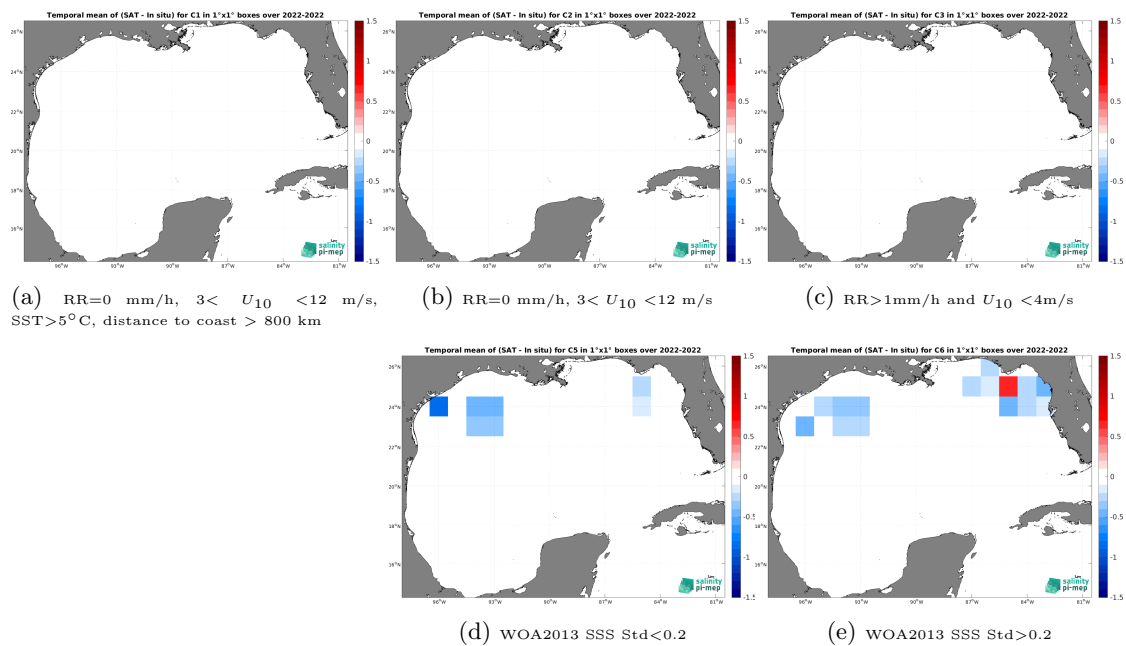
Figure 14: Temporal mean gridded over spatial boxes of size 1^\circ \times 1^\circ of \Delta\text{SSS} (SMOS SSS L3 v9 - 18 Days (CATDS-CEC-LOCEAN) - Saildrone) for 5 different subdatasets corresponding to: RR=0 mm/h, 3 < U_{10} < 12 m/s, SST > 5°C, distance to coast > 800 km (a), RR=0 mm/h, 3 < U_{10} < 12 m/s (b), RR > 1 mm/h and U_{10} < 4 m/s (c), WOA2013 SSS Std < 0.2 (d), WOA2013 SSS Std > 0.2 (e).
