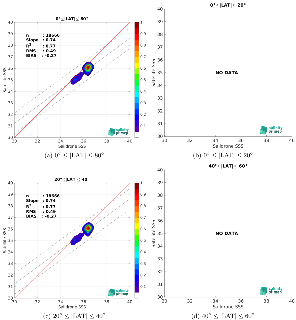
Figure 10: Contour maps of the concentration of SMOS SSS L3 v9 - 18 Days (CATDS-CEC-LOCEAN) SSS (y-axis) versus Sailldrone SSS (x-axis) at match-up pairs for different latitude bands. For each plot, the red line shows x=y . The black thin and dashed lines indicate a linear fit through the data cloud and the \pm 95\% confidence levels, respectively. The number match-up pairs n , the slope and R^2 coefficient of the linear fit, the root mean square (RMS) and the mean bias between satellite and in situ data are indicated for each latitude band in each plots.
