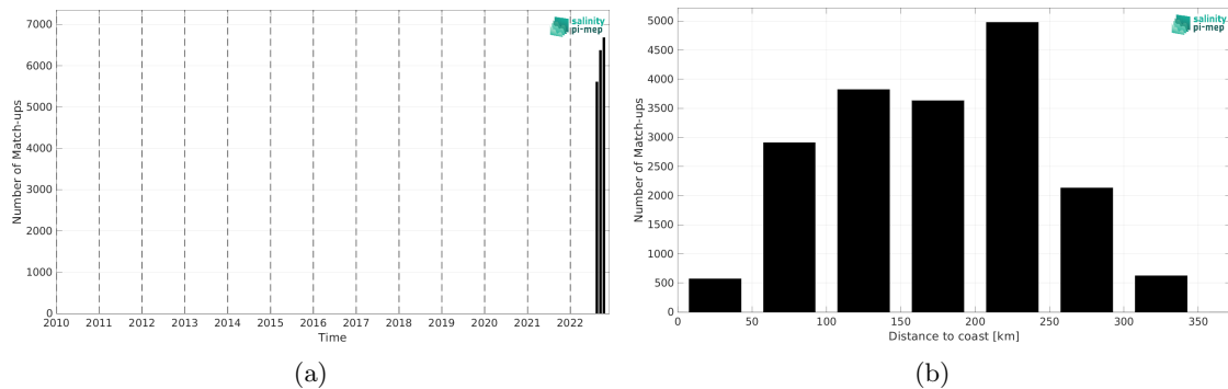
Figure 2: Number of match-ups between Saildrone and SMOS SSS L3 v9 - 18 Days (CATDS-CEC-LOCEAN) SSS as a function of time (a) and as function of the distance to coast (b) over the Gulf of Mexico Pi-MEP region and for the full satellite product period.
