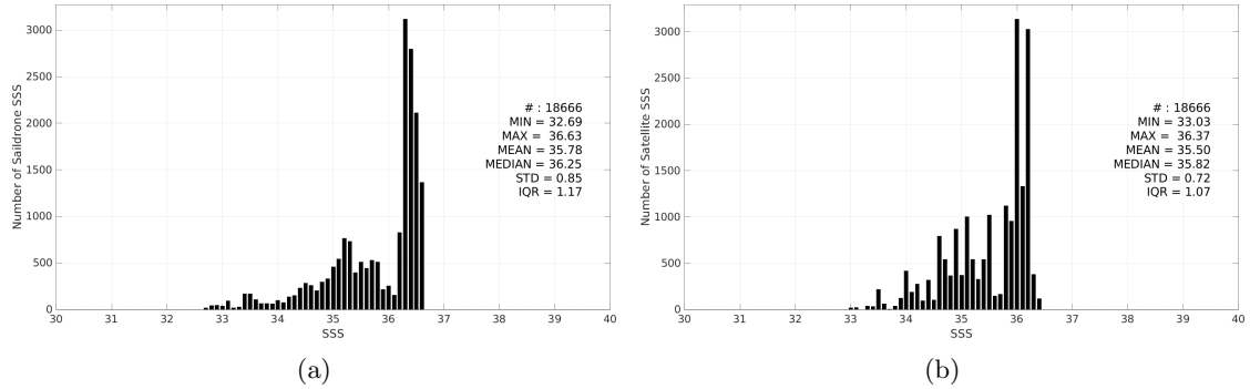
Figure 3: Histograms of SSS from Saildrone (a) and SMOS SSS L3 v9 - 18 Days (CATDS-CEC-LOCEAN) (b) considering all match-up pairs per bins of 0.1 over the Gulf of Mexico Pi-MEP region and for the full satellite product period.
