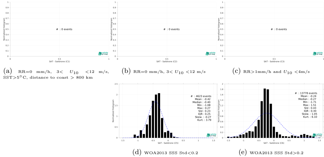
Figure 15: Normalized histogram of \Delta SSS (SMOS SSS L3 v9 - 18 Days (CATDS-CEC-LOCEAN) - Saildrone) for 5 different subdatasets corresponding to: RR=0 mm/h, 3 < U_{10} < 12 m/s, SST >5^{\circ} C, distance to coast > 800 km (a), RR=0 mm/h, 3 < U_{10} < 12 m/s (b), RR >1 mm/h and U_{10} < 4 m/s (c), WOA2013 SSS Std <0.2 (d), WOA2013 SSS Std >0.2 (e).
