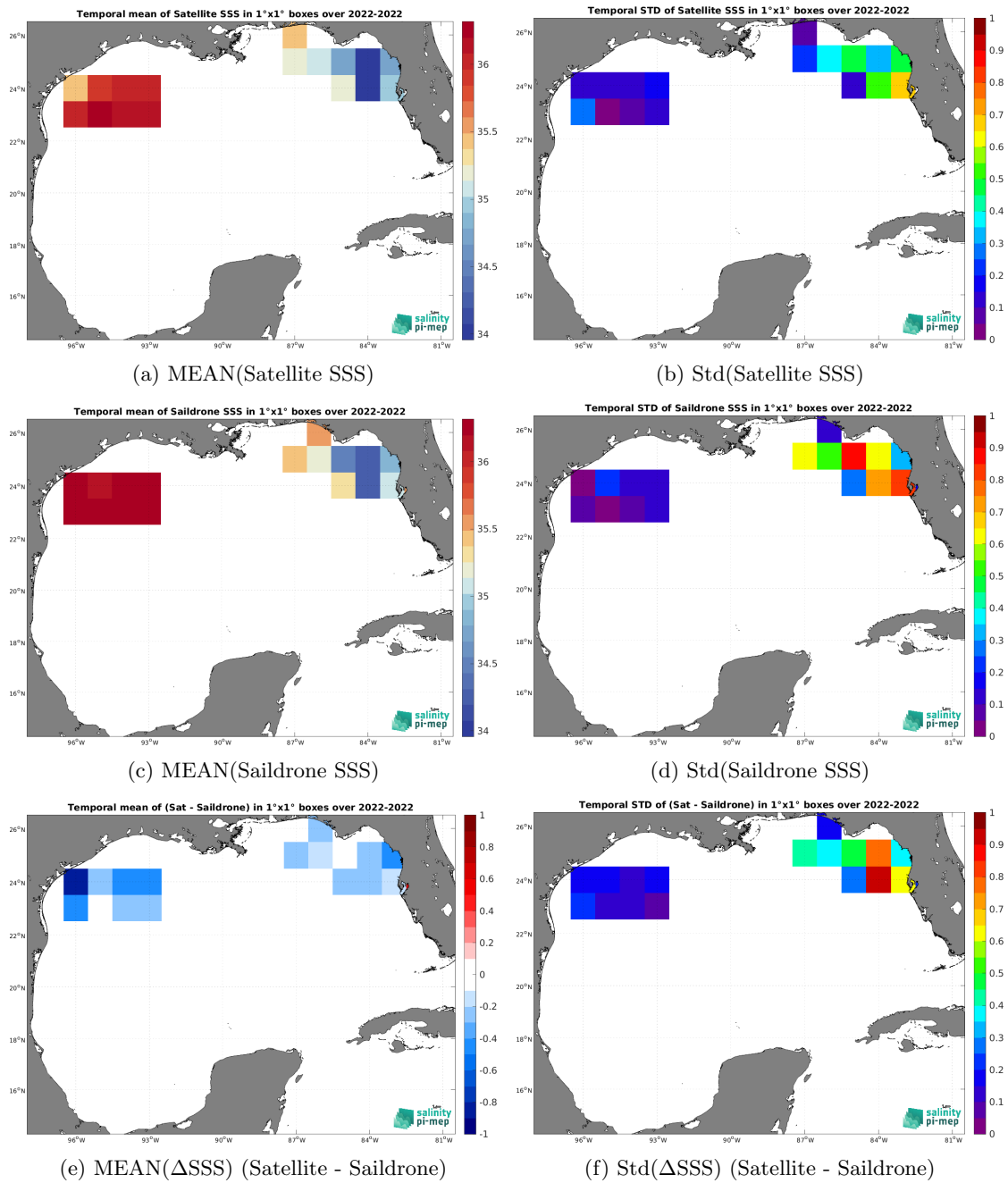
Figure 6: Temporal mean (left) and Std (right) of SSS from SMOS SSS L3 v9 - 18 Days (CATDS-CEC-LOCEAN) (top), Saildrone (middle), and of \Delta SSS (Satellite - Saildrone). Only match-up pairs are used to generate these maps.
