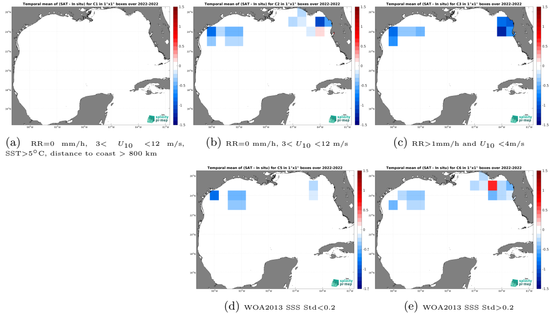
Figure 12: Temporal mean gridded over spatial boxes of size 1^{\circ}\times 1^{\circ} of \Delta\text{SSS} (SMOS SSS L3 v9 - 18 Days (CATDS-CEC-LOCEAN) - Saildrone) for 5 different subdatasets corresponding to:RR=0 mm/h, 3 < U_{10} < 12 m/s, SST >5^{\circ}\text{C} , distance to coast > 800 km (a), RR=0 mm/h, 3 < U_{10} < 12 m/s (b), RR >1 mm/h and U_{10} < 4 m/s (c), WOA2013 SSS Std <0.2 (d), WOA2013 SSS Std >0.2 (e).
