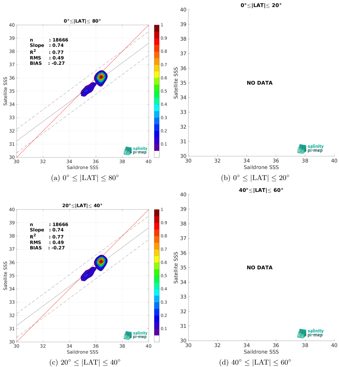
Figure 9: Contour maps of the concentration of SMOS SSS L3 v9 - 18 Days (CATDS-CEC-LOCEAN) SSS (y-axis) versus Sailldrone SSS (x-axis) at match-up pairs for different latitude bands. For each plot, the red line shows x=y . The black thin and dashed lines indicate a linear fit through the data cloud and the \pm 95\% confidence levels, respectively. The number match-up pairs n , the slope and R^2 coefficient of the linear fit, the root mean square (RMS) and the mean bias between satellite and in situ data are indicated for each latitude band in each plots.
