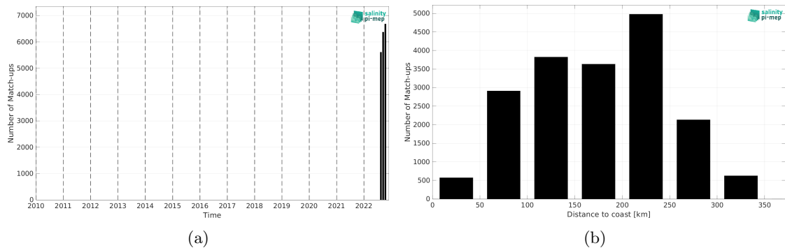
Figure 1: Number of match-ups between Saildrone and SMOS SSS L3 v9 - 18 Days (CATDS-CEC-LOCEAN) SSS as a function of time (a) and as function of the distance to coast (b) over the Gulf of Mexico Pi-MEP region and for the full satellite product period.
