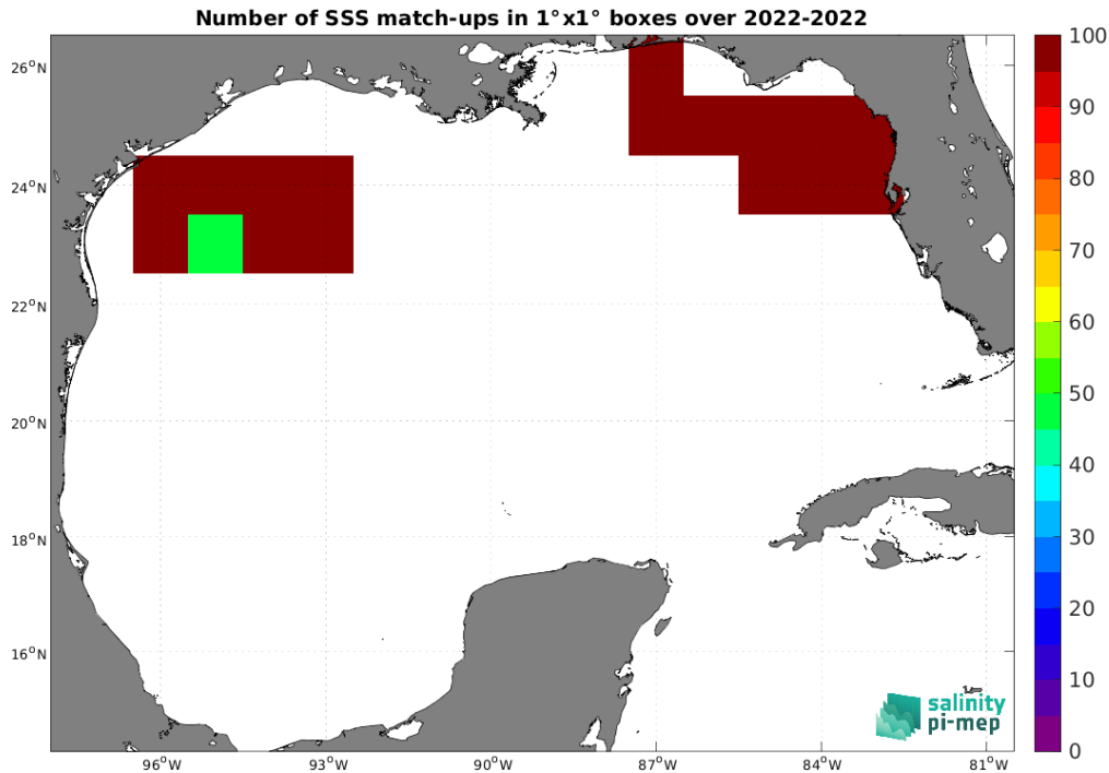
Figure 4: Number of SSS match-ups between Saildrone SSS and the SMOS SSS L3 v9 - 18 Days (CATDS-CEC-LOCEAN) SSS product for the Gulf of Mexico Pi-MEP region over 1^\circ \times 1^\circ boxes and for the full satellite product period.
