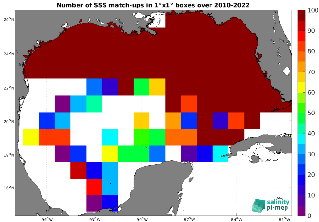
Figure 4: Number of SSS match-ups between TSG (SAMOS) SSS and the SMOS SSS L3 v8 - 9 Days (CATDS-CEC-LOCEAN) SSS product for the Gulf of Mexico Pi-MEP region over 1^\circ \times 1^\circ boxes and for the full satellite product period.
