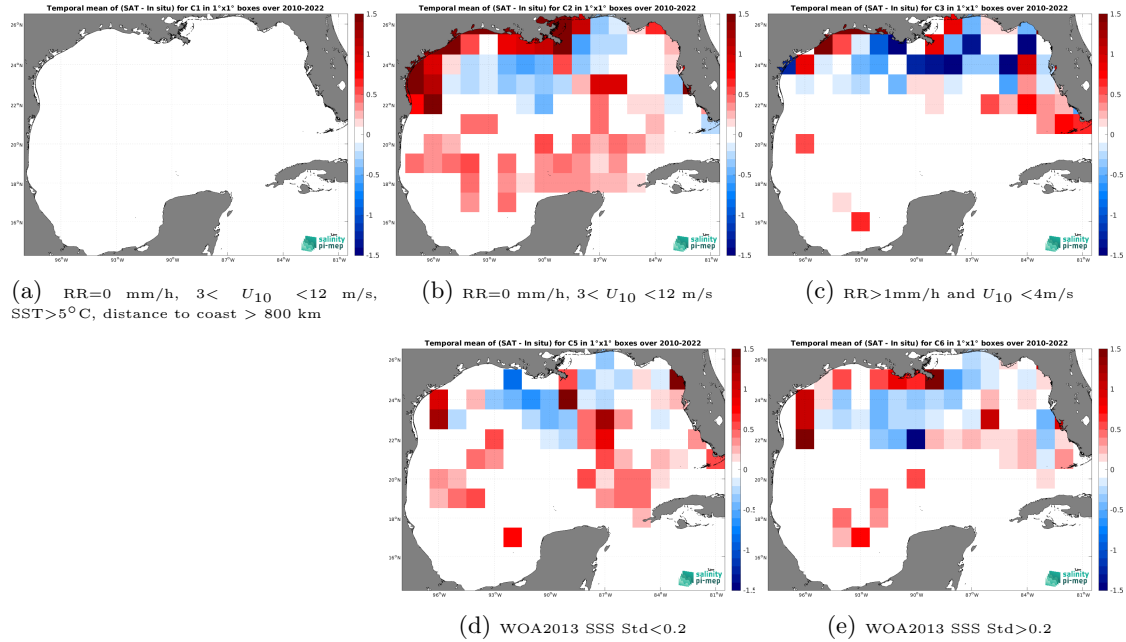
Figure 12: Temporal mean gridded over spatial boxes of size 1^{\circ}\times 1^{\circ} of \Delta\text{SSS} (SMOS SSS L3 v8 - 9 Days (CATDS-CEC-LOCEAN) - TSG (SAMOS)) for 5 different subdatasets corresponding to:RR=0 mm/h, 3 < U_{10} < 12 m/s, SST >5^{\circ}\text{C} , distance to coast > 800 km (a), RR=0 mm/h, 3 < U_{10} < 12 m/s (b), RR >1 mm/h and U_{10} < 4 m/s (c), WOA2013 SSS Std <0.2 (d), WOA2013 SSS Std >0.2 (e).
