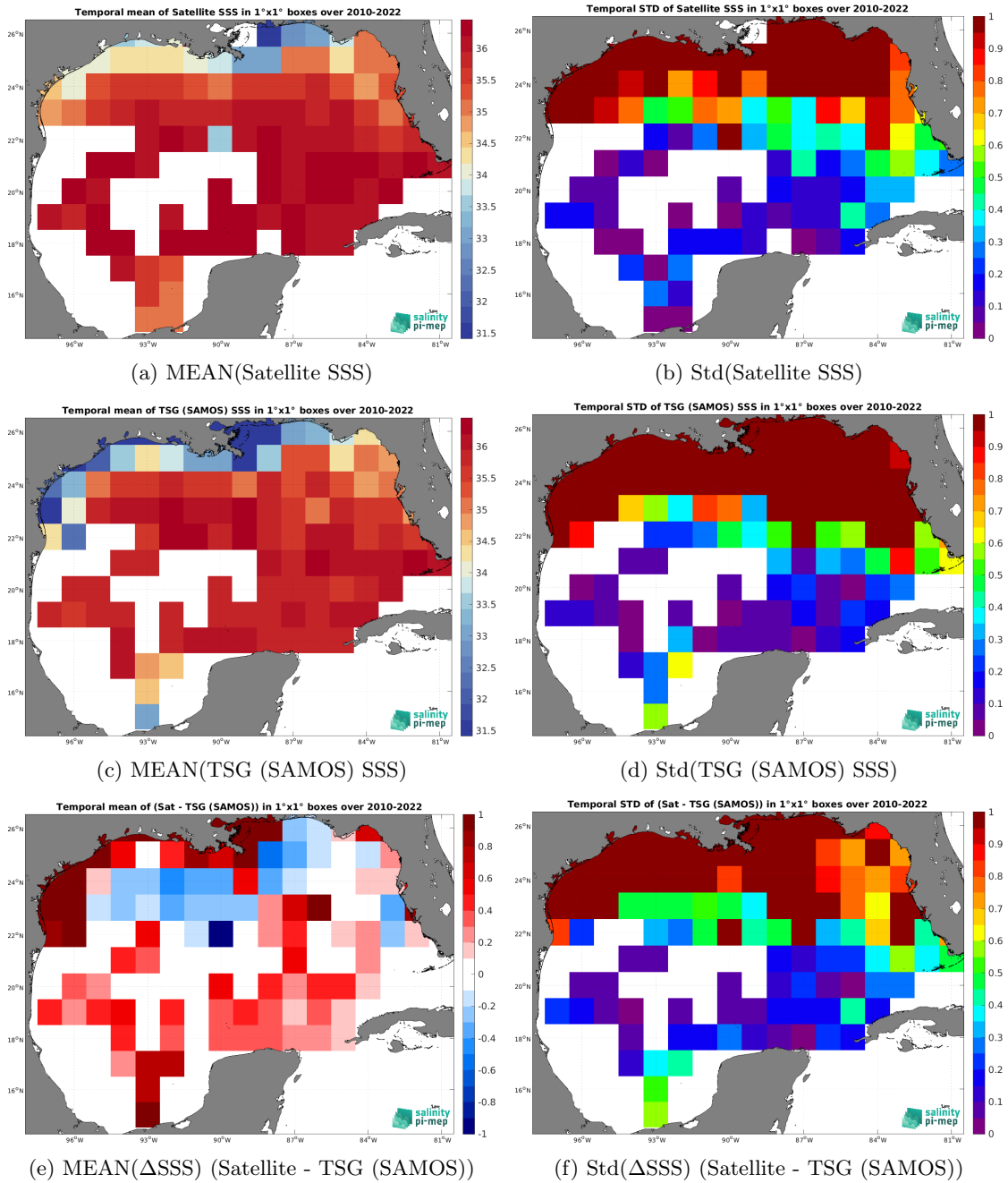
Figure 6: Temporal mean (left) and Std (right) of SSS from SMOS SSS L3 v8 - 9 Days (CATDS-CEC-LOCEAN) (top), TSG (SAMOS) (middle), and of \Delta SSS (Satellite - TSG (SAMOS)). Only match-up pairs are used to generate these maps.
