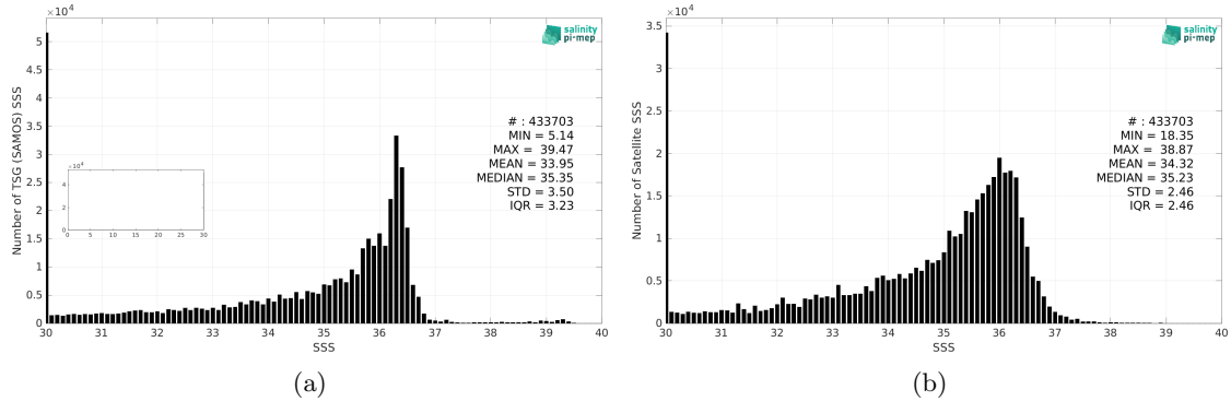
Figure 2: Histograms of SSS from TSG (SAMOS) (a) and SMOS SSS L3 v8 - 9 Days (CATDS-CEC-LOCEAN) (b) considering all match-up pairs per bins of 0.1 over the Gulf of Mexico Pi-MEP region and for the full satellite product period.
