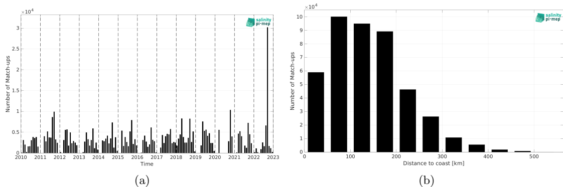
Figure 1: Number of match-ups between TSG (SAMOS) and SMOS SSS L3 v8 - 9 Days (CATDS-CEC-LOCEAN) SSS as a function of time (a) and as function of the distance to coast (b) over the Gulf of Mexico Pi-MEP region and for the full satellite product period.
