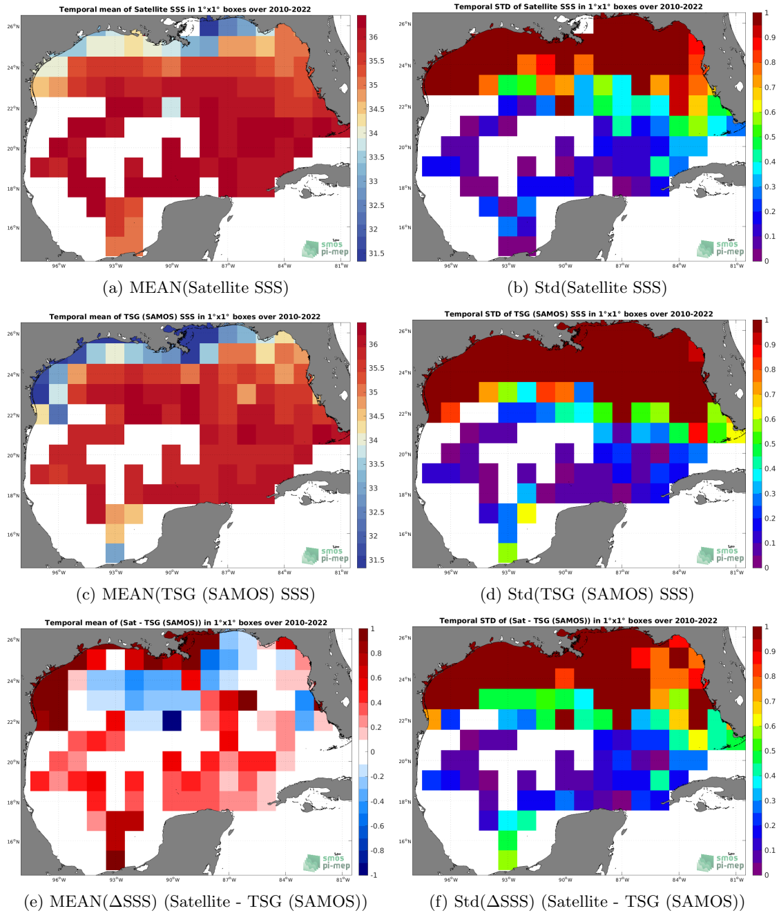
Figure 6: Temporal mean (left) and Std (right) of SSS from SMOS SSS L3 v8 - 9 Days (CATDS-CECOS-LOCEAN) (top), TSG (SAMOS) (middle), and of \Delta SSS (Satellite - TSG (SAMOS)). Only match-up pairs are used to generate these maps.
