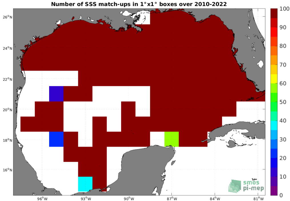
Figure 4: Number of SSS match-ups between TSG (SAMOS) SSS and the SMOS SSS L3 v8 - 9 Days (CATDS-CECOS-LOCEAN) SSS product for the Gulf of Mexico Pi-MEP region over 1^\circ \times 1^\circ boxes and for the full satellite product period.
