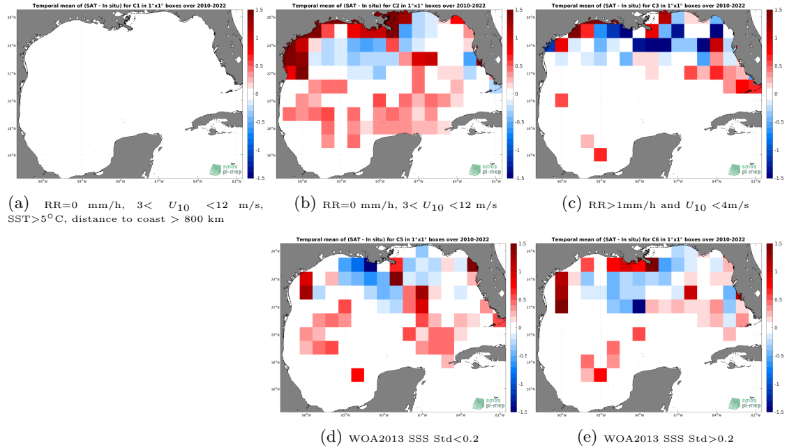
Figure 12: Temporal mean gridded over spatial boxes of size 1^{\circ}\times 1^{\circ} of \Delta\text{SSS} (SMOS SSS L3 v8 - 9 Days (CATDS-CECOS-LOCEAN) - TSG (SAMOS)) for 5 different subdatasets corresponding to:RR=0 mm/h, 3 < U_{10} < 12 m/s, SST >5^{\circ}\text{C} , distance to coast > 800 km (a), RR=0 mm/h, 3 < U_{10} < 12 m/s (b), RR >1 mm/h and U_{10} < 4 m/s (c), WOA2013 SSS Std <0.2 (d), WOA2013 SSS Std >0.2 (e).
