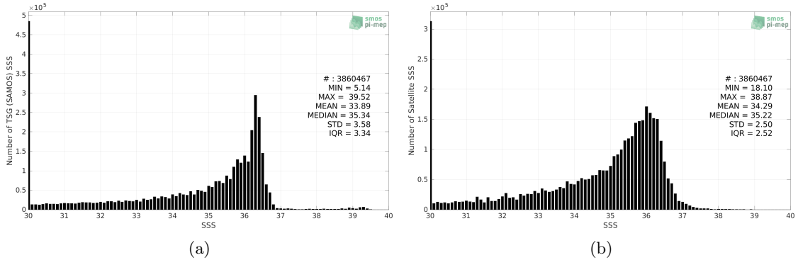
Figure 2: Histograms of SSS from TSG (SAMOS) (a) and SMOS SSS L3 v8 - 9 Days (CATDS-CECOS-LOCEAN) (b) considering all match-up pairs per bins of 0.1 over the Gulf of Mexico Pi-MEP region and for the full satellite product period.
