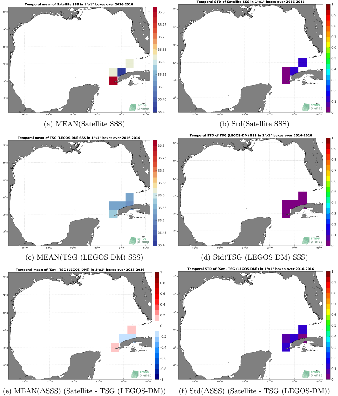
Figure 6: Temporal mean (left) and Std (right) of SSS from SMOS SSS L3 v8 - 9 Days (CATDS-CECOS-LOCEAN) (top), TSG (LEGOS-DM) (middle), and of \Delta SSS (Satellite - TSG (LEGOS-DM)). Only match-up pairs are used to generate these maps.
