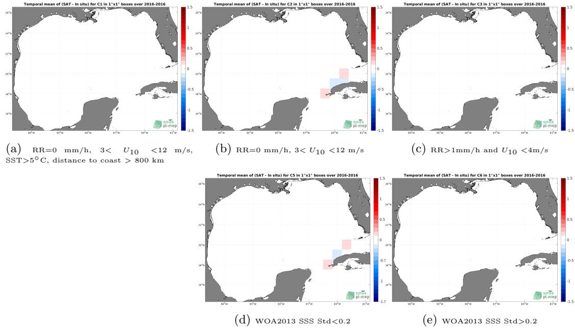
Figure 12: Temporal mean gridded over spatial boxes of size 1^{\circ}\times 1^{\circ} of \Delta\text{SSS} (SMOS SSS L3 v8 - 9 Days (CATDS-CECOS-LOCEAN) - TSG (LEGOS-DM)) for 5 different subdatasets corresponding to:RR=0 mm/h, 3 < U_{10} < 12 m/s, SST >5^{\circ}\text{C} , distance to coast > 800 km (a), RR=0 mm/h, 3 < U_{10} < 12 m/s (b), RR >1 mm/h and U_{10} < 4 m/s (c), WOA2013 SSS Std <0.2 (d), WOA2013 SSS Std >0.2 (e).
