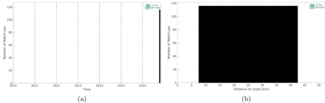
Figure 1: Number of match-ups between TSG (LEGOS-DM) and SMOS SSS L3 v8 - 9 Days (CATDS-CECOS-LOCEAN) SSS as a function of time (a) and as function of the distance to coast (b) over the Gulf of Mexico Pi-MEP region and for the full satellite product period.
