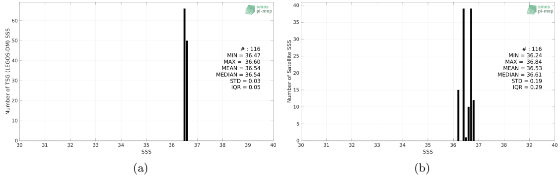
Figure 2: Histograms of SSS from TSG (LEGOS-DM) (a) and SMOS SSS L3 v8 - 9 Days (CATDS-CECOS-LOCEAN) (b) considering all match-up pairs per bins of 0.1 over the Gulf of Mexico Pi-MEP region and for the full satellite product period.
