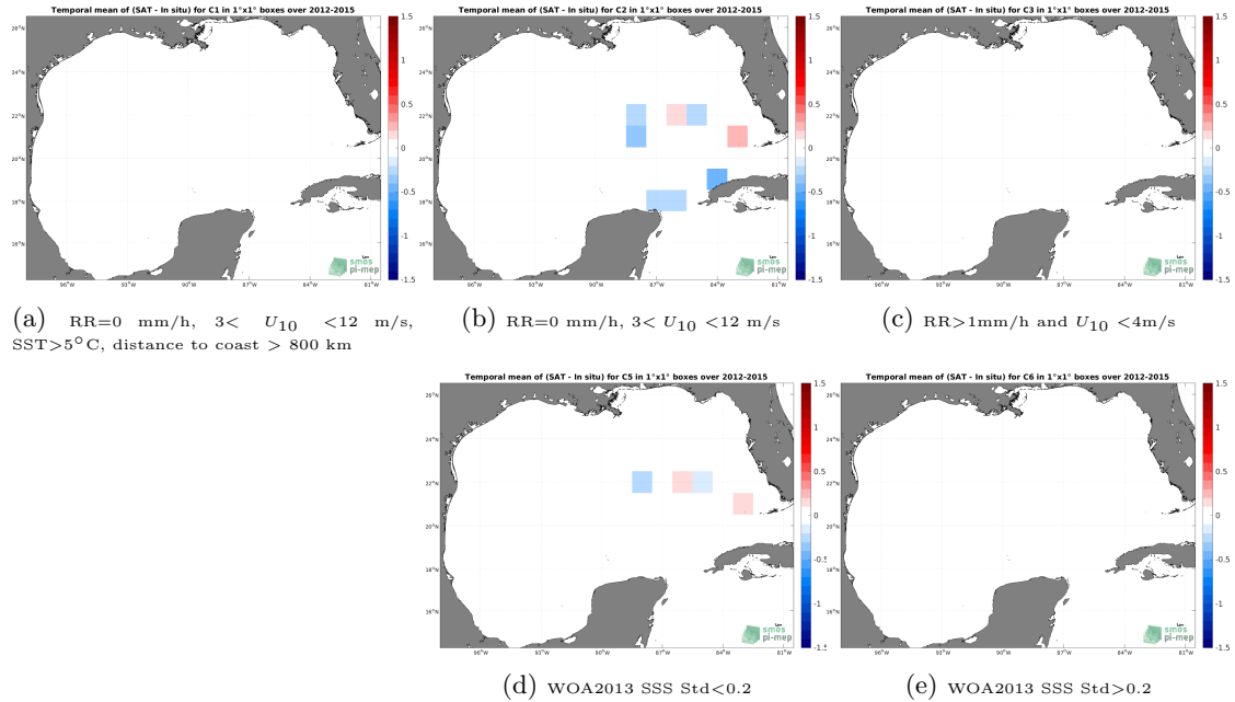
Figure 12: Temporal mean gridded over spatial boxes of size 1^{\circ}\times 1^{\circ} of \Delta SSS (SMOS SSS L3 v8 - 9 Days (CATDS-CECOS-LOCEAN) - TSG (GOSUD-Sailing-ship)) for 5 different subdatasets corresponding to:RR=0 mm/h, 3 < U_{10} < 12 m/s, SST >5^{\circ}\text{C} , distance to coast > 800 km (a), RR=0 mm/h, 3 < U_{10} < 12 m/s (b), RR >1 mm/h and U_{10} < 4 m/s (c), WOA2013 SSS Std <0.2 (d), WOA2013 SSS Std >0.2 (e).
