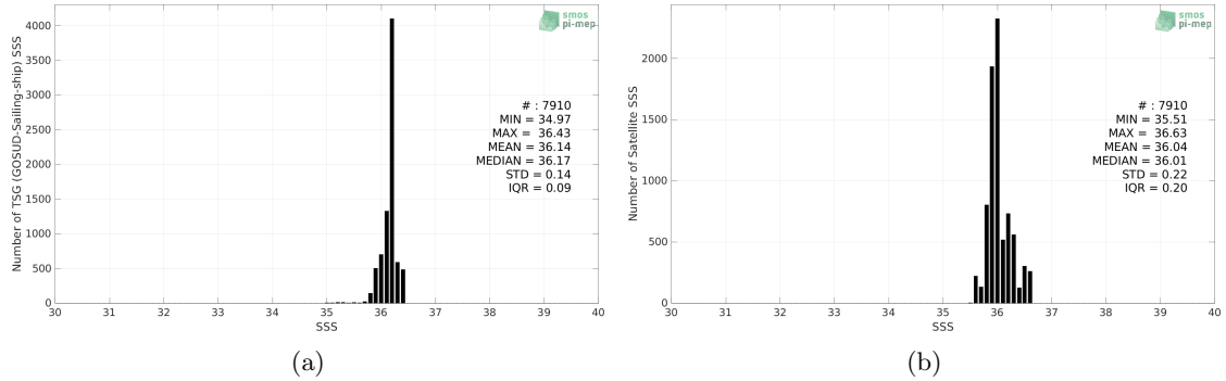
Figure 2: Histograms of SSS from TSG (GOSUD-Sailing-ship) (a) and SMOS SSS L3 v8 - 9 Days (CATDS-CECOS-LOCEAN) (b) considering all match-up pairs per bins of 0.1 over the Gulf of Mexico Pi-MEP region and for the full satellite product period.
