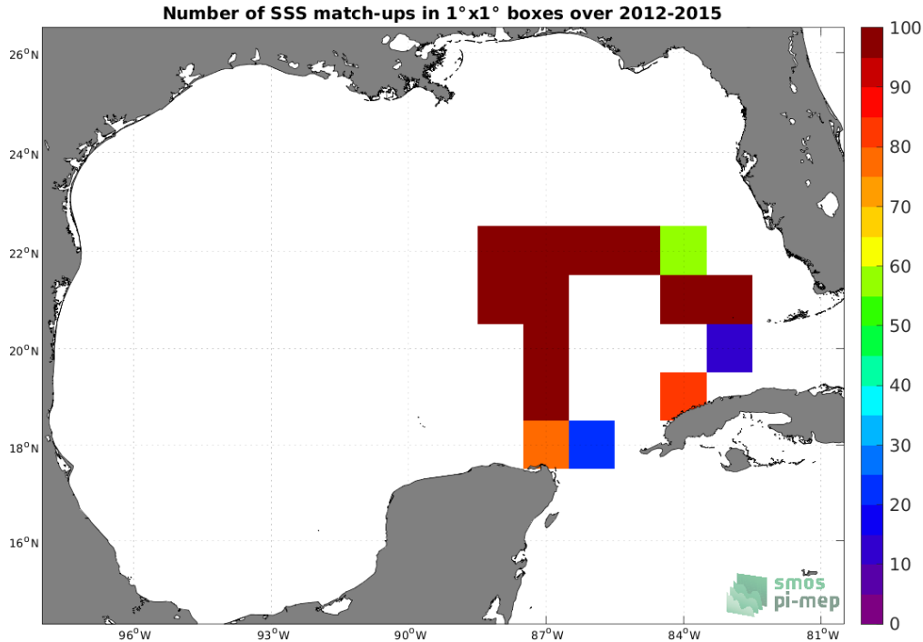
Figure 4: Number of SSS match-ups between TSG (GOSUD-Sailing-ship) SSS and the SMOS SSS L3 v8 - 9 Days (CATDS-CECOS-LOCEAN) SSS product for the Gulf of Mexico Pi-MEP region over 1^\circ \times 1^\circ boxes and for the full satellite product period.
