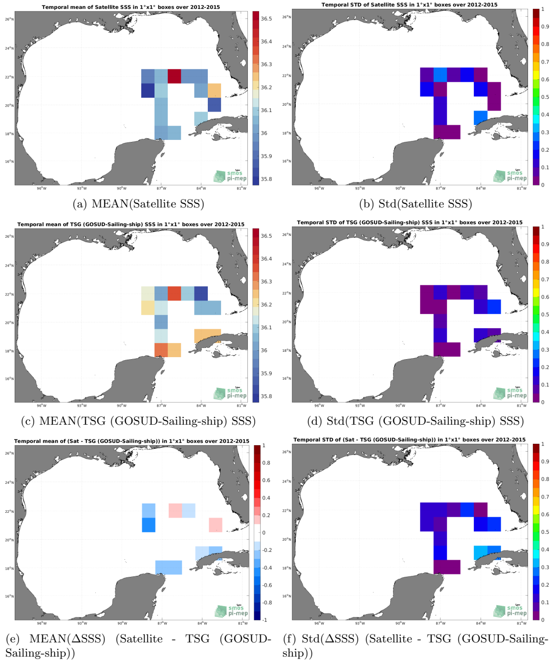
Figure 6: Temporal mean (left) and Std (right) of SSS from SMOS SSS L3 v8 - 9 Days (CATDS-CECOS-LOCEAN) (top), TSG (GOSUD-Sailing-ship) (middle), and of \Delta SSS (Satellite - TSG (GOSUD-Sailing-ship)). Only match-up pairs are used to generate these maps.
