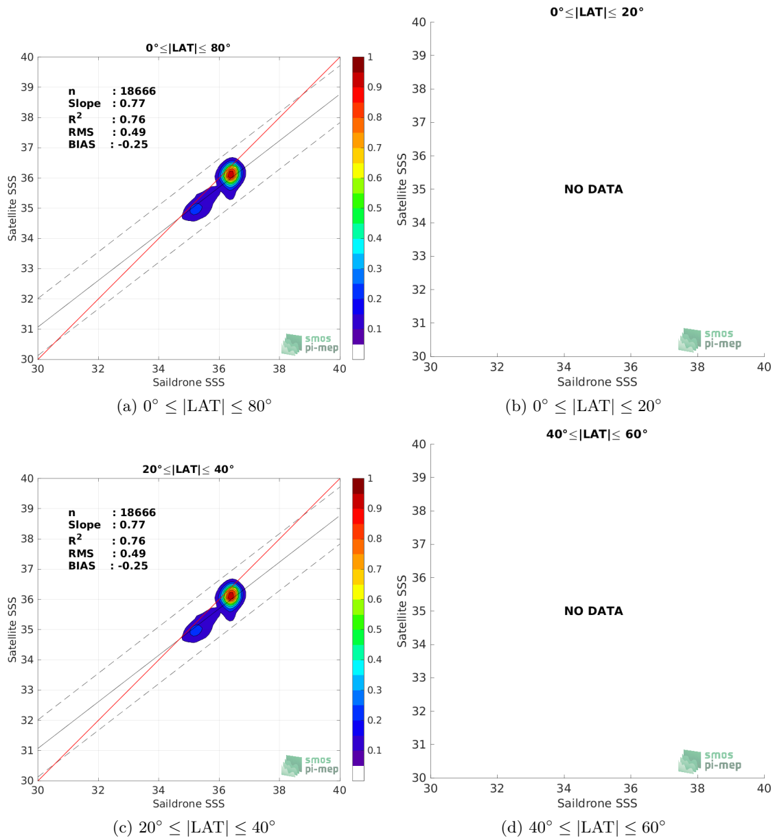
Figure 9: Contour maps of the concentration of SMOS SSS L3 v8 - 9 Days (CATDS-CECOS-LOCEAN) SSS (y-axis) versus Sailldrone SSS (x-axis) at match-up pairs for different latitude bands. For each plot, the red line shows x=y . The black thin and dashed lines indicate a linear fit through the data cloud and the \pm 95\% confidence levels, respectively. The number match-up pairs n , the slope and R^2 coefficient of the linear fit, the root mean square (RMS) and the mean bias between satellite and in situ data are indicated for each latitude band in each plots.
