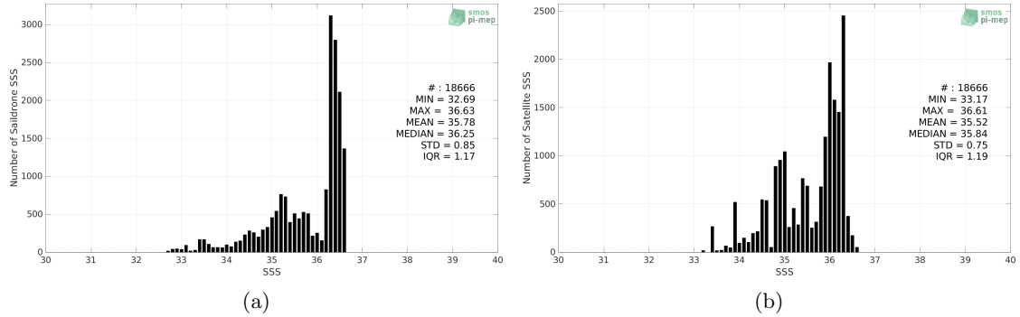
Figure 2: Histograms of SSS from Saildrone (a) and SMOS SSS L3 v8 - 9 Days (CATDS-CECOS-LOCEAN) (b) considering all match-up pairs per bins of 0.1 over the Gulf of Mexico Pi-MEP region and for the full satellite product period.
