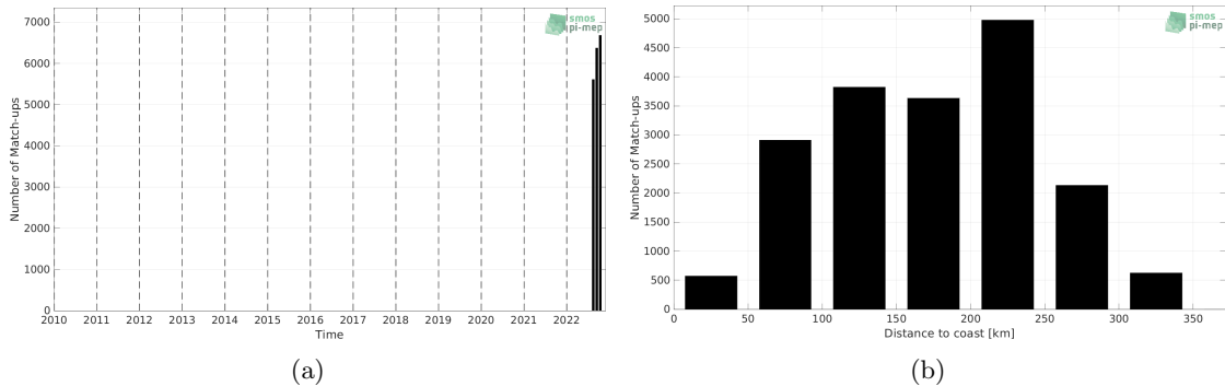
Figure 1: Number of match-ups between Saildrone and SMOS SSS L3 v8 - 9 Days (CATDS-CECOS-LOCEAN) SSS as a function of time (a) and as function of the distance to coast (b) over the Gulf of Mexico Pi-MEP region and for the full satellite product period.
