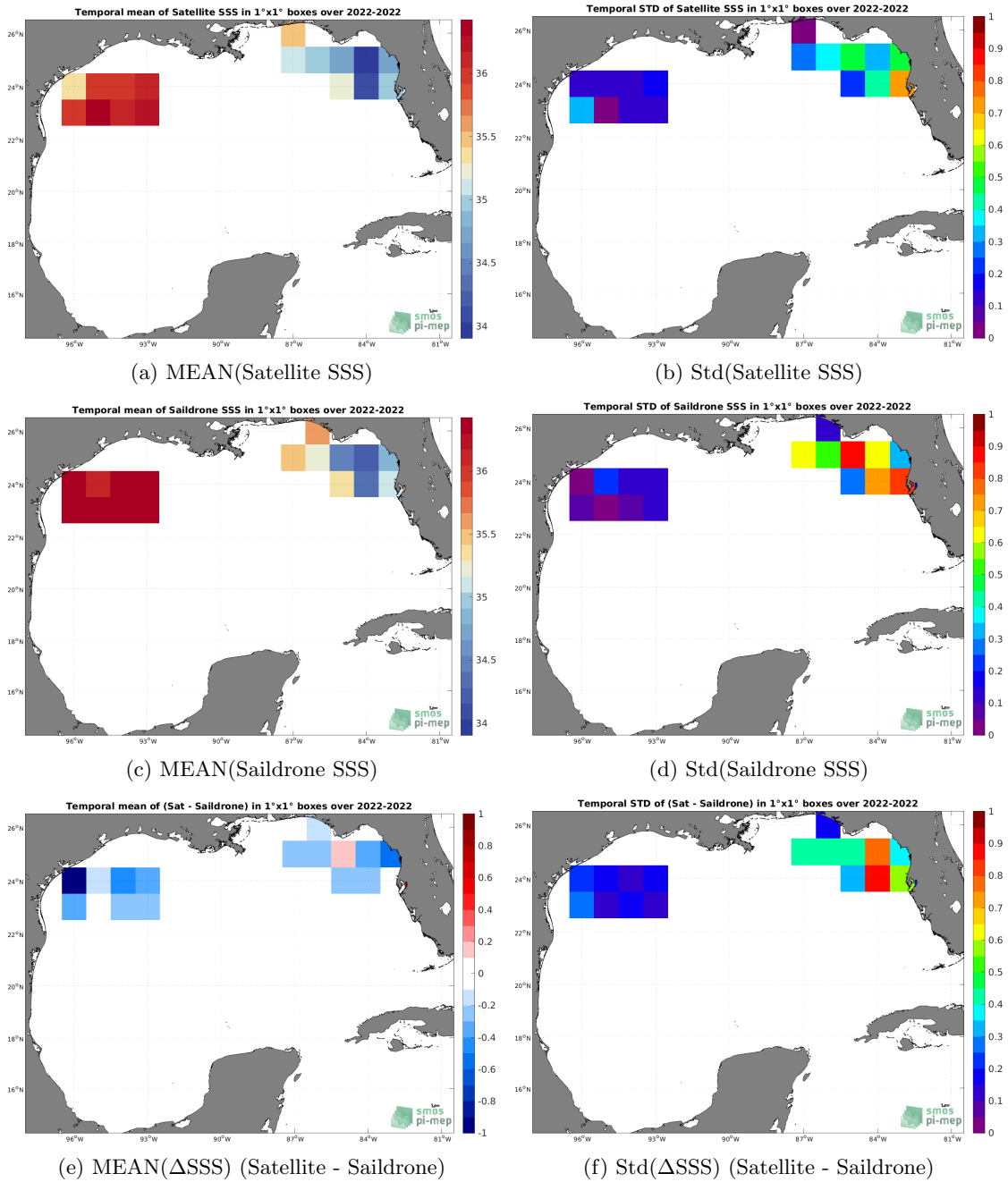
Figure 6: Temporal mean (left) and Std (right) of SSS from SMOS SSS L3 v8 - 9 Days (CATDS-CECOS-LOCEAN) (top), Saildrone (middle), and of \Delta SSS (Satellite - Saildrone). Only match-up pairs are used to generate these maps.
