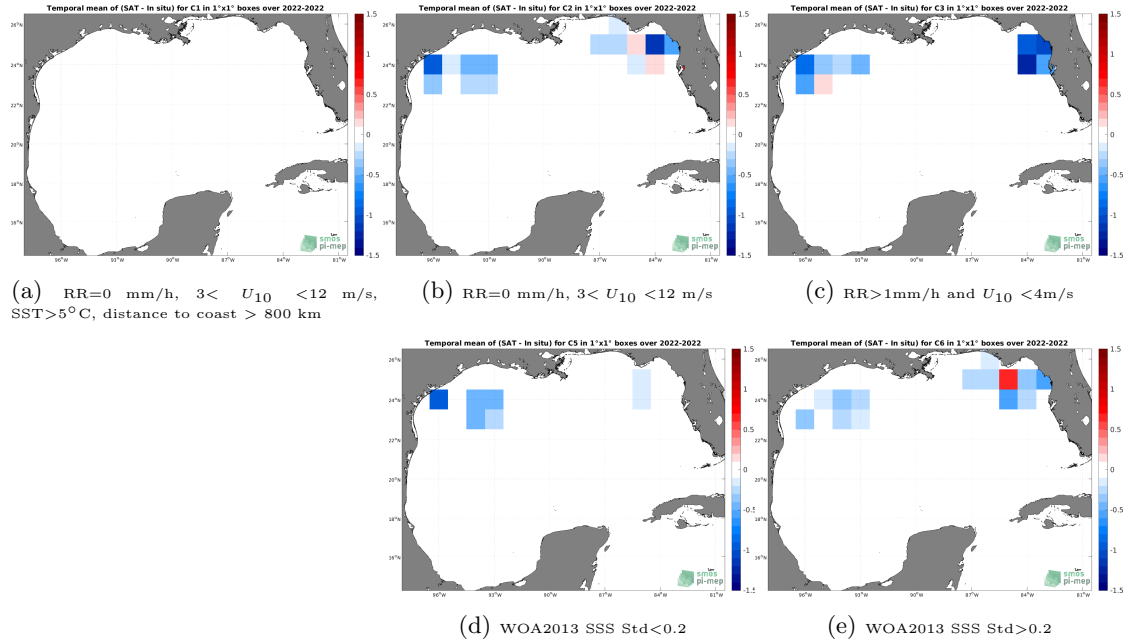
Figure 12: Temporal mean gridded over spatial boxes of size 1^{\circ}\times 1^{\circ} of \Delta\text{SSS} (SMOS SSS L3 v8 - 9 Days (CATDS-CECOS-LOCEAN) - Saildrone) for 5 different subdatasets corresponding to:RR=0 mm/h, 3 < U_{10} < 12 m/s, SST >5^{\circ}\text{C} , distance to coast > 800 km (a), RR=0 mm/h, 3 < U_{10} < 12 m/s (b), RR >1 mm/h and U_{10} < 4 m/s (c), WOA2013 SSS Std <0.2 (d), WOA2013 SSS Std >0.2 (e).
