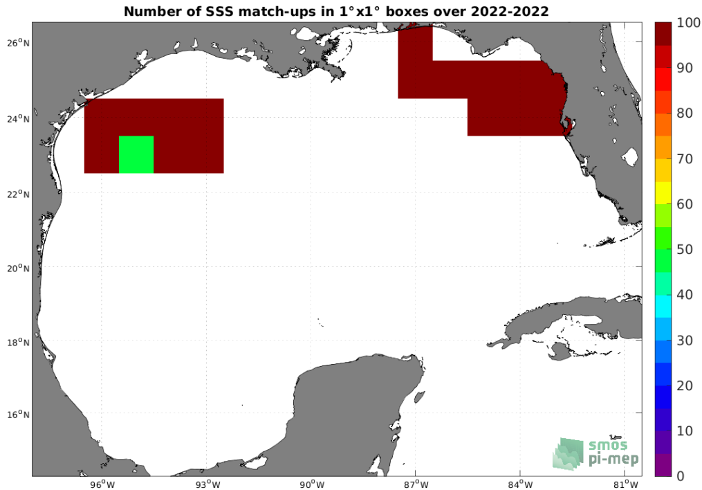
Figure 4: Number of SSS match-ups between Saildrone SSS and the SMOS SSS L3 v8 - 9 Days (CATDS-CECOS-LOCEAN) SSS product for the Gulf of Mexico Pi-MEP region over 1^\circ \times 1^\circ boxes and for the full satellite product period.
