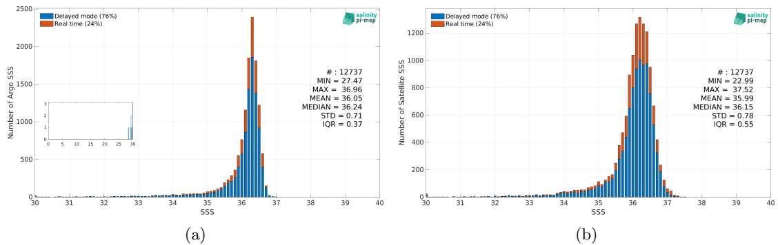
Figure 2: Histograms of SSS from Argo (a) and SMOS SSS L3 v8 - 9 Days (CATDS-CEC-LOCEAN) (b) considering all match-up pairs per bins of 0.1 over the Gulf of Mexico Pi-MEP region and for the full satellite product period.
