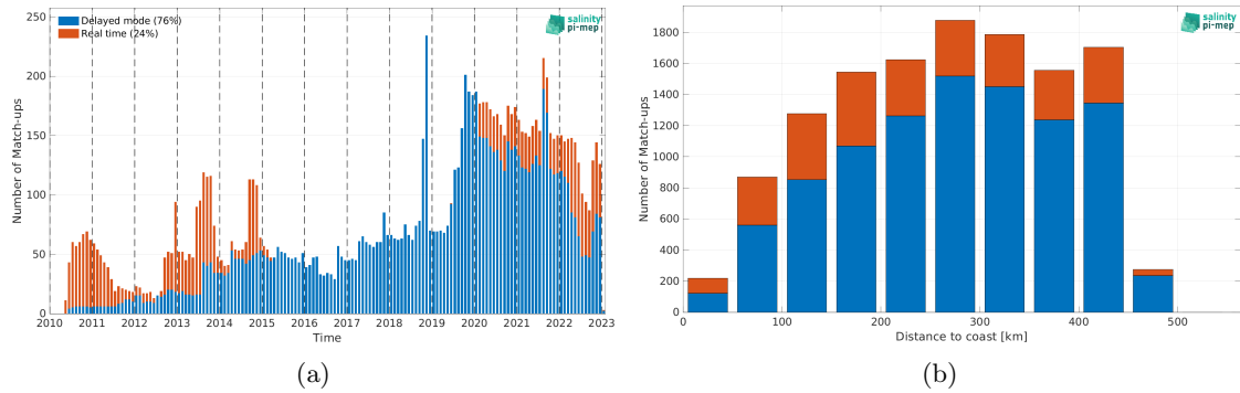
Figure 1: Number of match-ups between Argo and SMOS SSS L3 v8 - 9 Days (CATDS-CEC-LOCEAN) SSS as a function of time (a) and as function of the distance to coast (b) over the Gulf of Mexico Pi-MEP region and for the full satellite product period.
