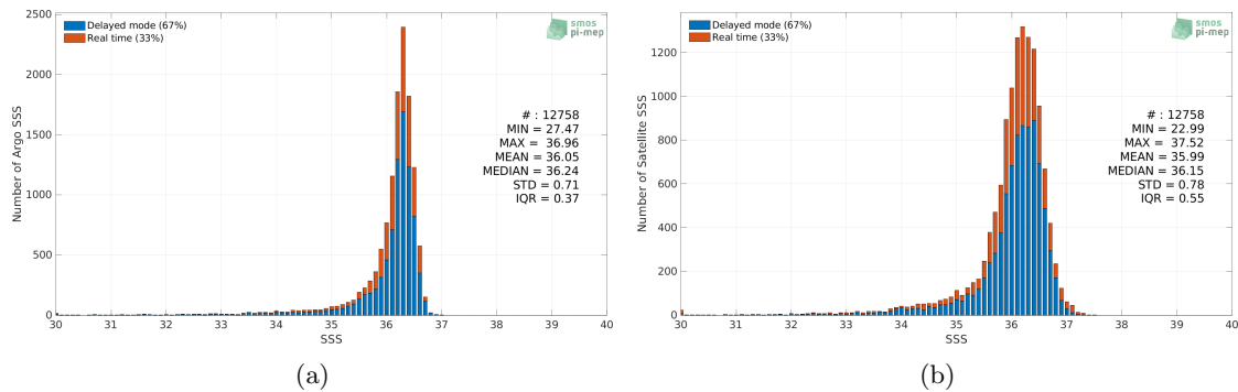
Figure 2: Histograms of SSS from Argo (a) and SMOS SSS L3 v8 - 9 Days (CATDS-CECOS-LOCEAN) (b) considering all match-up pairs per bins of 0.1 over the Gulf of Mexico Pi-MEP region and for the full satellite product period.
