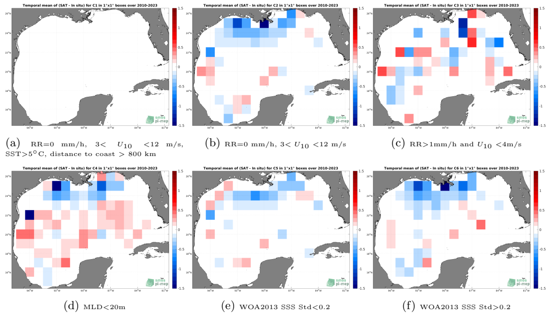
Figure 12: Temporal mean gridded over spatial boxes of size 1^\circ \times 1^\circ of \Delta SSS (SMOS SSS L3 v8 - 9 Days (CATDS-CECOS-LOCEAN) - Argo) for 6 different subdatasets corresponding to:RR=0 mm/h, 3 < U_{10} < 12 m/s, SST > 5^\circ\text{C} , distance to coast > 800 km (a), RR=0 mm/h, 3 < U_{10} < 12 m/s (b), RR > 1 mm/h and U_{10} < 4 m/s (c),MLD < 20 m (d),WOA2013 SSS Std < 0.2 (e),WOA2013 SSS Std > 0.2 (f).
