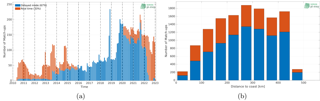
Figure 1: Number of match-ups between Argo and SMOS SSS L3 v8 - 9 Days (CATDS-CECOS-LOCEAN) SSS as a function of time (a) and as function of the distance to coast (b) over the Gulf of Mexico Pi-MEP region and for the full satellite product period.
