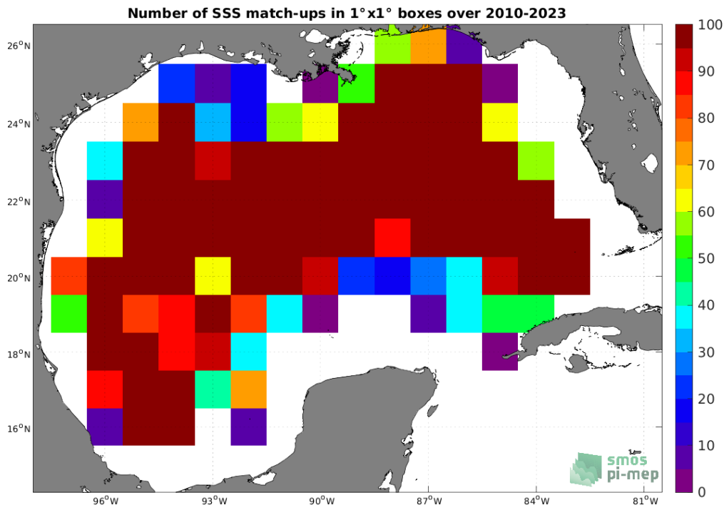
Figure 4: Number of SSS match-ups between Argo SSS and the SMOS SSS L3 v8 - 9 Days (CATDS-CECOS-LOCEAN) SSS product for the Gulf of Mexico Pi-MEP region over 1^\circ \times 1^\circ boxes and for the full satellite product period.
