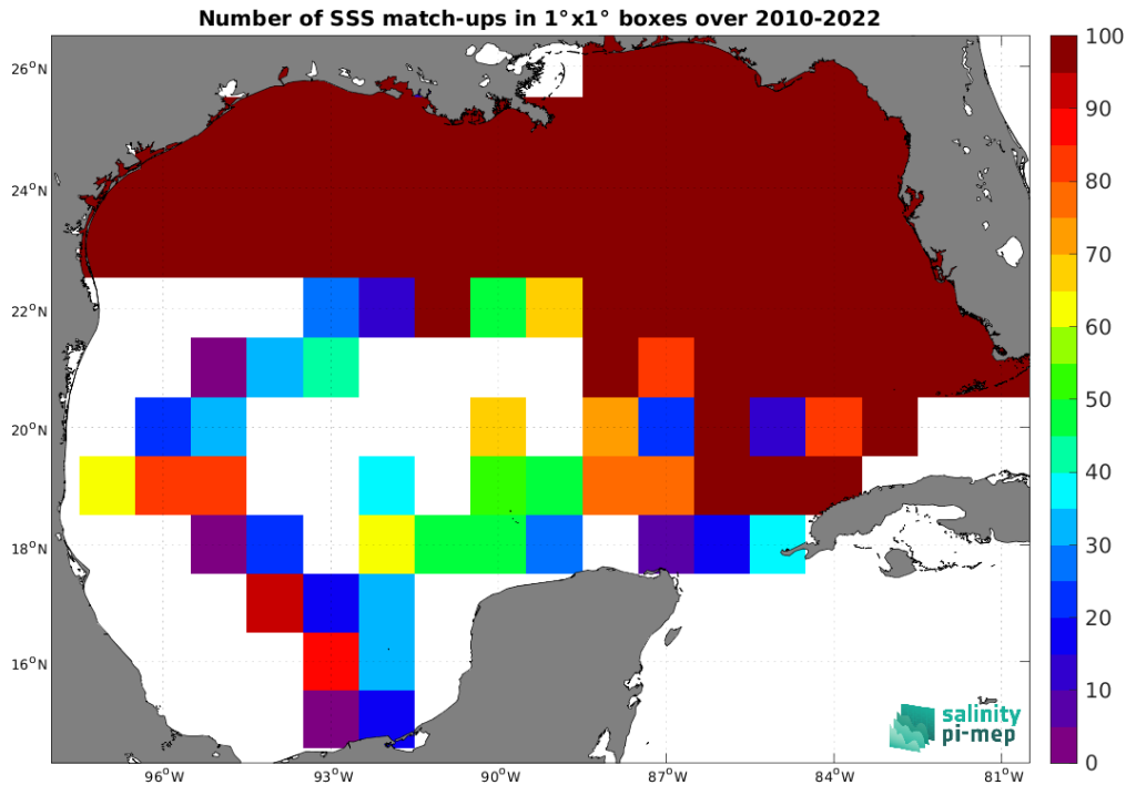
Figure 4: Number of SSS match-ups between TSG (SAMOS) SSS and the SMOS SSS L3 v8 - 18 Days (CATDS-CEC-LOCEAN) SSS product for the Gulf of Mexico Pi-MEP region over 1^\circ \times 1^\circ boxes and for the full satellite product period.
