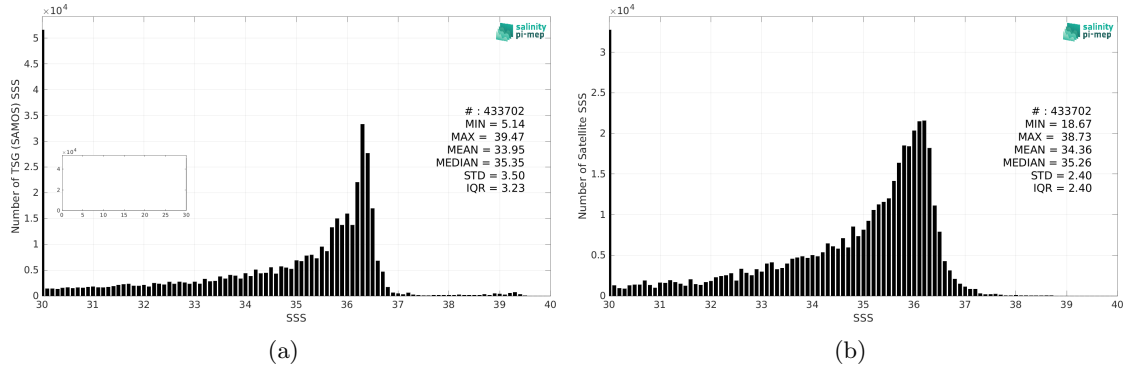
Figure 2: Histograms of SSS from TSG (SAMOS) (a) and SMOS SSS L3 v8 - 18 Days (CATDS-CEC-LOCEAN) (b) considering all match-up pairs per bins of 0.1 over the Gulf of Mexico Pi-MEP region and for the full satellite product period.
