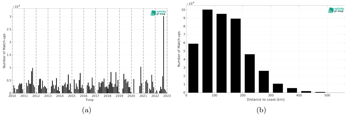
Figure 1: Number of match-ups between TSG (SAMOS) and SMOS SSS L3 v8 - 18 Days (CATDS-CEC-LOCEAN) SSS as a function of time (a) and as function of the distance to coast (b) over the Gulf of Mexico Pi-MEP region and for the full satellite product period.
