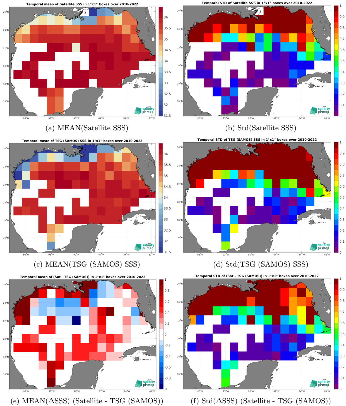
Figure 6: Temporal mean (left) and Std (right) of SSS from SMOS SSS L3 v8 - 18 Days (CATDS-CEC-LOCEAN) (top), TSG (SAMOS) (middle), and of \Delta SSS (Satellite - TSG (SAMOS)). Only match-up pairs are used to generate these maps.
