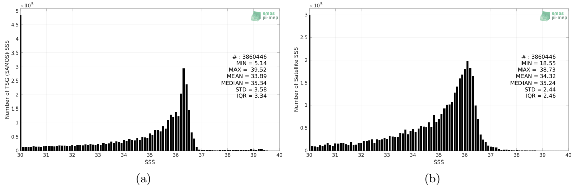
Figure 2: Histograms of SSS from TSG (SAMOS) (a) and SMOS SSS L3 v8 - 18 Days (CATDS-CECOS-LOCEAN) (b) considering all match-up pairs per bins of 0.1 over the Gulf of Mexico Pi-MEP region and for the full satellite product period.
