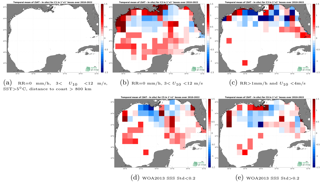
Figure 12: Temporal mean gridded over spatial boxes of size 1^{\circ}\times 1^{\circ} of \Delta\text{SSS} (SMOS SSS L3 v8 - 18 Days (CATDS-CECOS-LOCEAN) - TSG (SAMOS)) for 5 different subdatasets corresponding to:RR=0 mm/h, 3 < U_{10} < 12 m/s, SST >5^{\circ}\text{C} , distance to coast > 800 km (a), RR=0 mm/h, 3 < U_{10} < 12 m/s (b), RR >1 mm/h and U_{10} < 4 m/s (c), WOA2013 SSS Std <0.2 (d), WOA2013 SSS Std >0.2 (e).
