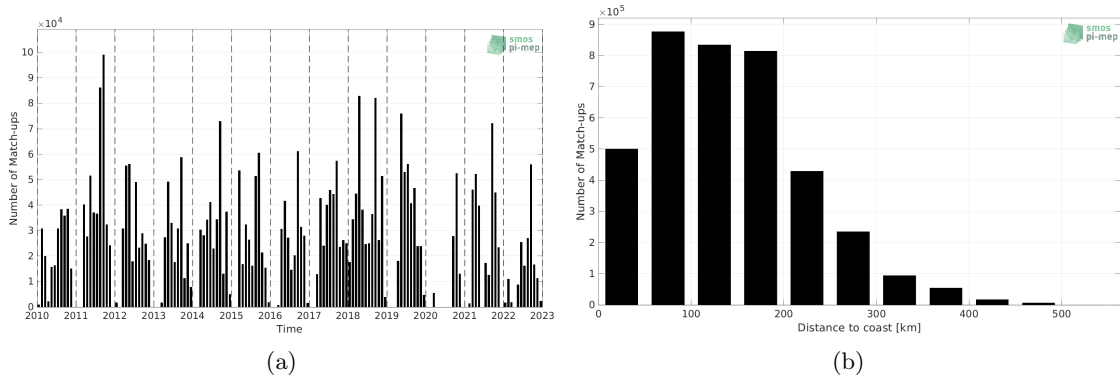
Figure 1: Number of match-ups between TSG (SAMOS) and SMOS SSS L3 v8 - 18 Days (CATDS-CECOS-LOCEAN) SSS as a function of time (a) and as function of the distance to coast (b) over the Gulf of Mexico Pi-MEP region and for the full satellite product period.
