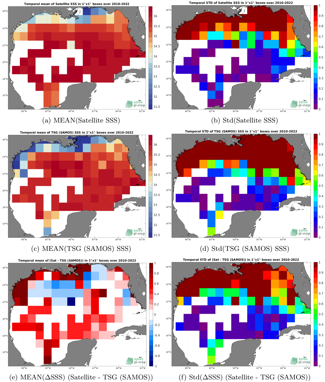
Figure 6: Temporal mean (left) and Std (right) of SSS from SMOS SSS L3 v8 - 18 Days (CATDS-CECOS-LOCEAN) (top), TSG (SAMOS) (middle), and of \Delta SSS (Satellite - TSG (SAMOS)). Only match-up pairs are used to generate these maps.
