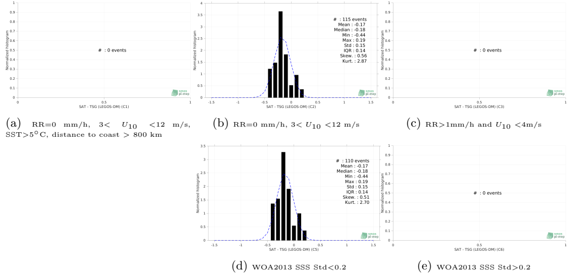
Figure 13: Normalized histogram of \Delta SSS (SMOS SSS L3 v8 - 18 Days (CATDS-CECOS-LOCEAN) - TSG (LEGOS-DM)) for 5 different subdatasets corresponding to: RR=0 mm/h, 3 < U_{10} < 12 m/s, SST > 5°C, distance to coast > 800 km (a), RR=0 mm/h, 3 < U_{10} < 12 m/s (b), RR > 1mm/h and U_{10} < 4 m/s (c), WOA2013 SSS Std < 0.2 (d), WOA2013 SSS Std > 0.2 (e).
