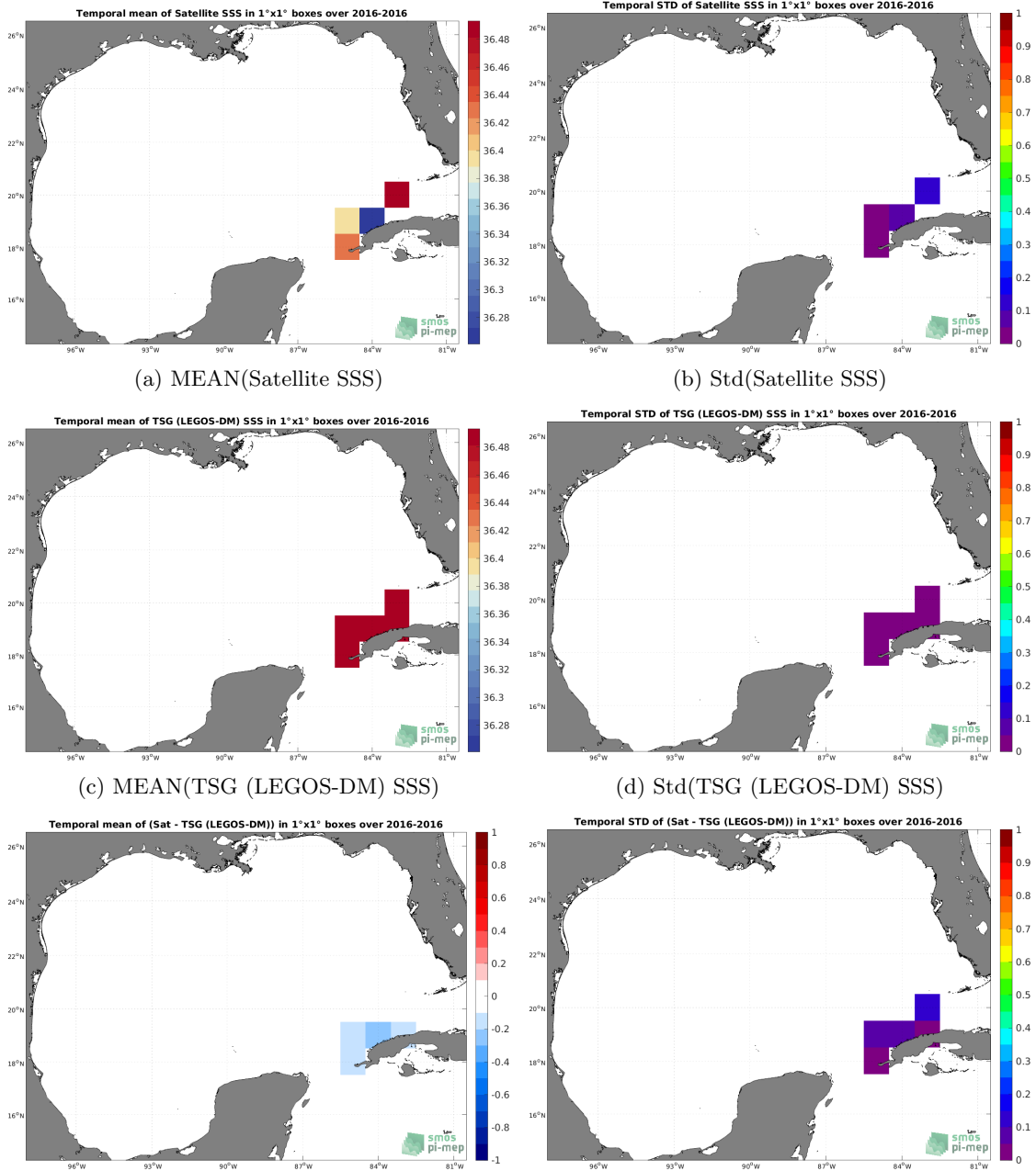
(e) MEAN( \Delta SSS) (Satellite - TSG (LEGOS-DM)) (f) Std( \Delta SSS) (Satellite - TSG (LEGOS-DM))
