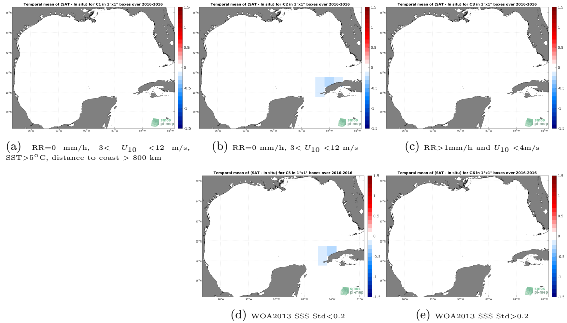
Figure 12: Temporal mean gridded over spatial boxes of size 1^{\circ}\times 1^{\circ} of \Delta\text{SSS} (SMOS SSS L3 v8 - 18 Days (CATDS-CECOS-LOCEAN) - TSG (LEGOS-DM)) for 5 different subdatasets corresponding to:RR=0 mm/h, 3 < U_{10} < 12 m/s, SST >5^{\circ}\text{C} , distance to coast > 800 km (a), RR=0 mm/h, 3 < U_{10} < 12 m/s (b), RR >1 mm/h and U_{10} < 4 m/s (c), WOA2013 SSS Std <0.2 (d), WOA2013 SSS Std >0.2 (e).
