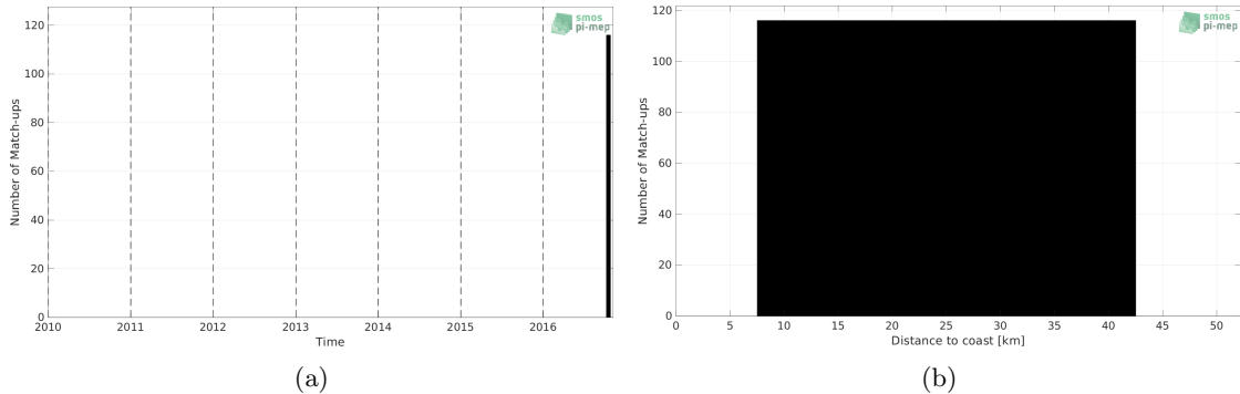
Figure 1: Number of match-ups between TSG (LEGOS-DM) and SMOS SSS L3 v8 - 18 Days (CATDS-CECOS-LOCEAN) SSS as a function of time (a) and as function of the distance to coast (b) over the Gulf of Mexico Pi-MEP region and for the full satellite product period.
