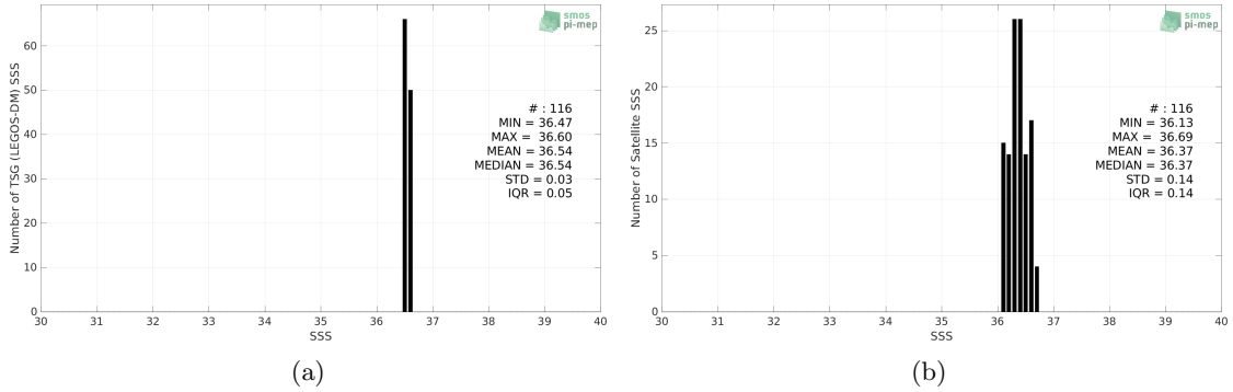
Figure 2: Histograms of SSS from TSG (LEGOS-DM) (a) and SMOS SSS L3 v8 - 18 Days (CATDS-CECOS-LOCEAN) (b) considering all match-up pairs per bins of 0.1 over the Gulf of Mexico Pi-MEP region and for the full satellite product period.
