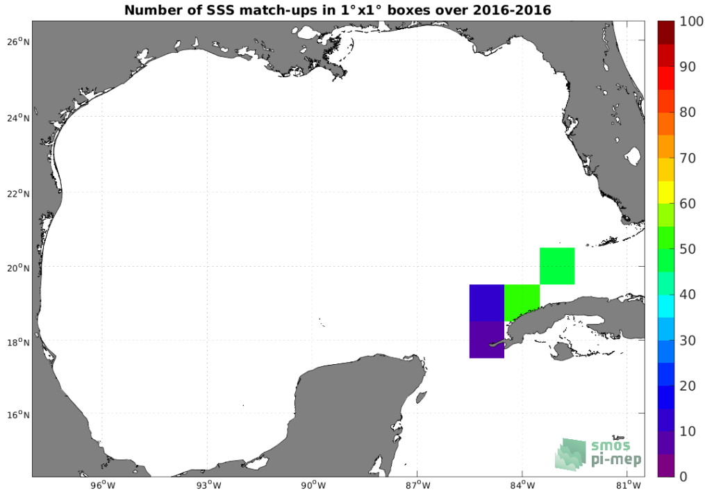
Figure 4: Number of SSS match-ups between TSG (LEGOS-DM) SSS and the SMOS SSS L3 v8 - 18 Days (CATDS-CECOS-LOCEAN) SSS product for the Gulf of Mexico Pi-MEP region over 1^\circ \times 1^\circ boxes and for the full satellite product period.
