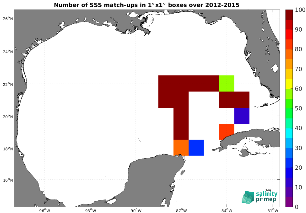
Figure 4: Number of SSS match-ups between TSG (GOSUD-Sailing-ship) SSS and the SMOS SSS L3 v8 - 18 Days (CATDS-CEC-LOCEAN) SSS product for the Gulf of Mexico Pi-MEP region over 1^\circ \times 1^\circ boxes and for the full satellite product period.
