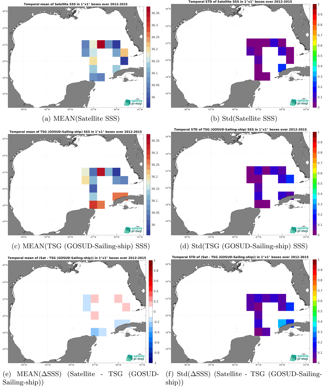
Figure 6: Temporal mean (left) and Std (right) of SSS from SMOS SSS L3 v8 - 18 Days (CATDS-CEC-LOCEAN) (top), TSG (GOSUD-Sailing-ship) (middle), and of \Delta SSS (Satellite - TSG (GOSUD-Sailing-ship)). Only match-up pairs are used to generate these maps.
