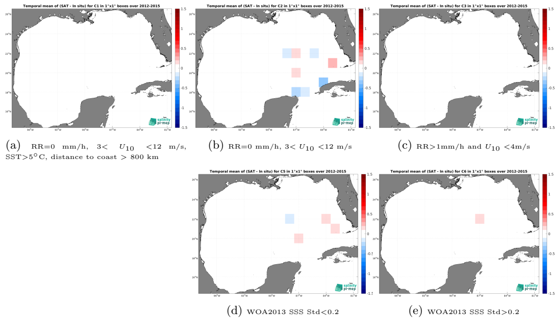
Figure 12: Temporal mean gridded over spatial boxes of size 1^{\circ}\times 1^{\circ} of \Delta SSS (SMOS SSS L3 v8 - 18 Days (CATDS-CEC-LOCEAN) - TSG (GOSUD-Sailing-ship)) for 5 different subdatasets corresponding to:RR=0 mm/h, 3 < U_{10} < 12 m/s, SST >5^{\circ}\text{C} , distance to coast > 800 km (a), RR=0 mm/h, 3 < U_{10} < 12 m/s (b), RR >1 mm/h and U_{10} < 4 m/s (c), WOA2013 SSS Std <0.2 (d), WOA2013 SSS Std >0.2 (e).
