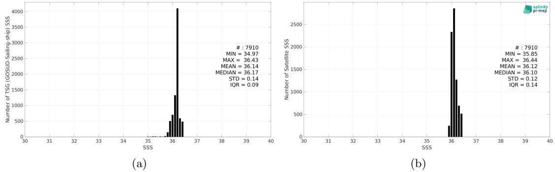
Figure 2: Histograms of SSS from TSG (GOSUD-Sailing-ship) (a) and SMOS SSS L3 v8 - 18 Days (CATDS-CEC-LOCEAN) (b) considering all match-up pairs per bins of 0.1 over the Gulf of Mexico Pi-MEP region and for the full satellite product period.
