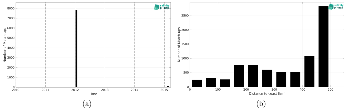
Figure 1: Number of match-ups between TSG (GOSUD-Sailing-ship) and SMOS SSS L3 v8 - 18 Days (CATDS-CEC-LOCEAN) SSS as a function of time (a) and as function of the distance to coast (b) over the Gulf of Mexico Pi-MEP region and for the full satellite product period.
