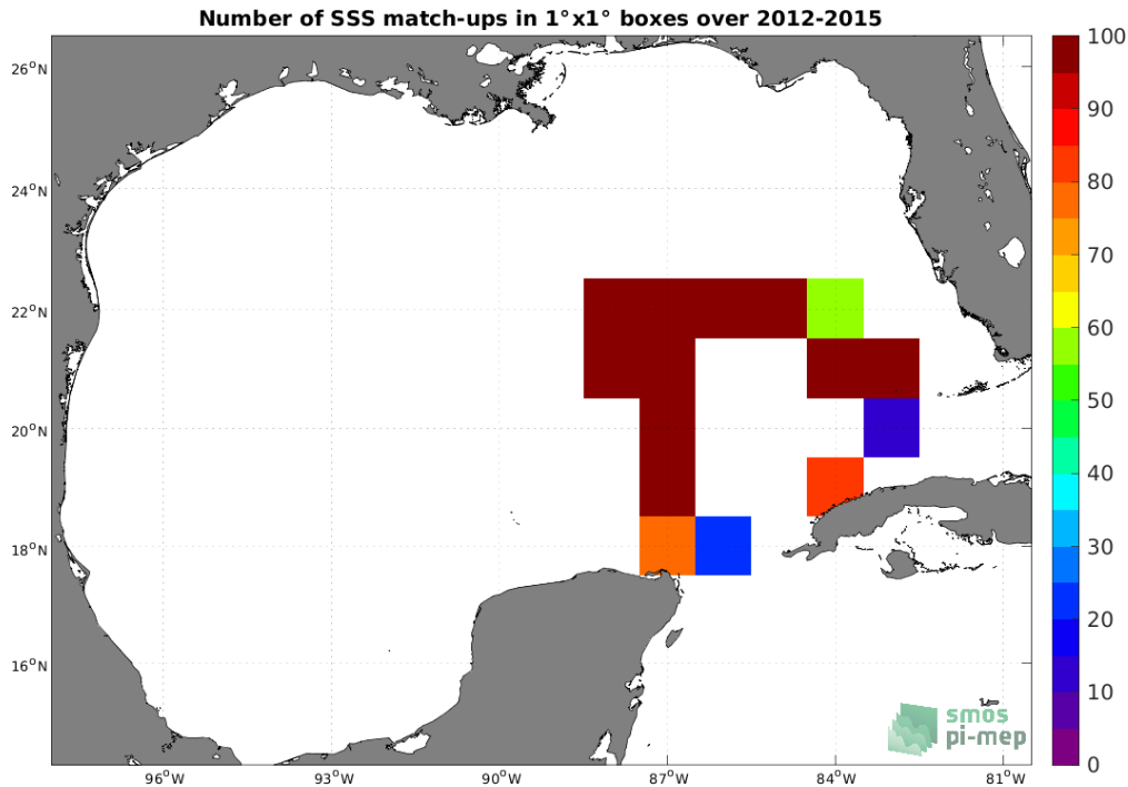
Figure 4: Number of SSS match-ups between TSG (GOSUD-Sailing-ship) SSS and the SMOS SSS L3 v8 - 18 Days (CATDS-CECOS-LOCEAN) SSS product for the Gulf of Mexico Pi-MEP region over 1^\circ \times 1^\circ boxes and for the full satellite product period.
