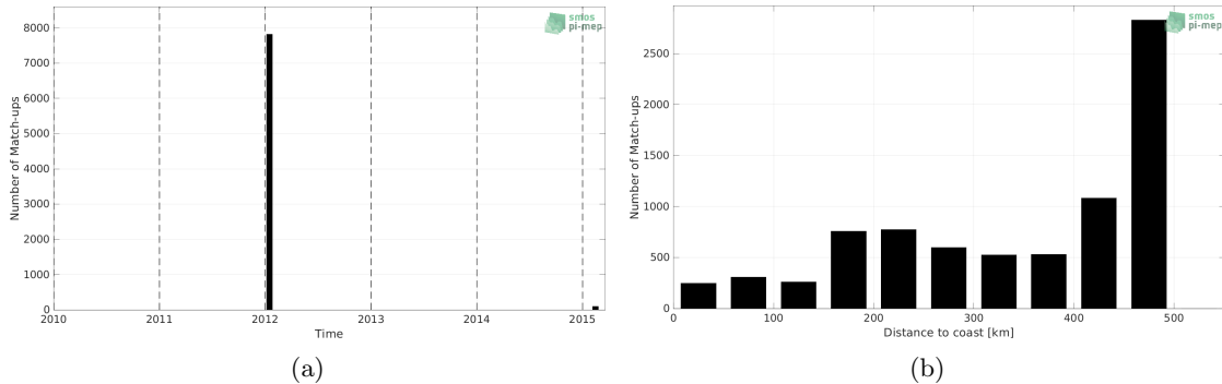
Figure 1: Number of match-ups between TSG (GOSUD-Sailing-ship) and SMOS SSS L3 v8 - 18 Days (CATDS-CECOS-LOCEAN) SSS as a function of time (a) and as function of the distance to coast (b) over the Gulf of Mexico Pi-MEP region and for the full satellite product period.
