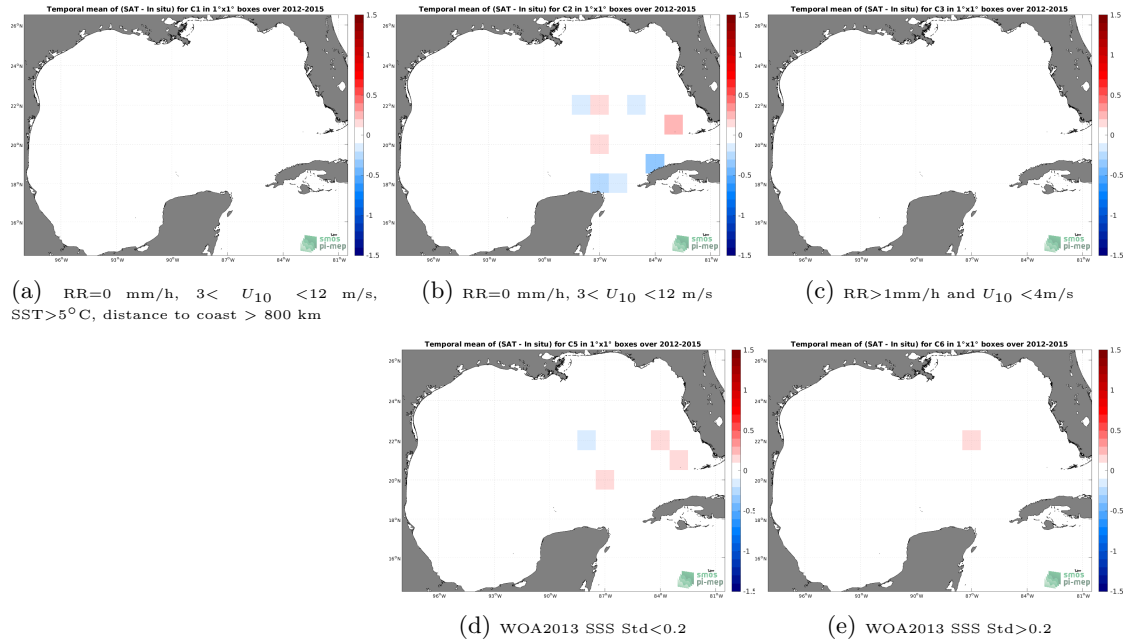
Figure 12: Temporal mean gridded over spatial boxes of size 1^{\circ}\times 1^{\circ} of \Delta SSS (SMOS SSS L3 v8 - 18 Days (CATDS-CECOS-LOCEAN) - TSG (GOSUD-Sailing-ship)) for 5 different subdatasets corresponding to:RR=0 mm/h, 3 < U_{10} < 12 m/s, SST >5^{\circ}\text{C} , distance to coast > 800 km (a), RR=0 mm/h, 3 < U_{10} < 12 m/s (b), RR >1 mm/h and U_{10} < 4 m/s (c), WOA2013 SSS Std <0.2 (d), WOA2013 SSS Std >0.2 (e).
