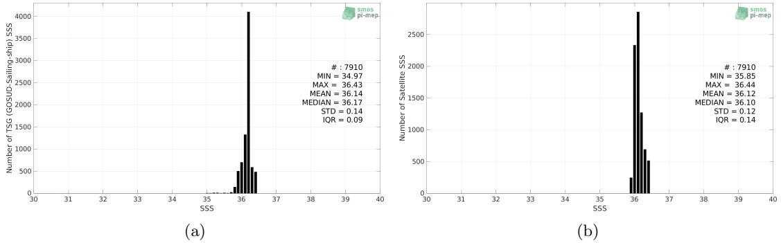
Figure 2: Histograms of SSS from TSG (GOSUD-Sailing-ship) (a) and SMOS SSS L3 v8 - 18 Days (CATDS-CECOS-LOCEAN) (b) considering all match-up pairs per bins of 0.1 over the Gulf of Mexico Pi-MEP region and for the full satellite product period.
