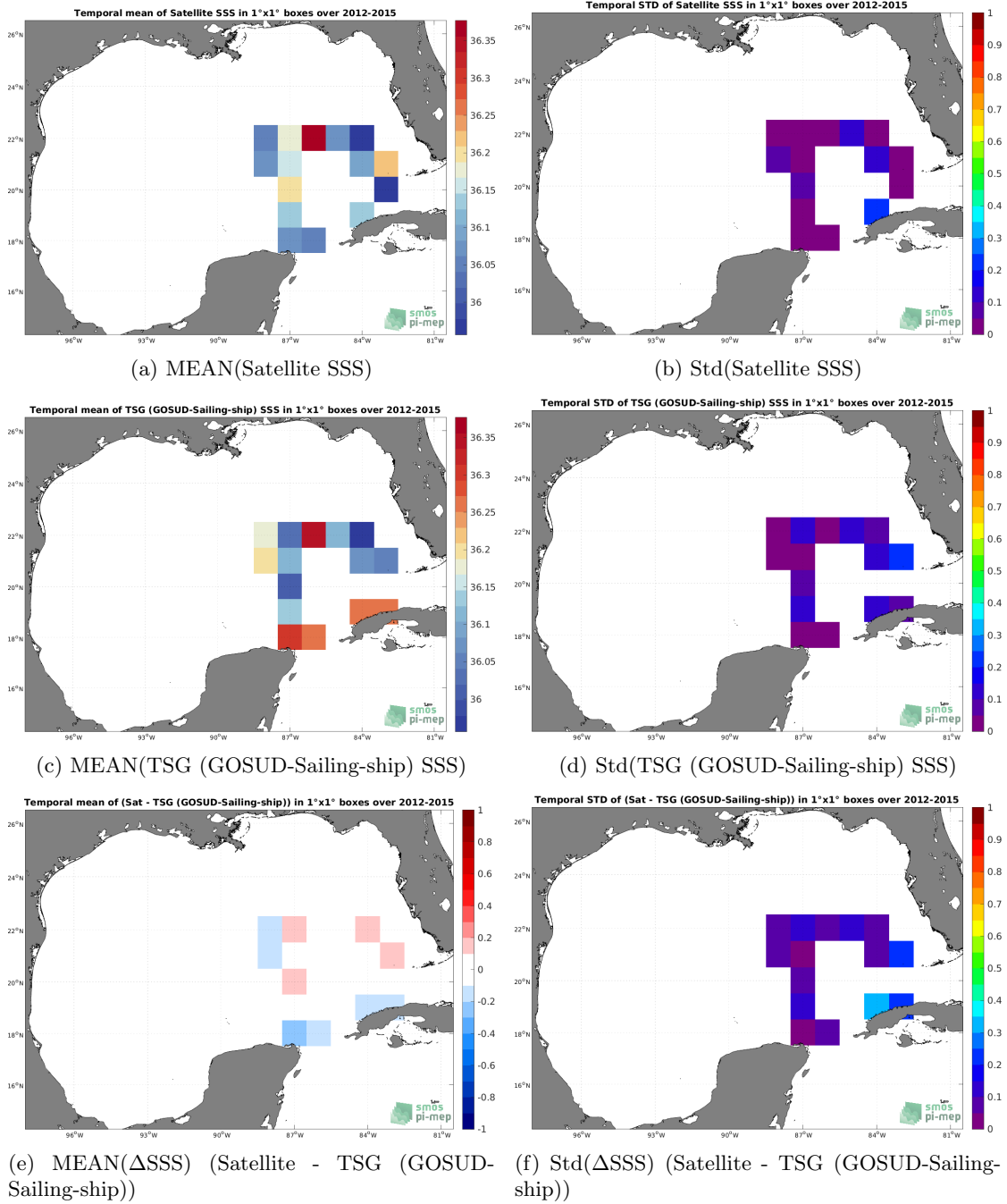
Figure 6: Temporal mean (left) and Std (right) of SSS from SMOS SSS L3 v8 - 18 Days (CATDS-CECOS-LOCEAN) (top), TSG (GOSUD-Sailing-ship) (middle), and of \Delta SSS (Satellite - TSG (GOSUD-Sailing-ship)). Only match-up pairs are used to generate these maps.
