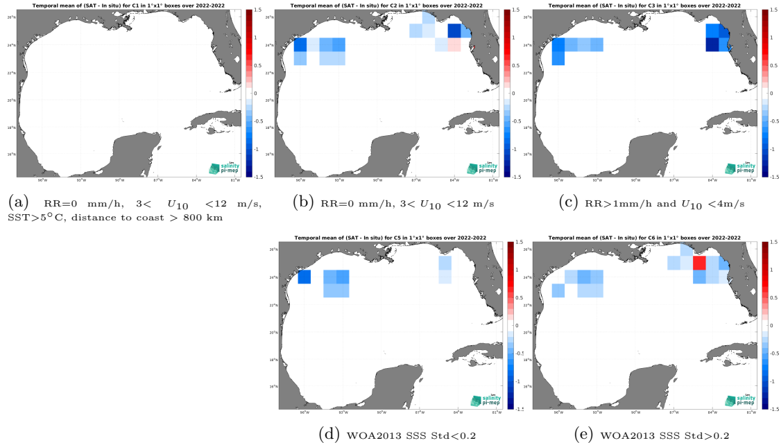
Figure 12: Temporal mean gridded over spatial boxes of size 1^{\circ}\times 1^{\circ} of \Delta\text{SSS} (SMOS SSS L3 v8 - 18 Days (CATDS-CEC-LOCEAN) - Saildrone) for 5 different subdatasets corresponding to:RR=0 mm/h, 3 < U_{10} < 12 m/s, SST >5^{\circ}\text{C} , distance to coast > 800 km (a), RR=0 mm/h, 3 < U_{10} < 12 m/s (b), RR >1 mm/h and U_{10} < 4 m/s (c), WOA2013 SSS Std <0.2 (d), WOA2013 SSS Std >0.2 (e).
