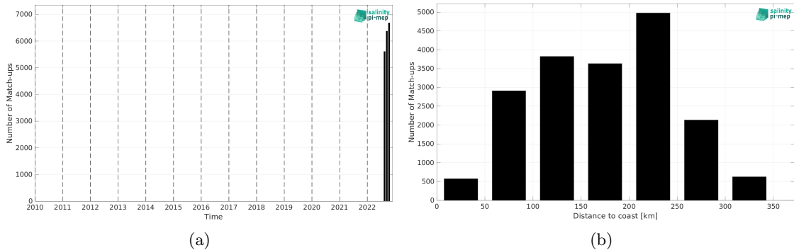
Figure 1: Number of match-ups between Saildrone and SMOS SSS L3 v8 - 18 Days (CATDS-CEC-LOCEAN) SSS as a function of time (a) and as function of the distance to coast (b) over the Gulf of Mexico Pi-MEP region and for the full satellite product period.
