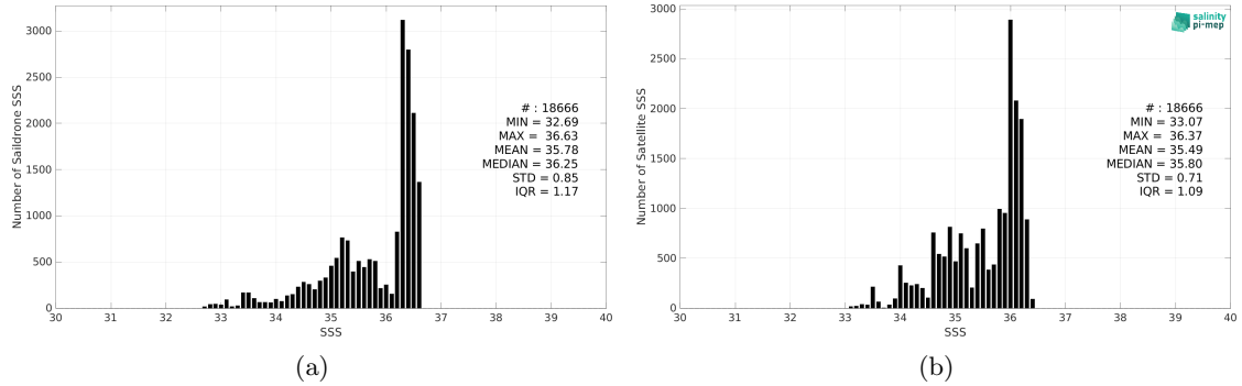
Figure 2: Histograms of SSS from Sairdrone (a) and SMOS SSS L3 v8 - 18 Days (CATDS-CEC-LOCEAN) (b) considering all match-up pairs per bins of 0.1 over the Gulf of Mexico Pi-MEP region and for the full satellite product period.
