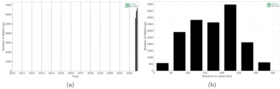
Figure 1: Number of match-ups between Saildrone and SMOS SSS L3 v8 - 18 Days (CATDS-CECOS-LOCEAN) SSS as a function of time (a) and as function of the distance to coast (b) over the Gulf of Mexico Pi-MEP region and for the full satellite product period.
