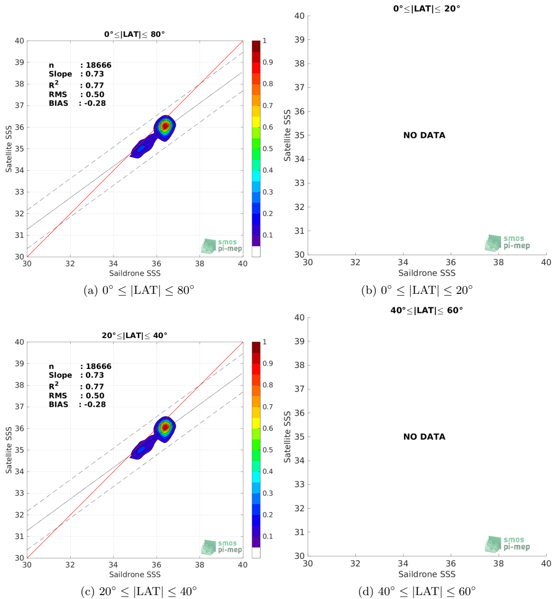
Figure 9: Contour maps of the concentration of SMOS SSS L3 v8 - 18 Days (CATDS-CECOS-LOCEAN) SSS (y-axis) versus Sailldrone SSS (x-axis) at match-up pairs for different latitude bands. For each plot, the red line shows x=y . The black thin and dashed lines indicate a linear fit through the data cloud and the \pm 95\% confidence levels, respectively. The number match-up pairs n , the slope and R^2 coefficient of the linear fit, the root mean square (RMS) and the mean bias between satellite and in situ data are indicated for each latitude band in each plots.
