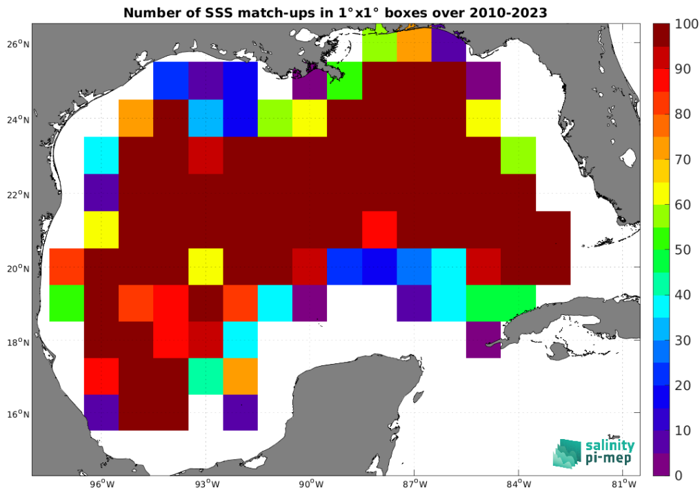
Figure 4: Number of SSS match-ups between Argo SSS and the SMOS SSS L3 v8 - 18 Days (CATDS-CEC-LOCEAN) SSS product for the Gulf of Mexico Pi-MEP region over 1^\circ \times 1^\circ boxes and for the full satellite product period.
