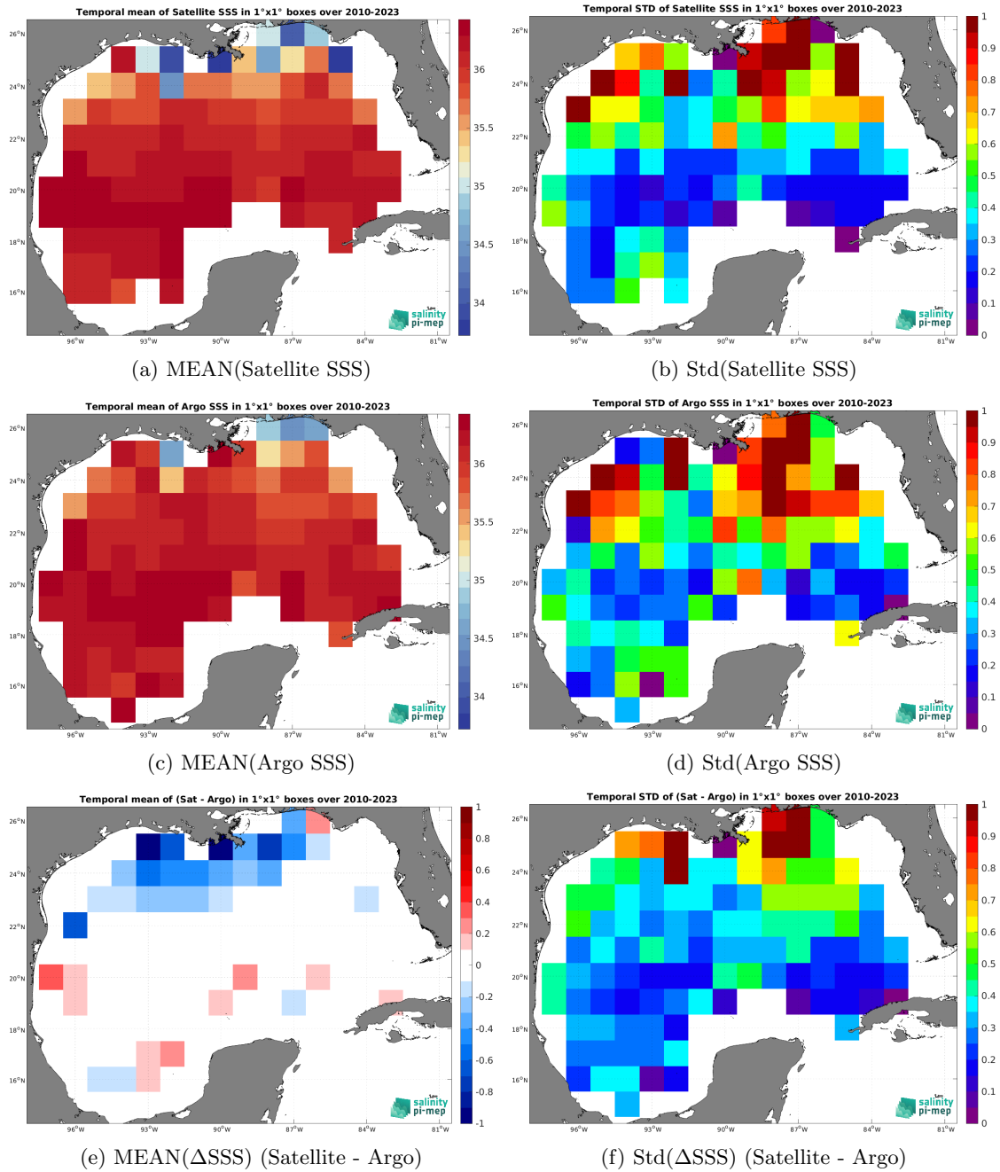
Figure 6: Temporal mean (left) and Std (right) of SSS from SMOS SSS L3 v8 - 18 Days (CATDS-CEC-LOCEAN) (top), Argo (middle), and of \Delta SSS (Satellite - Argo). Only match-up pairs are used to generate these maps.
