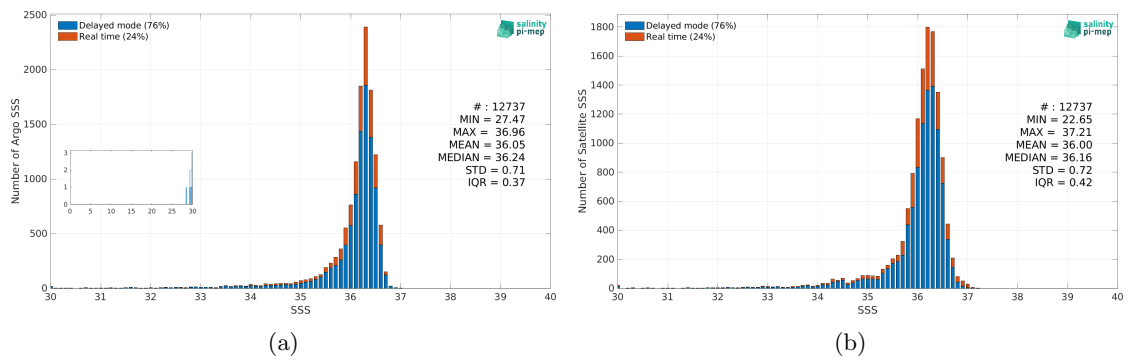
Figure 2: Histograms of SSS from Argo (a) and SMOS SSS L3 v8 - 18 Days (CATDS-CEC-LOCEAN) (b) considering all match-up pairs per bins of 0.1 over the Gulf of Mexico Pi-MEP region and for the full satellite product period.
