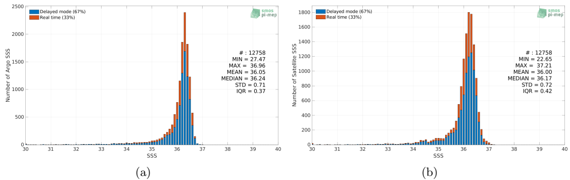
Figure 2: Histograms of SSS from Argo (a) and SMOS SSS L3 v8 - 18 Days (CATDS-CECOS-LOCEAN) (b) considering all match-up pairs per bins of 0.1 over the Gulf of Mexico Pi-MEP region and for the full satellite product period.
