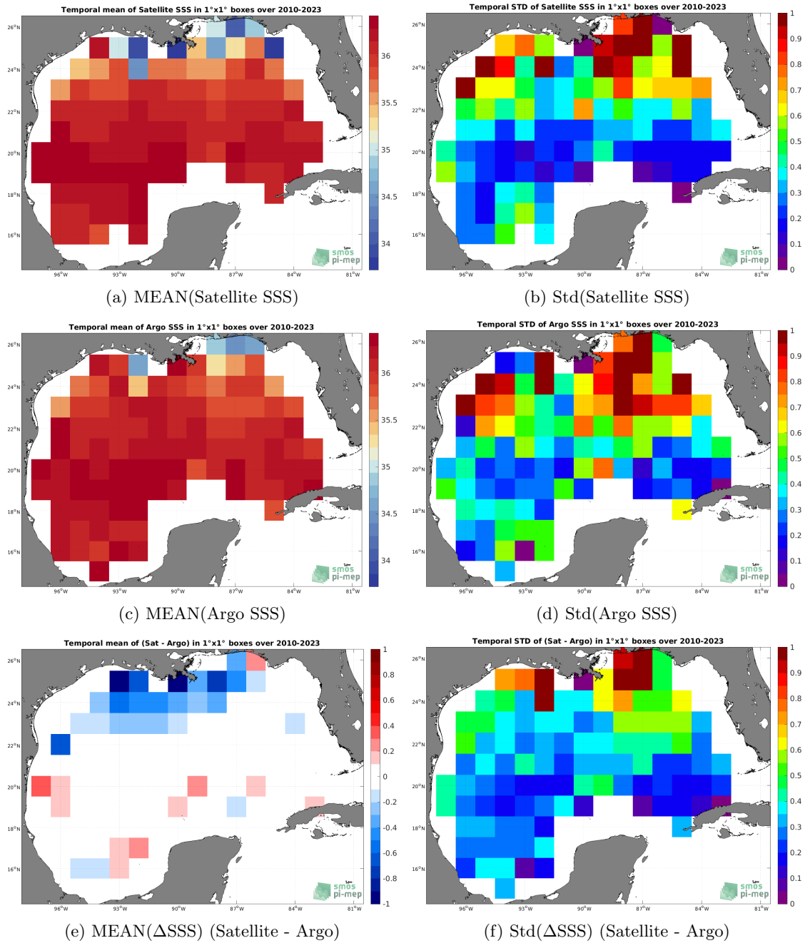
Figure 6: Temporal mean (left) and Std (right) of SSS from SMOS SSS L3 v8 - 18 Days (CATDS-CECOS-LOCEAN) (top), Argo (middle), and of \Delta SSS (Satellite - Argo). Only match-up pairs are used to generate these maps.
