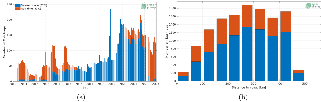
Figure 1: Number of match-ups between Argo and SMOS SSS L3 v8 - 18 Days (CATDS-CECOS-LOCEAN) SSS as a function of time (a) and as function of the distance to coast (b) over the Gulf of Mexico Pi-MEP region and for the full satellite product period.
