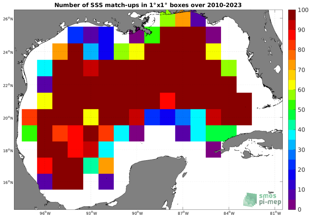
Figure 4: Number of SSS match-ups between Argo SSS and the SMOS SSS L3 v8 - 18 Days (CATDS-CECOS-LOCEAN) SSS product for the Gulf of Mexico Pi-MEP region over 1^\circ \times 1^\circ boxes and for the full satellite product period.
