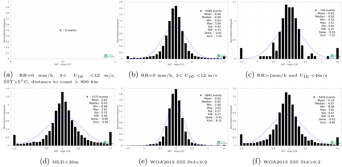
Figure 13: Normalized histogram of \Delta\text{SSS} (SMOS SSS L3 v8 - 18 Days (CATDS-CECOS-LOCEAN) - Argo) for 6 different subdatasets corresponding to: RR=0 mm/h, 3 < U_{10} < 12 m/s, SST>5°C, distance to coast > 800 km (a), RR=0 mm/h, 3 < U_{10} < 12 m/s (b), RR>1mm/h and U_{10} < 4 m/s (c), MLD<20m (d), WOA2013 SSS Std<0.2 (e), WOA2013 SSS Std>0.2 (f).
