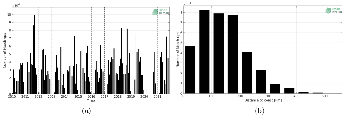
Figure 1: Number of match-ups between TSG (SAMOS) and SMOS SSS L3 v7 - 9 Days (CATDS-CECOS-LOCEAN) SSS as a function of time (a) and as function of the distance to coast (b) over the Gulf of Mexico Pi-MEP region and for the full satellite product period.
