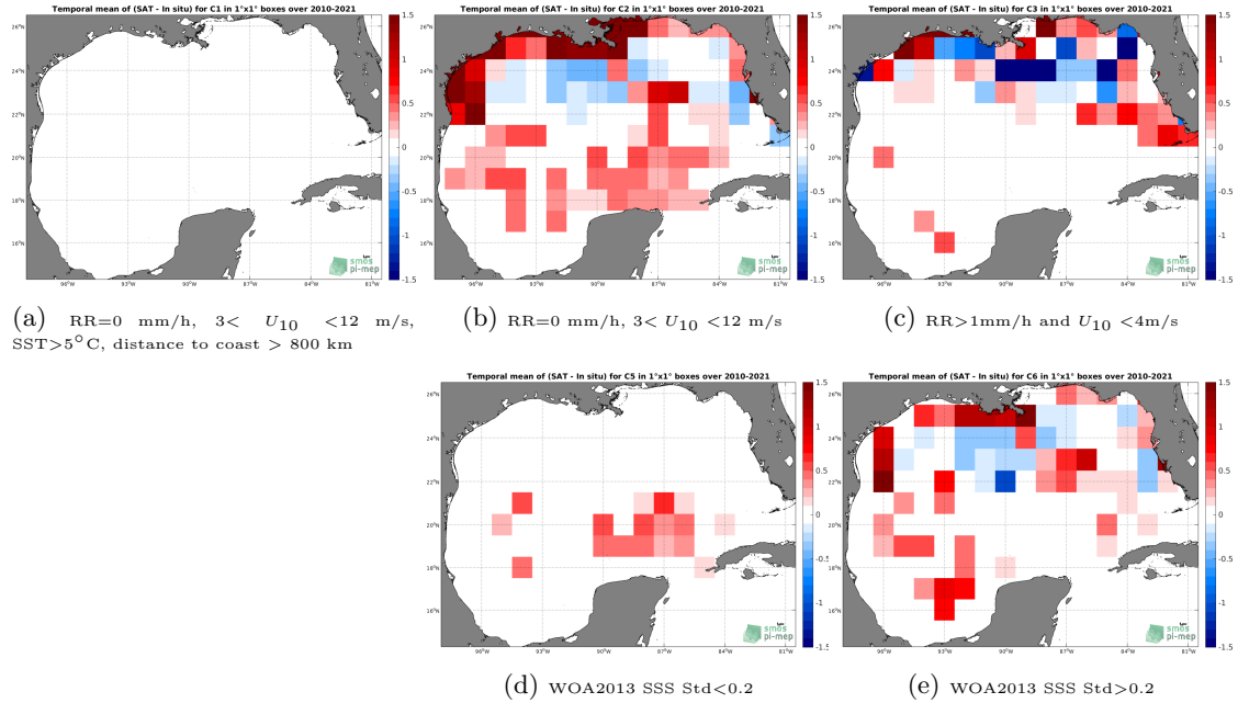
Figure 12: Temporal mean gridded over spatial boxes of size 1^{\circ}\times 1^{\circ} of \Delta\text{SSS} (SMOS SSS L3 v7 - 9 Days (CATDS-CECOS-LOCEAN) - TSG (SAMOS)) for 5 different subdatasets corresponding to:RR=0 mm/h, 3 < U_{10} < 12 m/s, SST >5^{\circ}\text{C} , distance to coast > 800 km (a), RR=0 mm/h, 3 < U_{10} < 12 m/s (b), RR >1 mm/h and U_{10} < 4 m/s (c), WOA2013 SSS Std <0.2 (d), WOA2013 SSS Std >0.2 (e).
