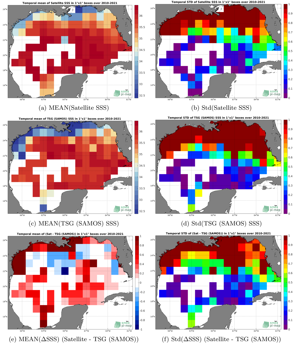
Figure 6: Temporal mean (left) and Std (right) of SSS from SMOS SSS L3 v7 - 9 Days (CATDS-CECOS-LOCEAN) (top), TSG (SAMOS) (middle), and of \Delta SSS (Satellite - TSG (SAMOS)). Only match-up pairs are used to generate these maps.
