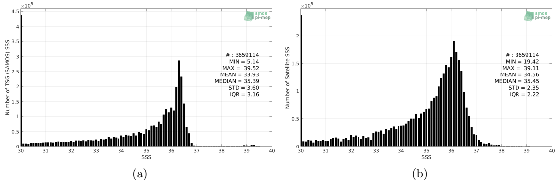
Figure 2: Histograms of SSS from TSG (SAMOS) (a) and SMOS SSS L3 v7 - 9 Days (CATDS-CECOS-LOCEAN) (b) considering all match-up pairs per bins of 0.1 over the Gulf of Mexico Pi-MEP region and for the full satellite product period.
