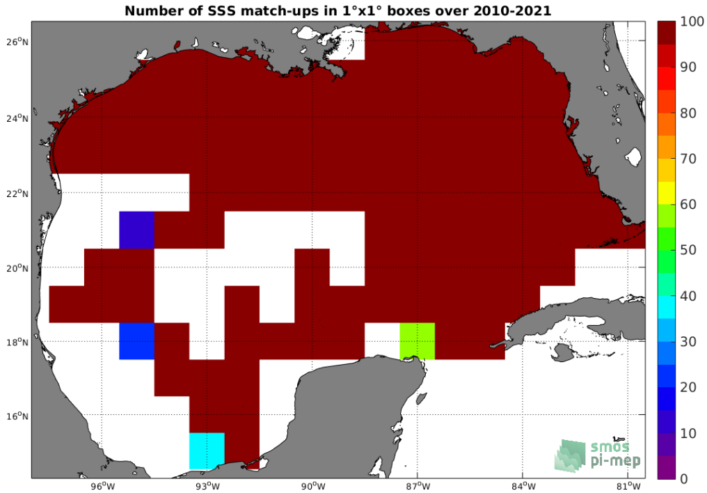
Figure 4: Number of SSS match-ups between TSG (SAMOS) SSS and the SMOS SSS L3 v7 - 9 Days (CATDS-CECOS-LOCEAN) SSS product for the Gulf of Mexico Pi-MEP region over 1^\circ \times 1^\circ boxes and for the full satellite product period.
