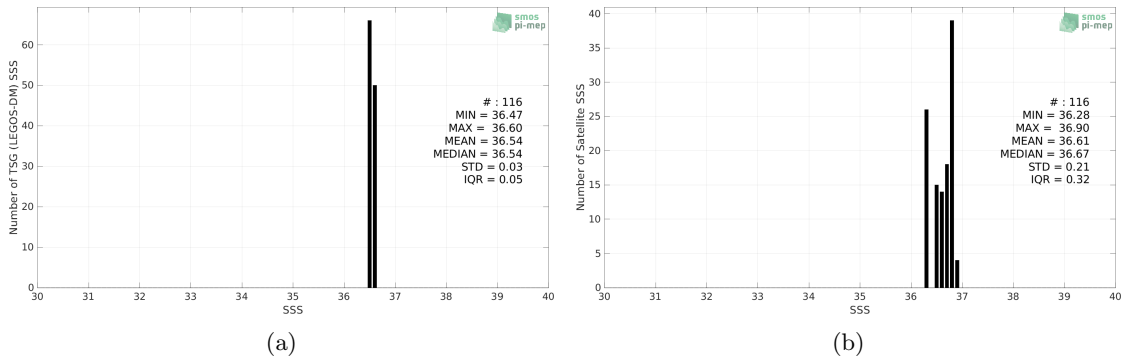
Figure 2: Histograms of SSS from TSG (LEGOS-DM) (a) and SMOS SSS L3 v7 - 9 Days (CATDS-CECOS-LOCEAN) (b) considering all match-up pairs per bins of 0.1 over the Gulf of Mexico Pi-MEP region and for the full satellite product period.
