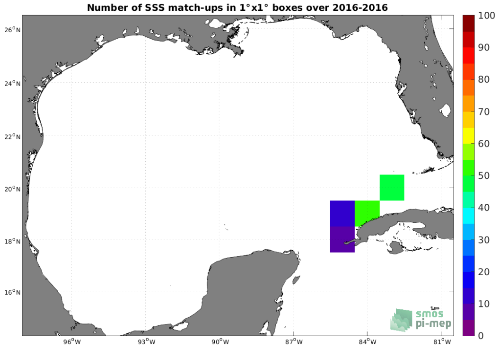
Figure 4: Number of SSS match-ups between TSG (LEGOS-DM) SSS and the SMOS SSS L3 v7 - 9 Days (CATDS-CECOS-LOCEAN) SSS product for the Gulf of Mexico Pi-MEP region over 1^\circ \times 1^\circ boxes and for the full satellite product period.
