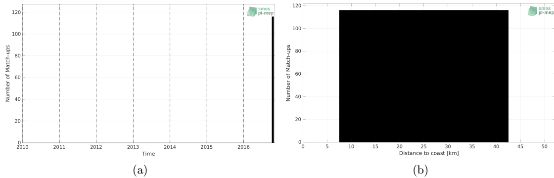
Figure 1: Number of match-ups between TSG (LEGOS-DM) and SMOS SSS L3 v7 - 9 Days (CATDS-CECOS-LOCEAN) SSS as a function of time (a) and as function of the distance to coast (b) over the Gulf of Mexico Pi-MEP region and for the full satellite product period.
