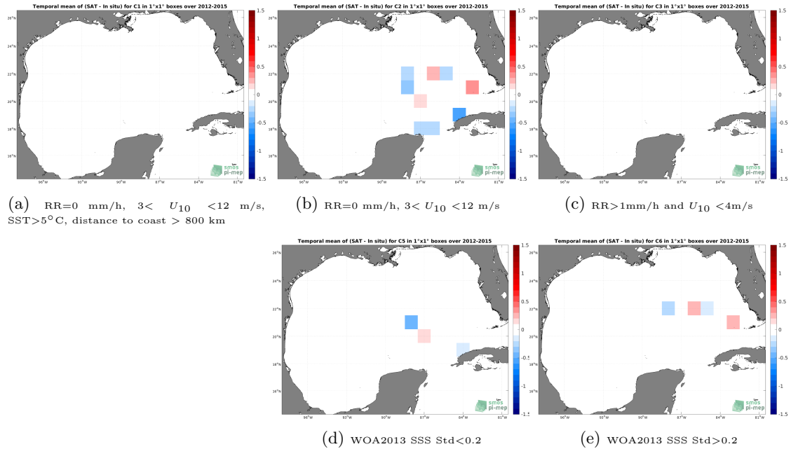
Figure 12: Temporal mean gridded over spatial boxes of size 1^{\circ}\times 1^{\circ} of \Delta SSS (SMOS SSS L3 v7 - 9 Days (CATDS-CECOS-LOCEAN) - TSG (GOSUD-Sailing-ship)) for 5 different subdatasets corresponding to:RR=0 mm/h, 3 < U_{10} < 12 m/s, SST >5^{\circ}\text{C} , distance to coast > 800 km (a), RR=0 mm/h, 3 < U_{10} < 12 m/s (b), RR >1 mm/h and U_{10} < 4 m/s (c), WOA2013 SSS Std <0.2 (d), WOA2013 SSS Std >0.2 (e).
