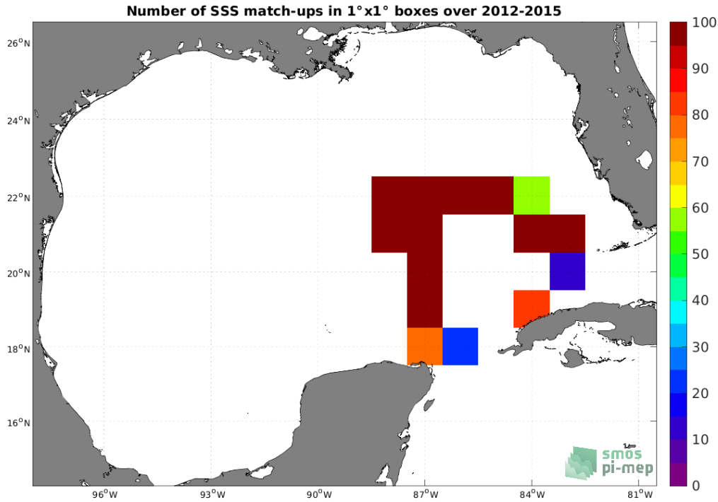
Figure 4: Number of SSS match-ups between TSG (GOSUD-Sailing-ship) SSS and the SMOS SSS L3 v7 - 9 Days (CATDS-CECOS-LOCEAN) SSS product for the Gulf of Mexico Pi-MEP region over 1^\circ \times 1^\circ boxes and for the full satellite product period.
