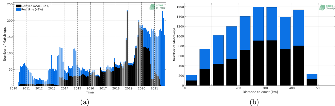
Figure 1: Number of match-ups between Argo and SMOS SSS L3 v7 - 9 Days (CATDS-CECOS-LOCEAN) SSS as a function of time (a) and as function of the distance to coast (b) over the Gulf of Mexico Pi-MEP region and for the full satellite product period.
