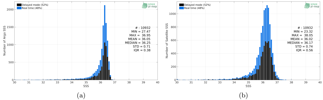
Figure 2: Histograms of SSS from Argo (a) and SMOS SSS L3 v7 - 9 Days (CATDS-CECOS-LOCEAN) (b) considering all match-up pairs per bins of 0.1 over the Gulf of Mexico Pi-MEP region and for the full satellite product period.
