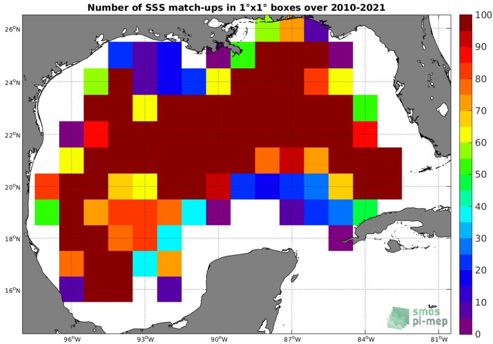
Figure 4: Number of SSS match-ups between Argo SSS and the SMOS SSS L3 v7 - 9 Days (CATDS-CECOS-LOCEAN) SSS product for the Gulf of Mexico Pi-MEP region over 1^\circ \times 1^\circ boxes and for the full satellite product period.
