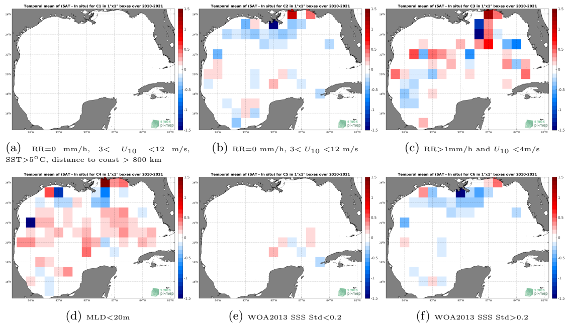
Figure 12: Temporal mean gridded over spatial boxes of size 1^\circ \times 1^\circ of \Delta SSS (SMOS SSS L3 v7 - 9 Days (CATDS-CECOS-LOCEAN) - Argo) for 6 different subdatasets corresponding to:RR=0 mm/h, 3 < U_{10} < 12 m/s, SST >5^\circ C, distance to coast > 800 km (a), RR=0 mm/h, 3 < U_{10} < 12 m/s (b), RR >1 mm/h and U_{10} < 4 m/s (c),MLD <20 m (d),WOA2013 SSS Std <0.2 (e),WOA2013 SSS Std >0.2 (f).
