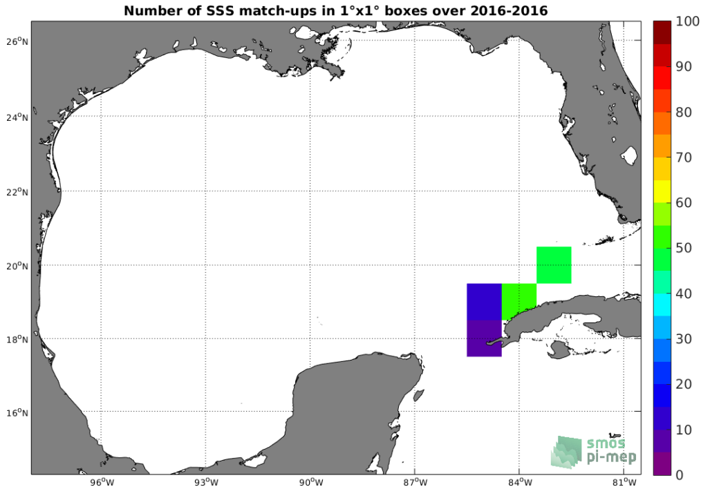
Figure 4: Number of SSS match-ups between TSG (LEGOS-DM) SSS and the SMOS SSS L3 v7 - 18 Days (CATDS-CECOS-LOCEAN) SSS product for the Gulf of Mexico Pi-MEP region over 1^\circ \times 1^\circ boxes and for the full satellite product period.
