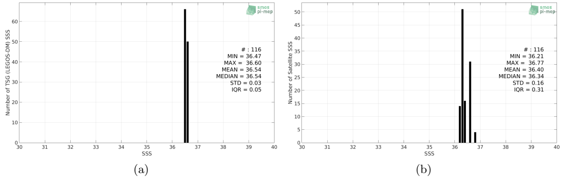
Figure 2: Histograms of SSS from TSG (LEGOS-DM) (a) and SMOS SSS L3 v7 - 18 Days (CATDS-CECOS-LOCEAN) (b) considering all match-up pairs per bins of 0.1 over the Gulf of Mexico Pi-MEP region and for the full satellite product period.
