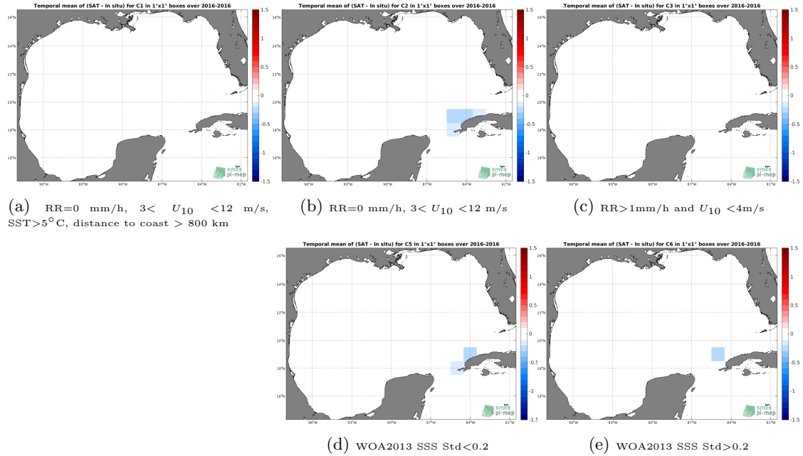
Figure 12: Temporal mean gridded over spatial boxes of size 1^{\circ}\times 1^{\circ} of \Delta\text{SSS} (SMOS SSS L3 v7 - 18 Days (CATDS-CECOS-LOCEAN) - TSG (LEGOS-DM)) for 5 different subdatasets corresponding to:RR=0 mm/h, 3 < U_{10} < 12 m/s, SST >5^{\circ}\text{C} , distance to coast > 800 km (a), RR=0 mm/h, 3 < U_{10} < 12 m/s (b), RR >1 mm/h and U_{10} < 4 m/s (c), WOA2013 SSS Std <0.2 (d), WOA2013 SSS Std >0.2 (e).
