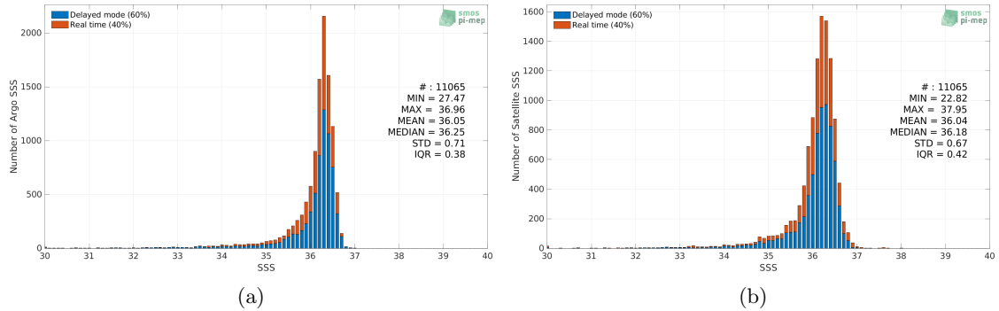
Figure 2: Histograms of SSS from Argo (a) and SMOS SSS L3 v7 - 18 Days (CATDS-CECOS-LOCEAN) (b) considering all match-up pairs per bins of 0.1 over the Gulf of Mexico Pi-MEP region and for the full satellite product period.
