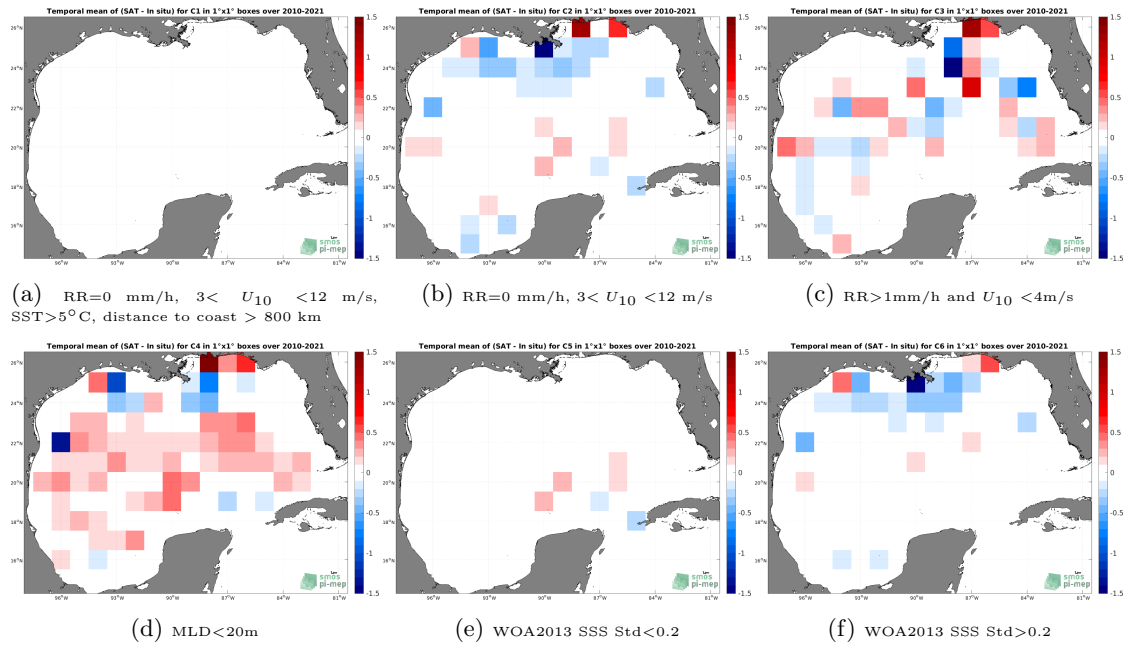
Figure 12: Temporal mean gridded over spatial boxes of size 1^\circ \times 1^\circ of \Delta SSS (SMOS SSS L3 v7 - 18 Days (CATDS-CECOS-LOCEAN) - Argo) for 6 different subdatasets corresponding to:RR=0 mm/h, 3 < U_{10} < 12 m/s, SST > 5^\circ\text{C} , distance to coast > 800 km (a), RR=0 mm/h, 3 < U_{10} < 12 m/s (b), RR > 1 mm/h and U_{10} < 4 m/s (c),MLD < 20 m (d),WOA2013 SSS Std < 0.2 (e),WOA2013 SSS Std > 0.2 (f).
