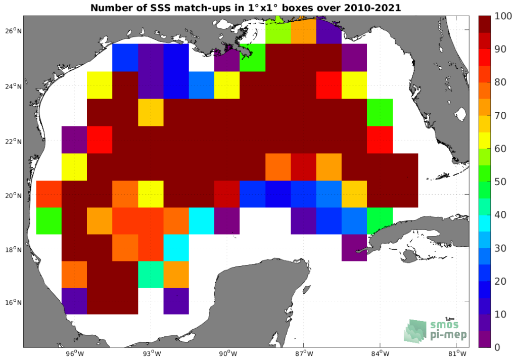
Figure 4: Number of SSS match-ups between Argo SSS and the SMOS SSS L3 v7 - 18 Days (CATDS-CECOS-LOCEAN) SSS product for the Gulf of Mexico Pi-MEP region over 1^\circ \times 1^\circ boxes and for the full satellite product period.
