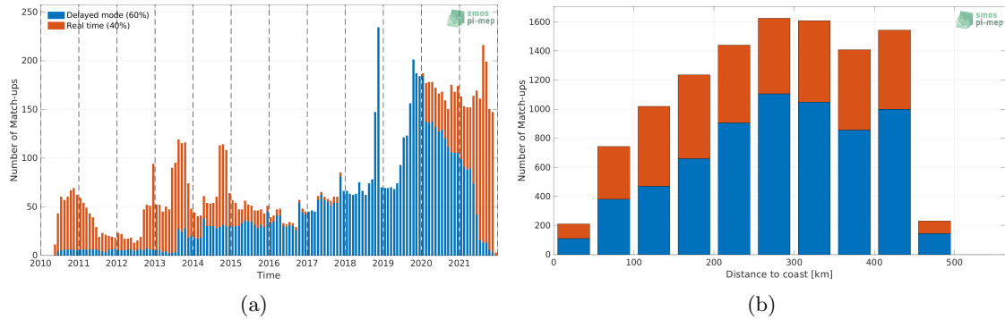
Figure 1: Number of match-ups between Argo and SMOS SSS L3 v7 - 18 Days (CATDS-CECOS-LOCEAN) SSS as a function of time (a) and as function of the distance to coast (b) over the Gulf of Mexico Pi-MEP region and for the full satellite product period.
