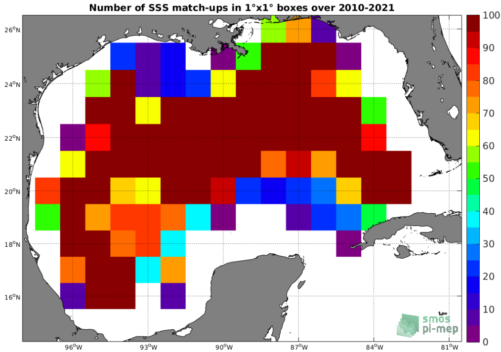
Figure 4: Number of SSS match-ups between Argo SSS and the SMOS SSS L3 v7 - 18 Days (CATDS-CECOS-LOCEAN) SSS product for the Gulf of Mexico Pi-MEP region over 1^{\circ} \times 1^{\circ} boxes and for the full satellite product period.
