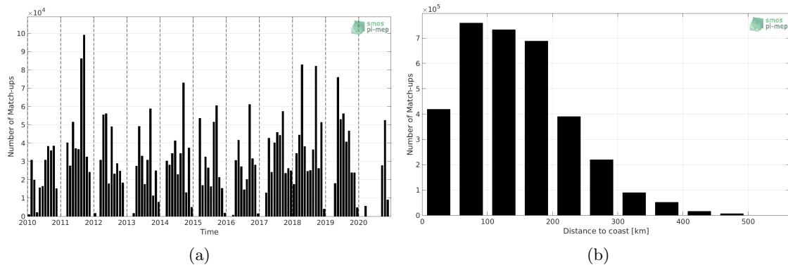
Figure 1: Number of match-ups between TSG (SAMOS) and SMOS SSS L3 v5 - 9 Days (CATDS-CECOS-LOCEAN) SSS as a function of time (a) and as function of the distance to coast (b) over the Gulf of Mexico Pi-MEP region and for the full satellite product period.
