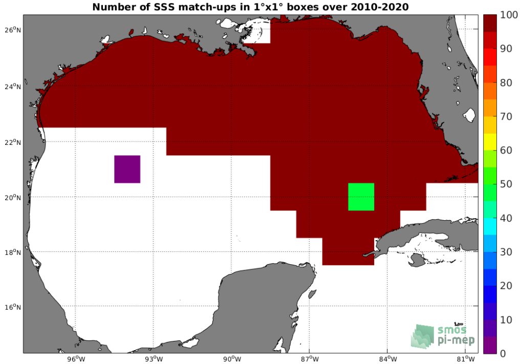
Figure 4: Number of SSS match-ups between TSG (SAMOS) SSS and the SMOS SSS L3 v5 - 9 Days (CATDS-CECOS-LOCEAN) SSS product for the Gulf of Mexico Pi-MEP region over 1^\circ \times 1^\circ boxes and for the full satellite product period.
