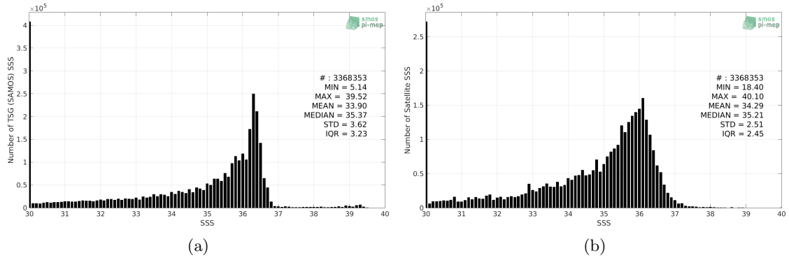
Figure 2: Histograms of SSS from TSG (SAMOS) (a) and SMOS SSS L3 v5 - 9 Days (CATDS-CECOS-LOCEAN) (b) considering all match-up pairs per bins of 0.1 over the Gulf of Mexico Pi-MEP region and for the full satellite product period.
