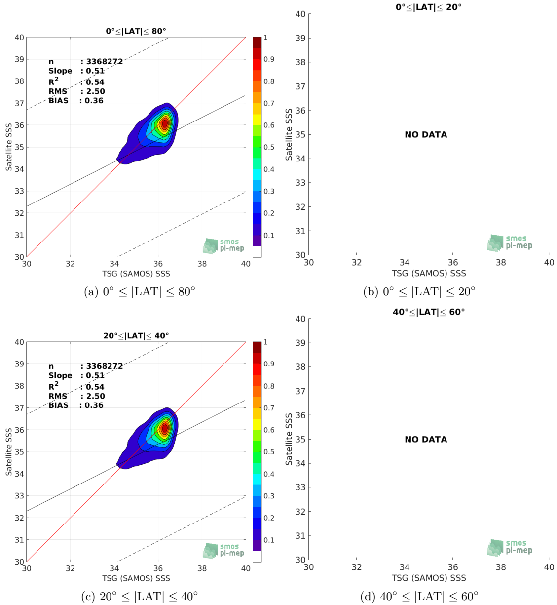
Figure 9: Contour maps of the concentration of SMOS SSS L3 v5 - 9 Days (CATDS-CECOS-LOCEAN) SSS (y-axis) versus TSG (SAMOS) SSS (x-axis) at match-up pairs for different latitude bands. For each plot, the red line shows x=y . The black thin and dashed lines indicate a linear fit through the data cloud and the \pm 95\% confidence levels, respectively. The number match-up pairs n , the slope and R^2 coefficient of the linear fit, the root mean square (RMS) and the mean bias between satellite and in situ data are indicated for each latitude band in each plots.
