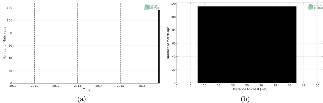
Figure 1: Number of match-ups between TSG (LEGOS-DM) and SMOS SSS L3 v5 - 9 Days (CATDS-CECOS-LOCEAN) SSS as a function of time (a) and as function of the distance to coast (b) over the Gulf of Mexico Pi-MEP region and for the full satellite product period.
