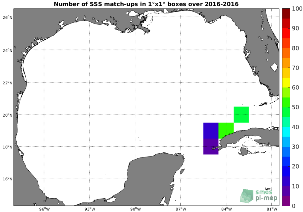
Figure 4: Number of SSS match-ups between TSG (LEGOS-DM) SSS and the SMOS SSS L3 v5 - 9 Days (CATDS-CECOS-LOCEAN) SSS product for the Gulf of Mexico Pi-MEP region over 1°×1° boxes and for the full satellite product period.
