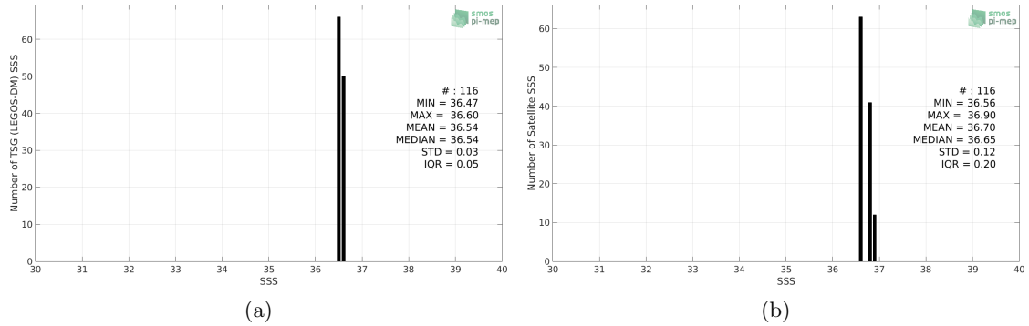
Figure 2: Histograms of SSS from TSG (LEGOS-DM) (a) and SMOS SSS L3 v5 - 9 Days (CATDS-CECOS-LOCEAN) (b) considering all match-up pairs per bins of 0.1 over the Gulf of Mexico Pi-MEP region and for the full satellite product period.
