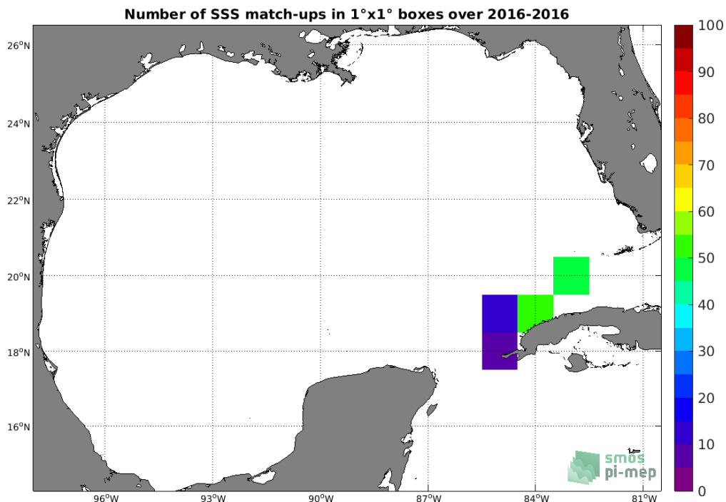
Figure 4: Number of SSS match-ups between TSG (LEGOS-DM) SSS and the SMOS SSS L3 v5 - 9 Days (CATDS-CECOS-LOCEAN) SSS product for the Gulf of Mexico Pi-MEP region over 1^\circ \times 1^\circ boxes and for the full satellite product period.
