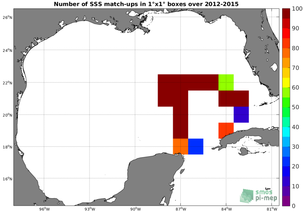
Figure 4: Number of SSS match-ups between TSG (GOSUD-Sailing-ship) SSS and the SMOS SSS L3 v5 - 9 Days (CATDS-CECOS-LOCEAN) SSS product for the Gulf of Mexico Pi-MEP region over 1^\circ \times 1^\circ boxes and for the full satellite product period.
