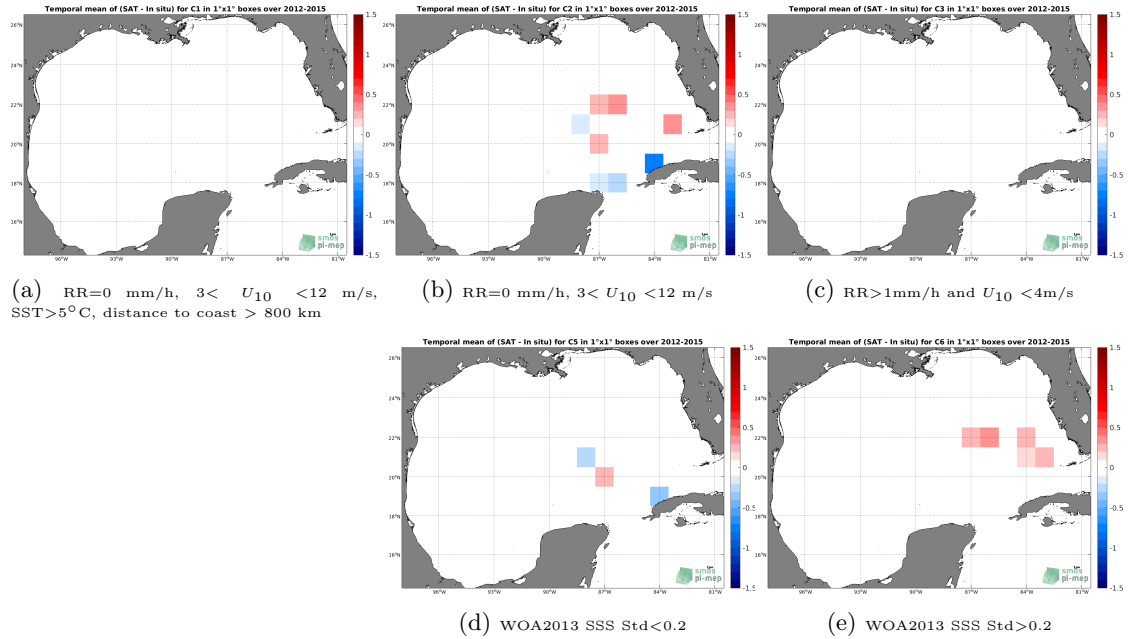
Figure 12: Temporal mean gridded over spatial boxes of size 1^{\circ}\times 1^{\circ} of \Delta SSS (SMOS SSS L3 v5 - 9 Days (CATDS-CECOS-LOCEAN) - TSG (GOSUD-Sailing-ship)) for 5 different subdatasets corresponding to:RR=0 mm/h, 3 < U_{10} < 12 m/s, SST >5^{\circ}\text{C} , distance to coast > 800 km (a), RR=0 mm/h, 3 < U_{10} < 12 m/s (b), RR >1 mm/h and U_{10} < 4 m/s (c), WOA2013 SSS Std <0.2 (d), WOA2013 SSS Std >0.2 (e).
