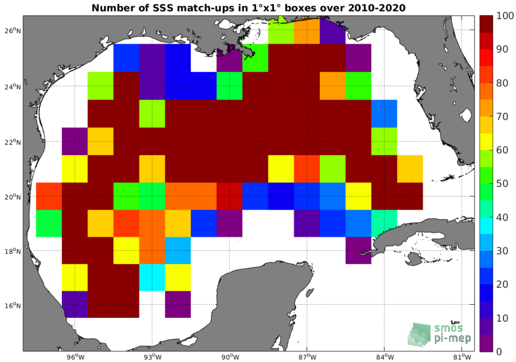
Figure 4: Number of SSS match-ups between Argo SSS and the SMOS SSS L3 v5 - 9 Days (CATDS-CECOS-LOCEAN) SSS product for the Gulf of Mexico Pi-MEP region over 1^\circ \times 1^\circ boxes and for the full satellite product period.
