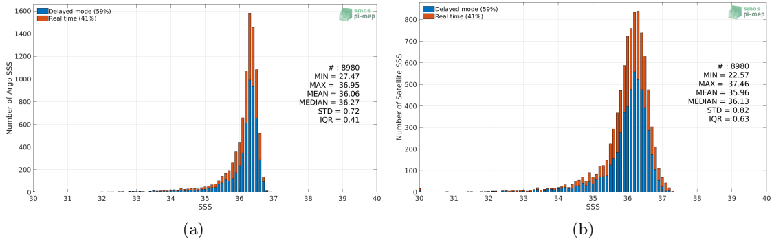
Figure 2: Histograms of SSS from Argo (a) and SMOS SSS L3 v5 - 9 Days (CATDS-CECOS-LOCEAN) (b) considering all match-up pairs per bins of 0.1 over the Gulf of Mexico Pi-MEP region and for the full satellite product period.
