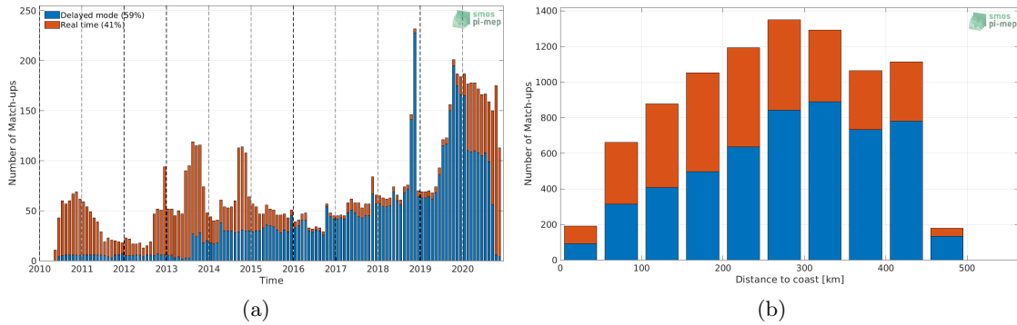
Figure 1: Number of match-ups between Argo and SMOS SSS L3 v5 - 9 Days (CATDS-CECOS-LOCEAN) SSS as a function of time (a) and as function of the distance to coast (b) over the Gulf of Mexico Pi-MEP region and for the full satellite product period.
