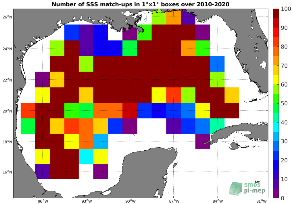
Figure 4: Number of SSS match-ups between Argo SSS and the SMOS SSS L3 v5 - 9 Days (CATDS-CECOS-LOCEAN) SSS product for the Gulf of Mexico Pi-MEP region over 1°x1° boxes and for the full satellite product period.
