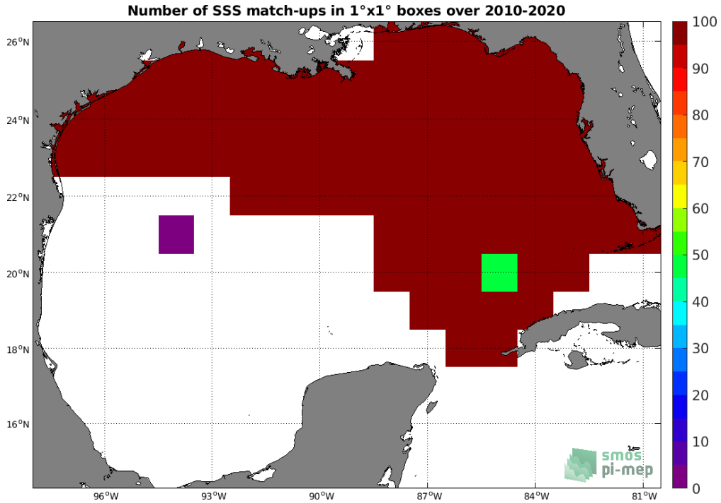
Figure 4: Number of SSS match-ups between TSG (SAMOS) SSS and the SMOS SSS L3 v5 - 18 Days (CATDS-CECOS-LOCEAN) SSS product for the Gulf of Mexico Pi-MEP region over 1^\circ \times 1^\circ boxes and for the full satellite product period.
