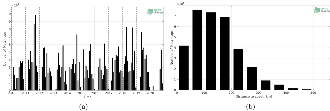
Figure 1: Number of match-ups between TSG (SAMOS) and SMOS SSS L3 v5 - 18 Days (CATDS-CECOS-LOCEAN) SSS as a function of time (a) and as function of the distance to coast (b) over the Gulf of Mexico Pi-MEP region and for the full satellite product period.
