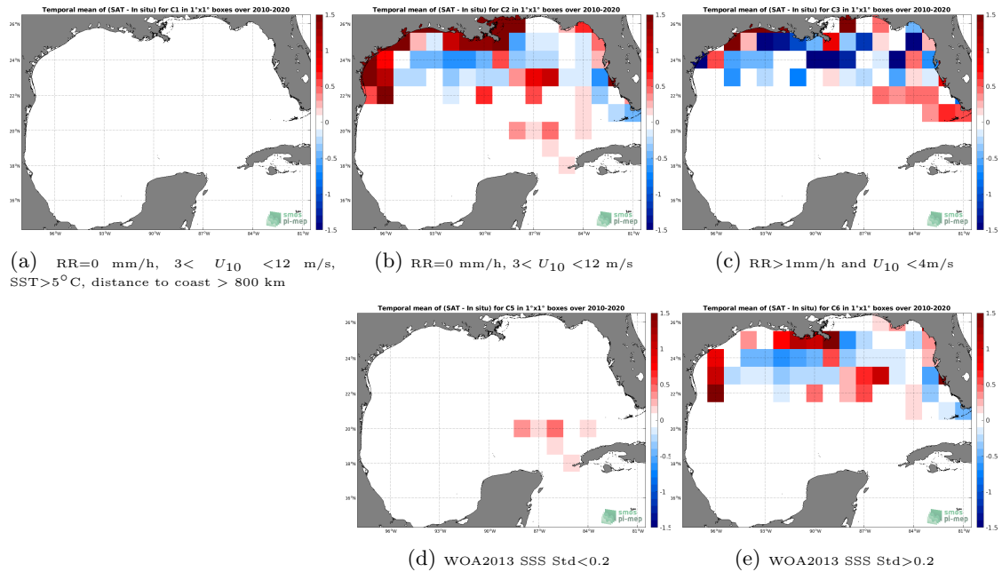
Figure 12: Temporal mean gridded over spatial boxes of size 1^{\circ}\times 1^{\circ} of \Delta\text{SSS} (SMOS SSS L3 v5 - 18 Days (CATDS-CECOS-LOCEAN) - TSG (SAMOS)) for 5 different subdatasets corresponding to:RR=0 mm/h, 3 < U_{10} < 12 m/s, SST >5^{\circ}\text{C} , distance to coast > 800 km (a), RR=0 mm/h, 3 < U_{10} < 12 m/s (b), RR >1 mm/h and U_{10} < 4 m/s (c), WOA2013 SSS Std <0.2 (d), WOA2013 SSS Std >0.2 (e).
