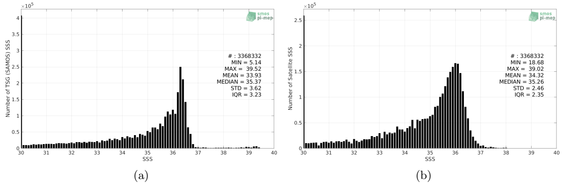
Figure 2: Histograms of SSS from TSG (SAMOS) (a) and SMOS SSS L3 v5 - 18 Days (CATDS-CECOS-LOCEAN) (b) considering all match-up pairs per bins of 0.1 over the Gulf of Mexico Pi-MEP region and for the full satellite product period.
