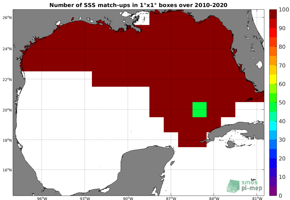
Figure 4: Number of SSS match-ups between TSG (SAMOS) SSS and the SMOS SSS L3 v5 - 18 Days (CATDS-CECOS-LOCEAN) SSS product for the Gulf of Mexico Pi-MEP region over 1°x1° boxes and for the full satellite product period.
