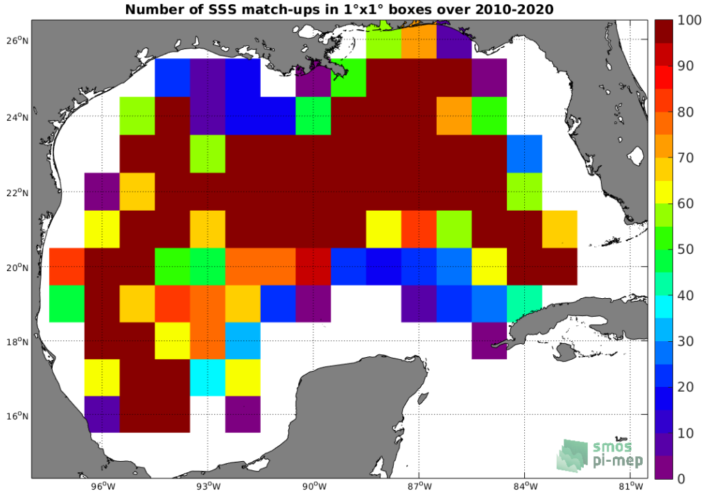
Figure 4: Number of SSS match-ups between Argo SSS and the SMOS SSS L3 v5 - 18 Days (CATDS-CECOS-LOCEAN) SSS product for the Gulf of Mexico Pi-MEP region over 1^\circ \times 1^\circ boxes and for the full satellite product period.
