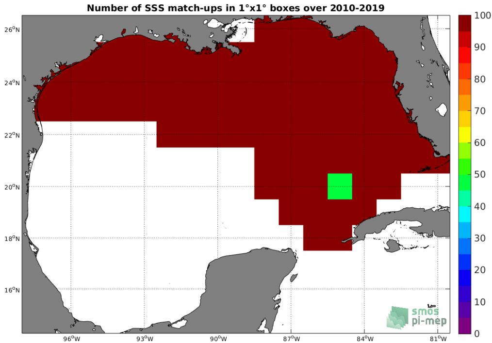
Figure 4: Number of SSS match-ups between TSG (SAMOS) SSS and the SMOS SSS L3 v4 - 9 Days (CATDS-CECOS-LOCEAN) SSS product for the Gulf of Mexico Pi-MEP region over 1°x1° boxes and for the full satellite product period.
