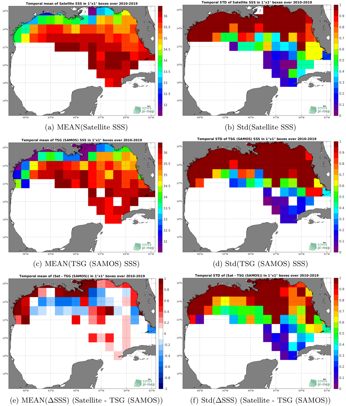
Figure 6: Temporal mean (left) and Std (right) of SSS from SMOS SSS L3 v4 - 9 Days (CATDS-CECOS-LOCEAN) (top), TSG (SAMOS) (middle), and of \Delta SSS (Satellite - TSG (SAMOS)). Only match-up pairs are used to generate these maps.
