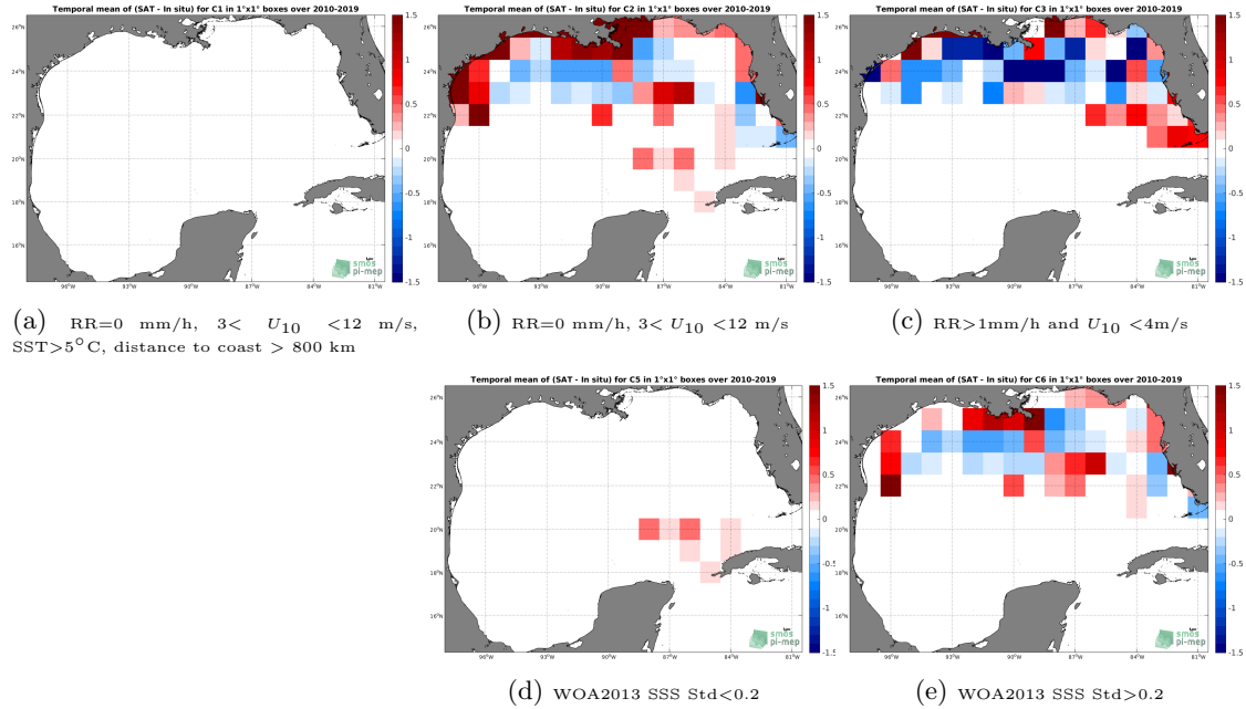
Figure 12: Temporal mean gridded over spatial boxes of size 1^{\circ}\times 1^{\circ} of \Delta\text{SSS} (SMOS SSS L3 v4 - 9 Days (CATDS-CECOS-LOCEAN) - TSG (SAMOS)) for 5 different subdatasets corresponding to:RR=0 mm/h, 3 < U_{10} < 12 m/s, SST >5^{\circ}\text{C} , distance to coast > 800 km (a), RR=0 mm/h, 3 < U_{10} < 12 m/s (b), RR >1 mm/h and U_{10} < 4 m/s (c), WOA2013 SSS Std <0.2 (d), WOA2013 SSS Std >0.2 (e).
