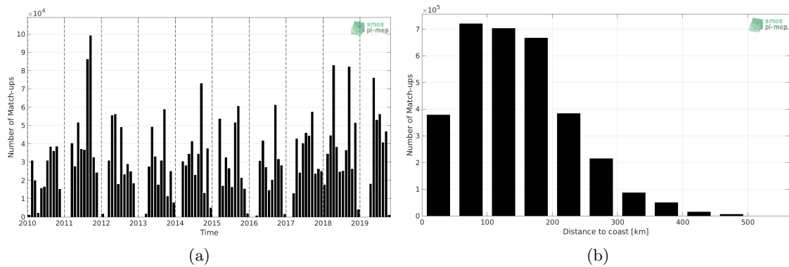
Figure 1: Number of match-ups between TSG-SAMOS and SMOS-L3-CATDS-CECOS-LOCEAN-V4-9DAYS-25KM SSS as a function of time (a) and as function of the distance to coast (b) over the Gulf of Mexico Pi-MEP region and for the full satellite product period.
