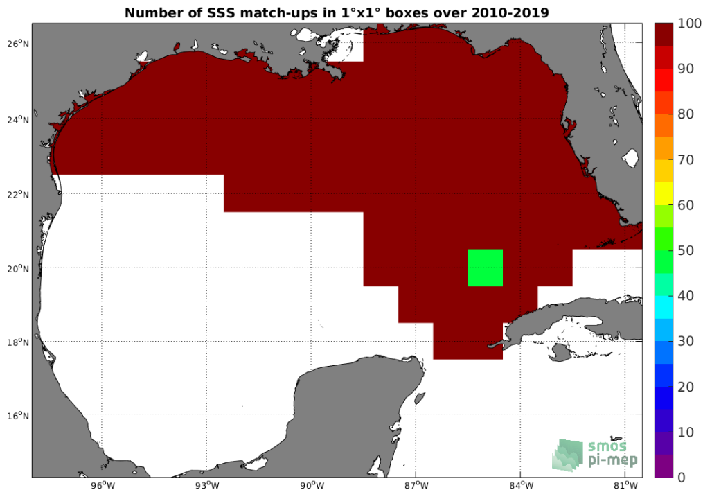
Figure 4: Number of SSS match-ups between TSG-SAMOS SSS and the SMOS-L3-CATDS-CECOS-LOCEAN-V4-9DAYS-25KM SSS product for the Gulf of Mexico Pi-MEP region over 1^\circ \times 1^\circ boxes and for the full satellite product period.
