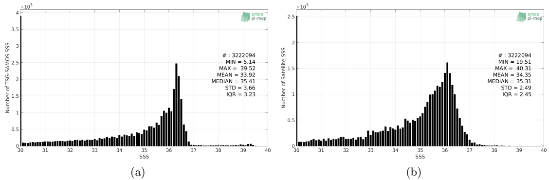
Figure 2: Histograms of SSS from TSG-SAMOS (a) and SMOS-L3-CATDS-CECOS-LOCEAN-V4-9DAYS-25KM (b) considering all match-up pairs per bins of 0.1 over the Gulf of Mexico Pi-MEP region and for the full satellite product period.
