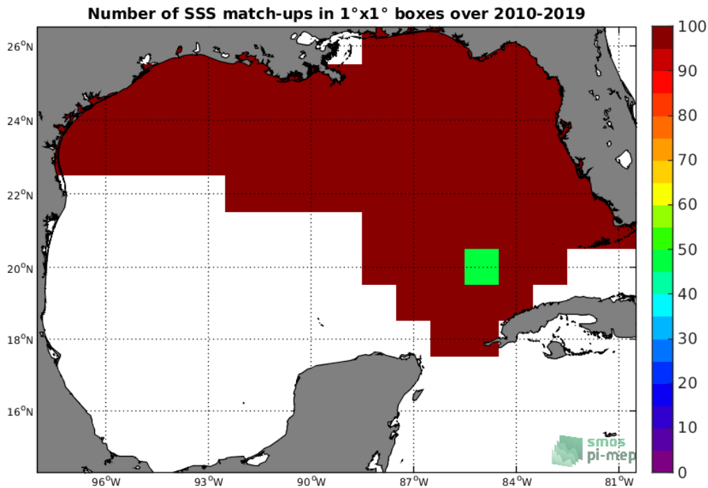
Figure 4: Number of SSS match-ups between TSG-SAMOS SSS and the SMOS-L3-CATDS-CECOS-LOCEAN-V4-9DAYS-25KM SSS product for the Gulf of Mexico Pi-MEP region over 1°x1° boxes and for the full satellite product period.
