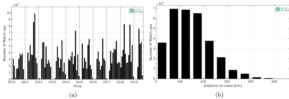
Figure 1: Number of match-ups between TSG-SAMOS and SMOS-L3-CATDS-CECOS-LOCEAN-V4-9DAYS-25KM SSS as a function of time (a) and as function of the distance to coast (b) over the Gulf of Mexico Pi-MEP region and for the full satellite product period.
