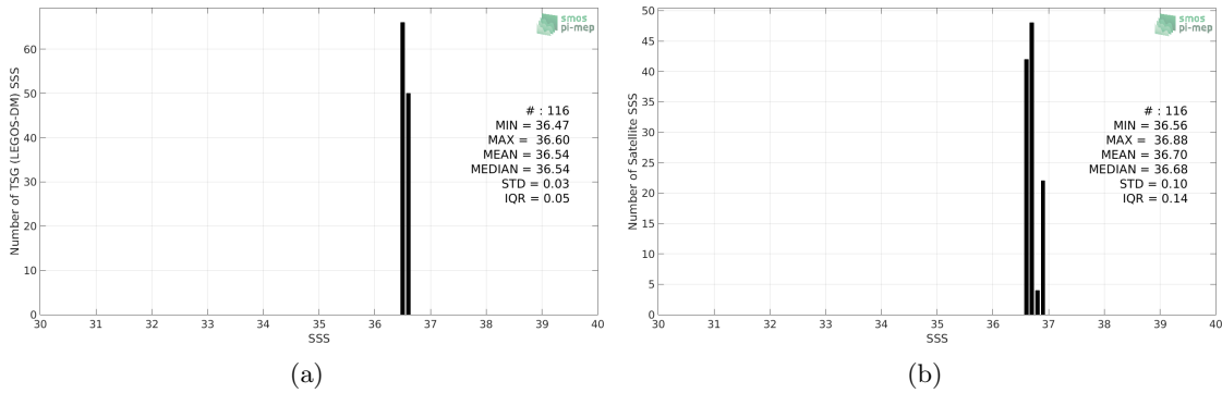
Figure 2: Histograms of SSS from TSG (LEGOS-DM) (a) and SMOS SSS L3 v4 - 9 Days (CATDS-CECOS-LOCEAN) (b) considering all match-up pairs per bins of 0.1 over the Gulf of Mexico Pi-MEP region and for the full satellite product period.
