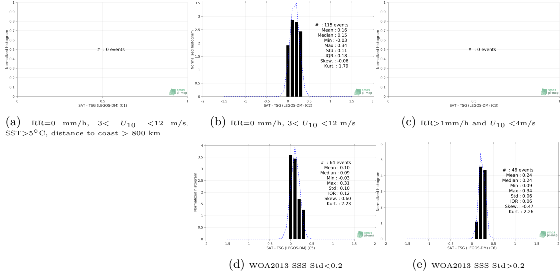
Figure 13: Normalized histogram of \Delta\text{SSS} (SMOS SSS L3 v4 - 9 Days (CATDS-CECOS-LOCEAN) - TSG (LEGOS-DM)) for 5 different subdatasets corresponding to: RR=0 mm/h, 3 < U_{10} < 12 m/s, SST > 5^{\circ}\text{C} , distance to coast > 800 km (a), RR=0 mm/h, 3 < U_{10} < 12 m/s (b), RR > 1\text{mm/h} and U_{10} < 4\text{m/s} (c), WOA2013 SSS Std < 0.2 (d), WOA2013 SSS Std > 0.2 (e).
