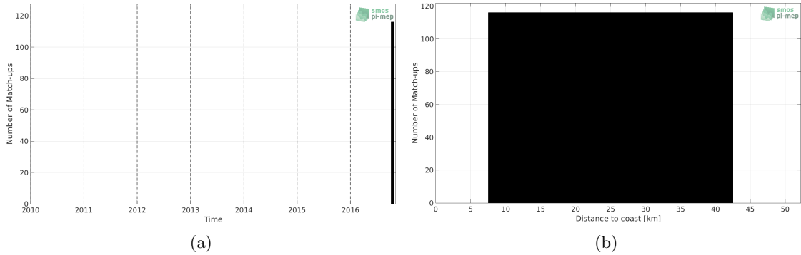
Figure 1: Number of match-ups between TSG (LEGOS-DM) and SMOS SSS L3 v4 - 9 Days (CATDS-CECOS-LOCEAN) SSS as a function of time (a) and as function of the distance to coast (b) over the Gulf of Mexico Pi-MEP region and for the full satellite product period.
