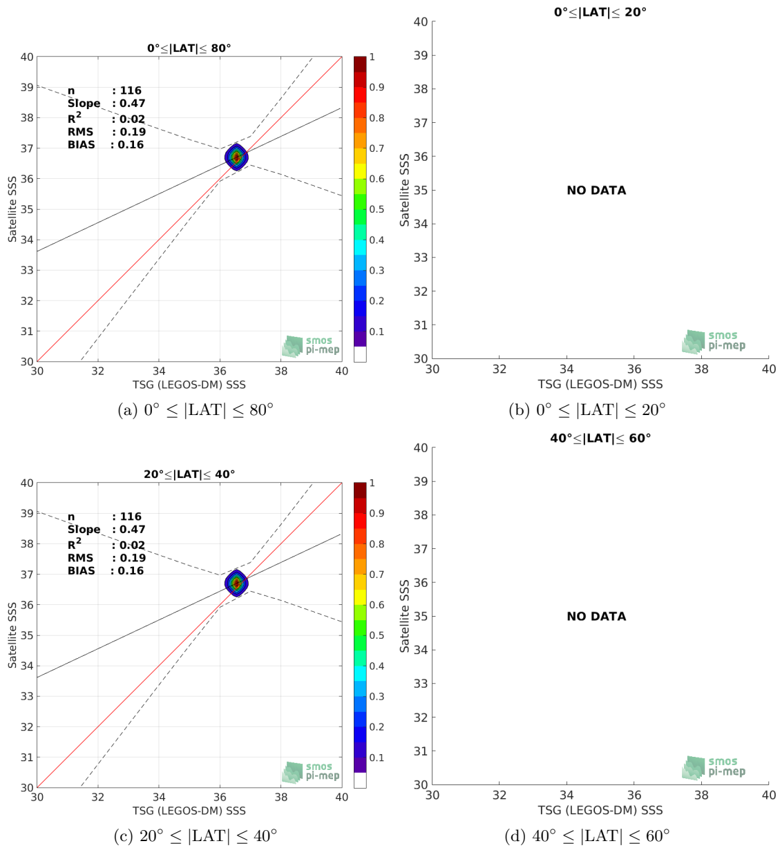
Figure 9: Contour maps of the concentration of SMOS SSS L3 v4 - 9 Days (CATDS-CECOS-LOCEAN) SSS (y-axis) versus TSG (LEGOS-DM) SSS (x-axis) at match-up pairs for different latitude bands. For each plot, the red line shows x=y . The black thin and dashed lines indicate a linear fit through the data cloud and the \pm 95\% confidence levels, respectively. The number match-up pairs n , the slope and R^2 coefficient of the linear fit, the root mean square (RMS) and the mean bias between satellite and in situ data are indicated for each latitude band in each plots.
