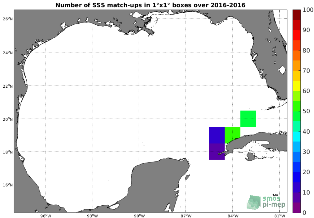
Figure 4: Number of SSS match-ups between TSG (LEGOS-DM) SSS and the SMOS SSS L3 v4 - 9 Days (CATDS-CECOS-LOCEAN) SSS product for the Gulf of Mexico Pi-MEP region over 1^\circ \times 1^\circ boxes and for the full satellite product period.
