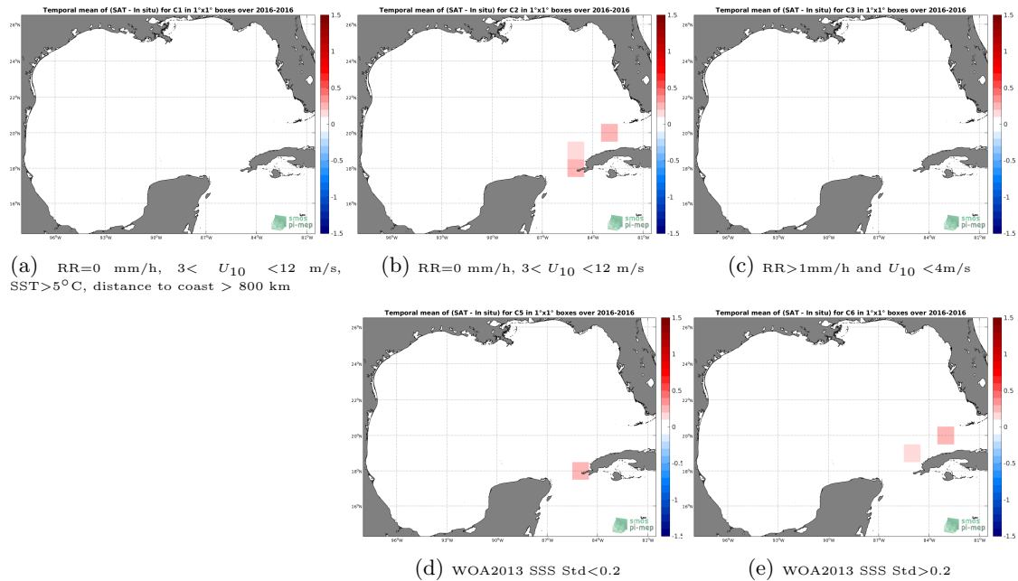
Figure 12: Temporal mean gridded over spatial boxes of size 1^{\circ}\times 1^{\circ} of \Delta\text{SSS} (SMOS-L3-CATDS-CECOS-LOCEAN-V4-9DAYS-25KM - TSG-LEGOS-DM) for 5 different subdatasets corresponding to:RR=0 mm/h, 3 < U_{10} < 12 m/s, SST >5^{\circ}\text{C} , distance to coast > 800 km (a), RR=0 mm/h, 3 < U_{10} < 12 m/s (b), RR >1 mm/h and U_{10} < 4 m/s (c), WOA2013 SSS Std <0.2 (d), WOA2013 SSS Std >0.2 (e).
